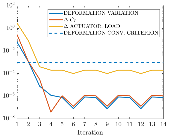
Figure 6. Convergence assessment of the FSI framework for actuator loads and \delta C_L for Bend down morphing condition. Reproduced with permission from [31].
