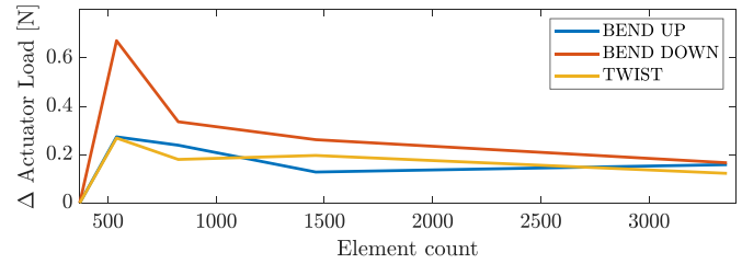
Figure 21. Structural mesh convergence study [31].
