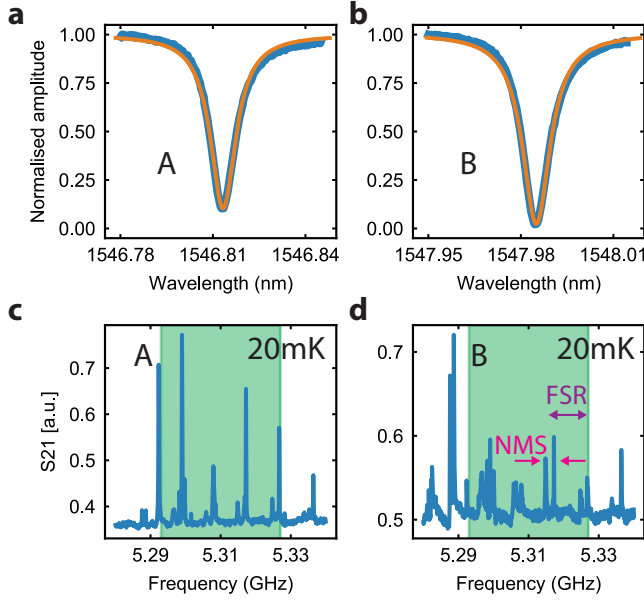
Figure 4.2: a,b) Optical response of device A (left) and B (right). The devices have optical resonances in the C-band at telecom wavelengths. c,d) Mechanical spectrum of device A (left) and B (right) measured using OMIT. We observe a series of Fabry-Pérot modes spaced by \Delta\nu_{\text{FRS}} and split by the normal-mode splitting \Delta\nu_{\text{NMS}} due to the directional coupler. The green shaded area indicates the spectral region used to investigate the dynamics of phononic wavepackets (see text for more details).
