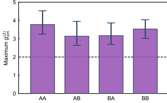
Figure 4.4: The second order cross-correlation g_{om}^{(2)} between the Stokes and anti-Stokes scattered photons from the write and read pulses – we measure g_{om,AA}^{(2)} = 3.8^{+0.8}_{-0.5} , g_{om,AB}^{(2)} = 3.1^{+0.8}_{-0.5} , g_{om,BA}^{(2)} = 3.2^{+0.7}_{-0.5} and g_{om,BB}^{(2)} = 3.5^{+0.5}_{-0.5} – all values are above the classical threshold of 2 (dashed line) by more than two standard deviations. Error bars indicate one standard deviation.
