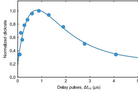
Figure 3.6: Normalized clickrates from the probe pulse that gives an uncalibrated measure of the thermal population in time. The delay between pump and probe pulse is \Delta t_{r0} . We extract T_1 \approx 2.2\mu\text{s} , by fitting the data (solid curve).
