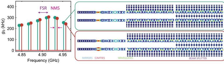
Figure 4.5: Simulation of the whole structure for a device with 50 unit cell of directional coupler and about 80\text{ }\mu\text{m} total length (shorter than the measured device in the main text, for a faster simulation time). Left: calculated single photon optomechanical coupling rate for symmetric (green) and anti-symmetric (red) modes - for each Fabry-Pérot mode, the symmetric and anti-symmetric modes form a doublet split by \Delta\nu_{\text{NMS}} due to the phononic coupling between the top and bottom waveguides. Right: mechanical mode profiles corresponding to one of the doublets. The whole structure is reported in segments for space reason.
