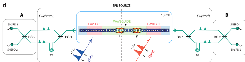
Figure 3.13: Different version of Fig. 3.1d. The vertical dashed line represent a "mirroring" of the device and setup. despite being less accurate and intuitive, it gives a very clear and immediate idea of the EPR pair (Stokes scattered photons and the phonons that traveled in the waveguide once converted in anti-Stokes scattered photons) and of the station A and B.
