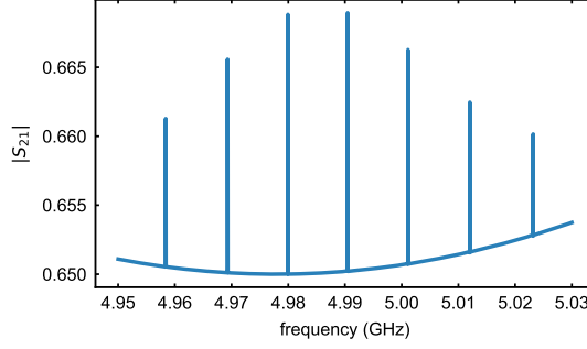
Figure 2.12: Numerically calculated S_{21} signal, using the parameters given in the main text.
