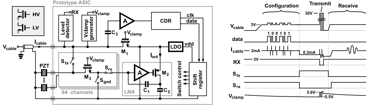
Fig. 2. Block diagram of the prototype ASIC and corresponding waveforms.
