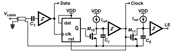
Fig. 7. Block diagram of data recovery circuit.
