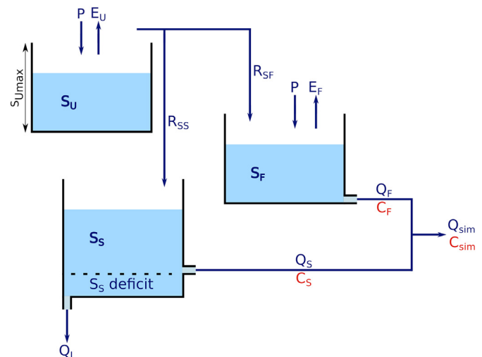
Fig. 2. Conceptual diagram of the hydro-chemical model. P is precipitation, E_i , S_i and Q_i are the i th reservoir's evaporative fluxes, water storage and contributions to the modeled discharge Q_{sim} , respectively. S_{Umax} is the storage capacity of the unsaturated reservoir, and R_{SS} and R_{SF} are water flows from S_U to S_S and S_F , respectively. Q_S and Q_F are the slow and fast contributions to stream flow, respectively. Q_L are deep losses. C_S , C_F and C_{sim} are the solute concentrations of Q_S , Q_F and Q_{sim} , respectively.
