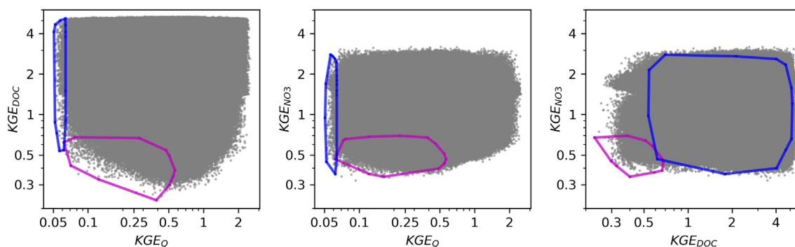
Fig. 4. Log-scaled dot-plots of KGE_x scores for discharge (Q), dissolved organic carbon (DOC) and nitrate ( \text{NO}_3^- ) after 10^7 simulations. The circled areas include the 1000 best simulations (i.e. with the lowest KGE_x scores) based on discharge-only ( KGE_Q , blue) or overall ( KGE_{\text{global}} , purple) performance metrics. (For interpretation of the references to color in this figure legend, the reader is referred to the web version of this article.)
