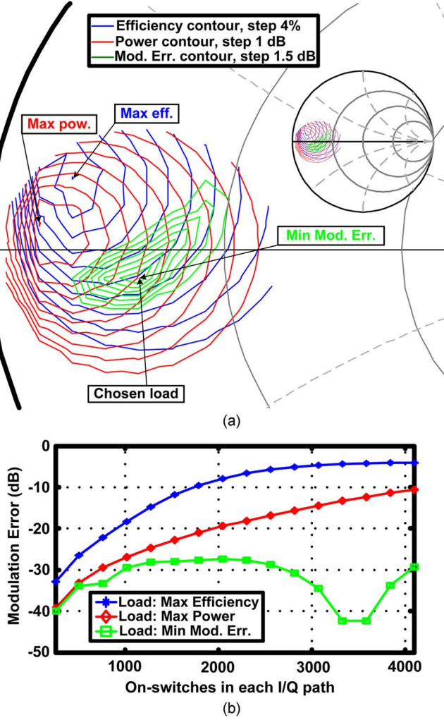
Fig. 6. (a) Load-pull simulations for Drain + node. (b) Modulation error of different load types (max efficiency, max power, and min modulation error) versus count of on-switches in each orthogonal path.
