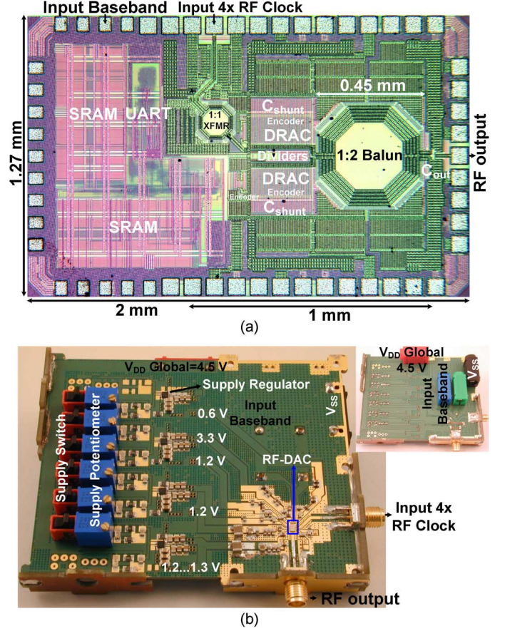
Fig. 19. (a) Micrograph of the 2 \times 13 -bit all-digital I/Q RF-DAC TX. (b) Front and back view of its related PCB.
