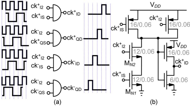
Fig. 11. (a) 25% duty cycle generator schematic from [11]. (b) Its AND logic circuit.
