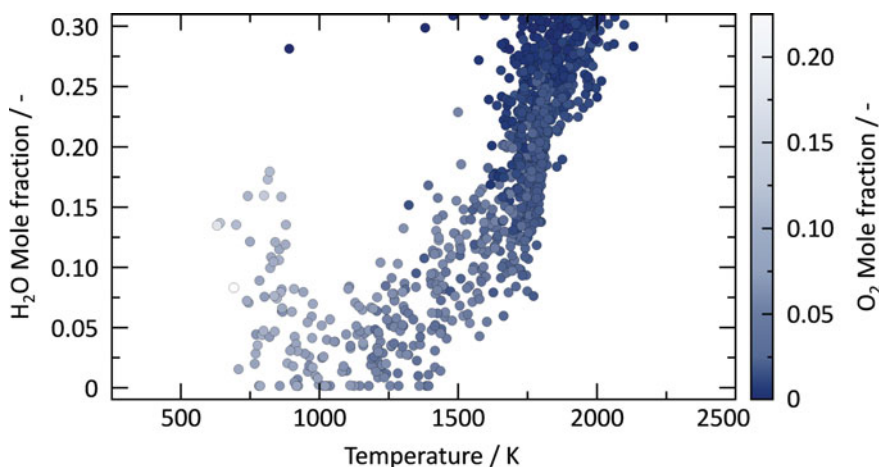
Fig. 13.16 Complete scalar characterization in a turbulent hydrogen jet flame. Each point in the scatter plot represents the local temperature and absolute \text{O}_2 and \text{H}_2\text{O} mole fractions measured 6.75 mm from the centerline of the turbulent jet flame. 300 single-shot fs/ps CARS spectra are acquired in the sample. As expected, strong positive and negative correlations are found between temperature and \text{H}_2\text{O} and \text{O}_2 mole fractions, respectively. Adapted with permission from Castellanos et al. [72]. © 2022 Elsevier Inc.
