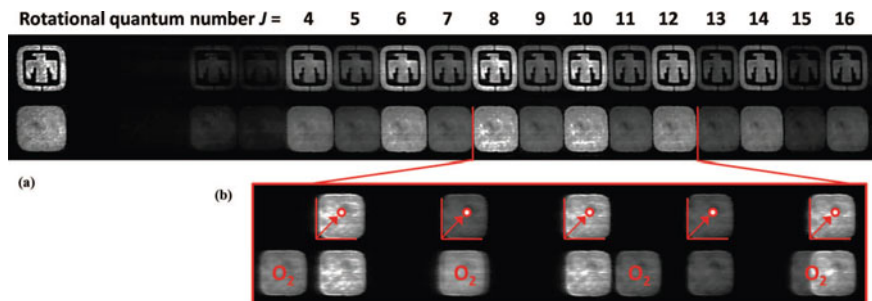
Fig. 13.4 Two-beam fs/ps planar CARS imaging (2D-CARS). a Single-shot hyperspectral \text{N}_2 CARS image recorded at room temperature. In the first row, a mask is placed on the probe beam path to illustrate the imaging quality of the CARS instrument. b High-spectral resolution 2D CARS images acquired in \text{N}_2 (first row) and \text{O}_2 (second row), each square image corresponding to an isolated line in the pure-rotational Raman spectrum. Each image consists of \sim 125 \times 120 pixels, corresponding to \sim 15000 spatially correlated spectra recorded with a single-shot. Adapted with permission from Bohlin and Kliewer [37]. © 2013 AIP Publishing LLC
