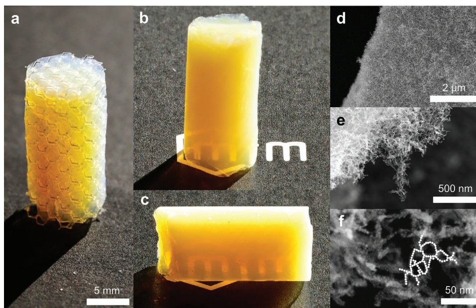
Figure 2. Photographs of translucent cm-sized aerogel monoliths a) with and b,c) without an embedded standard scaffold and d–f) SEM images of the \text{TiO}_2 -Pd aerogel morphology at different magnifications. The pearl-necklace-like structure of the nanoparticle network is highlighted with white filled circles in (f).
