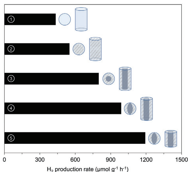
Figure 9. Hydrogen production rate in μmol g -1 h -1 after 10 h of illumination time of TiO 2 -Pd aerogels synthesized around various scaffold geometries: no scaffold (1), standard scaffold (2), scaffold with solid core with circular cross-section (3), scaffold with solid core with elliptical cross-section (4), scaffold with solid core with elliptical cross-section and optimized length of 1.5 cm (5).
