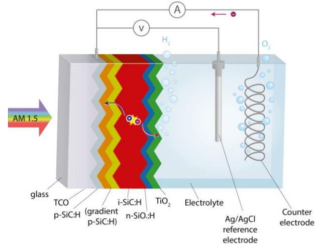
Figure 1. Schematic representation of the 3-electrode photocathode configuration
