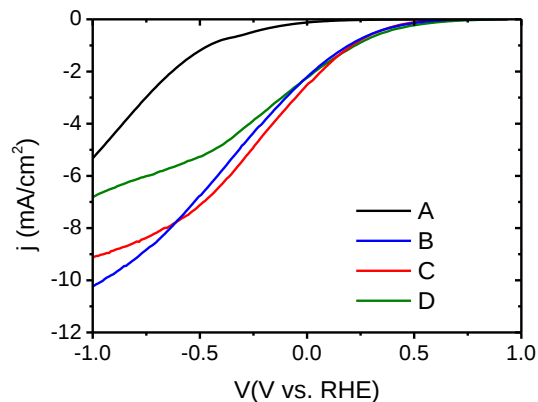
Fig. 3. Schematic illustration and PEC results of the p-i a-SiC:H photocathode (A) p-i-n photocathode (B), p-grad. p-i photocathode (C) and p-grad. p-i-n photocathode (D).
