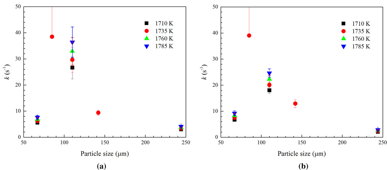
Fig. 6—Effect of particle size on the reaction rate constant in (a) PCR4' and (b) PCR2' atmospheres.
