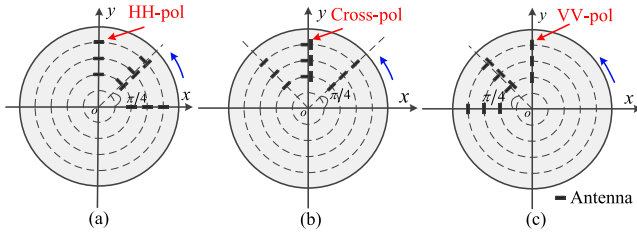
Fig. 1. Operating scheme of a rotated antenna array for full-polarimetric imaging. (a)–(c) Three instantaneous positions of the rotated antenna array during the operation.
