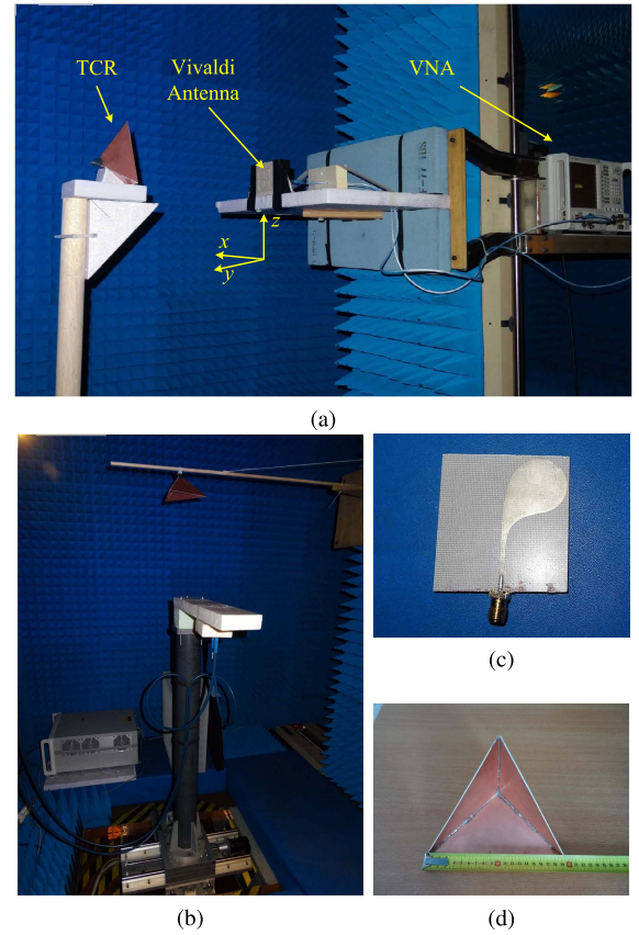
Fig. 4. Experimental setups for rotated arrays and traditional full-pol antenna arrays. (a) Setup for traditional polarimetric arrays. (b) Measurement setup for rotated antenna arrays. (c) Antipodal Vivaldi antenna used for measurement. (d) TCR.
