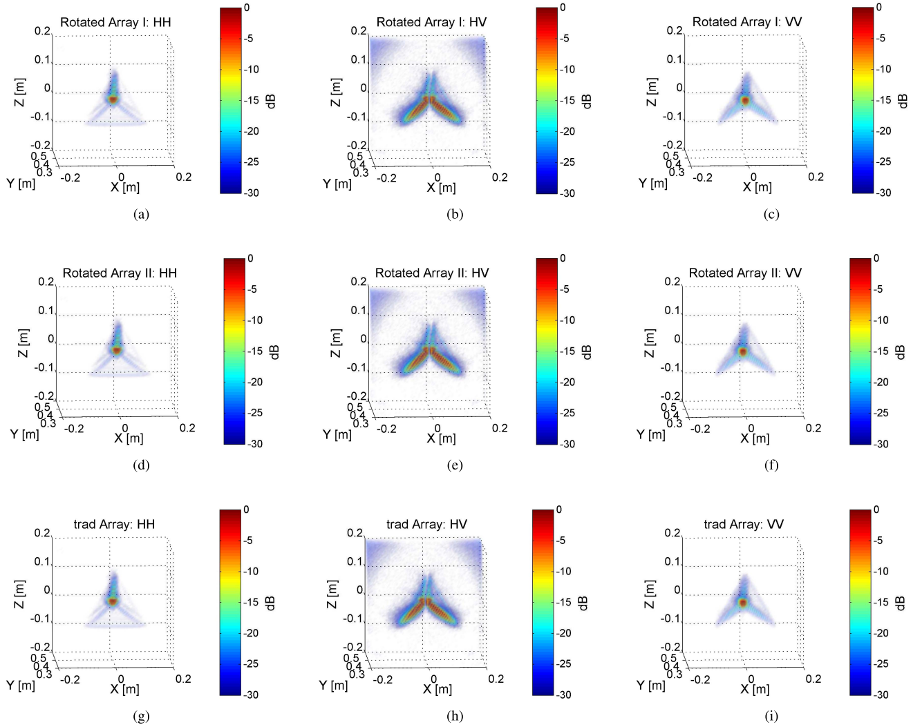
Fig. 3. HH-, HV-, and VV-pol images reconstructed with the three different antenna arrays. (a)–(c) Images obtained with the rotated antenna array by acquiring two co-pol and one cross-pol signals at each position (array I). (d)–(f) Images obtained with the rotated antenna array by acquiring three co-pol signals at each position (array II). (g)–(i) Images obtained with traditional antenna arrays (array III).
