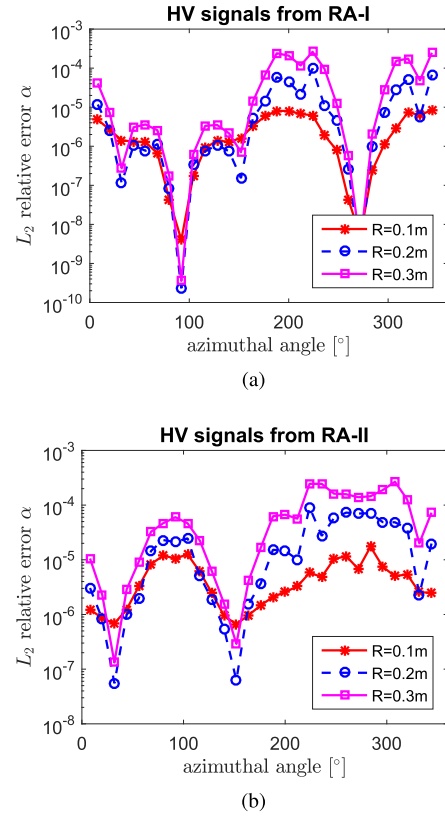
Fig. 2. L_2 relative errors of the retrieved cross-pol signals at some sampling positions over three circles of radii 0.1, 0.2, and 0.3 m within the aperture. (a) and (b) Relative errors of HV signals obtained with rotated arrays I and II, respectively.
