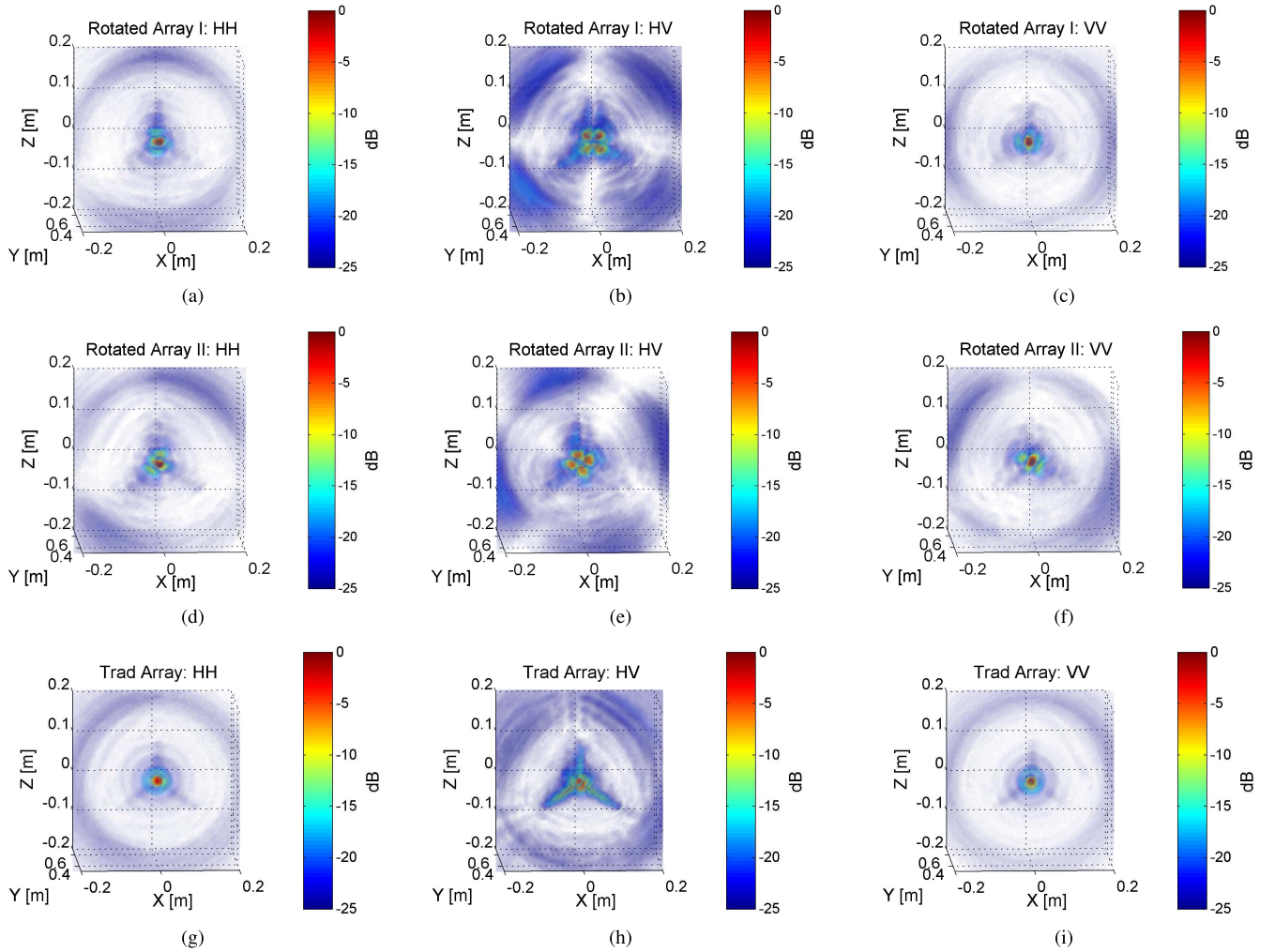
Fig. 5. 3-D polarimetric images of a TCR formed with the experimental measurements by the three antenna arrays. (a)–(c) HH-, HV-, and VV-pol images focused with the measurements of rotated antenna array I. (d)–(f) Measurements of rotated antenna array II. (g)–(i) Measurements of traditional antenna arrays (array III).
