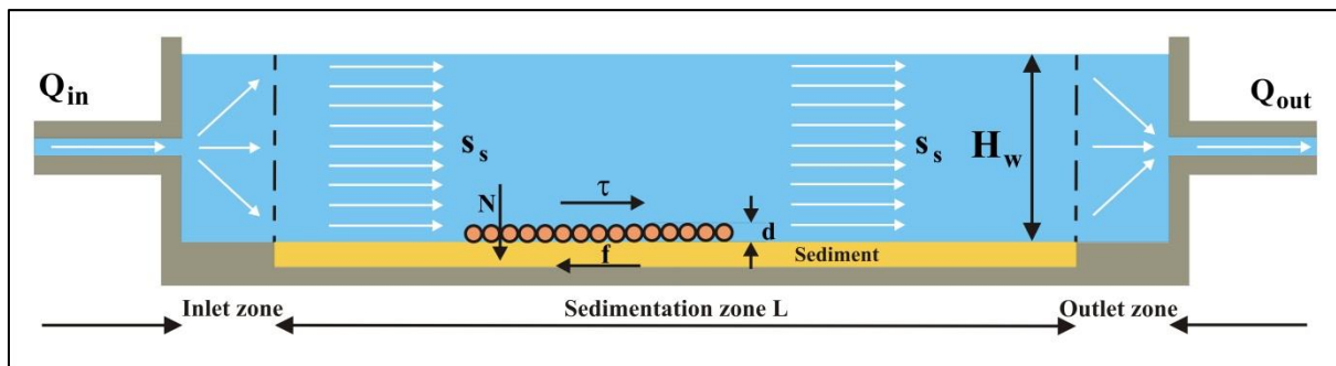
Figure 10-28: The equilibrium of forces on a particle.
