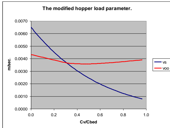
Figure 10-33: d=0.10 mm.
