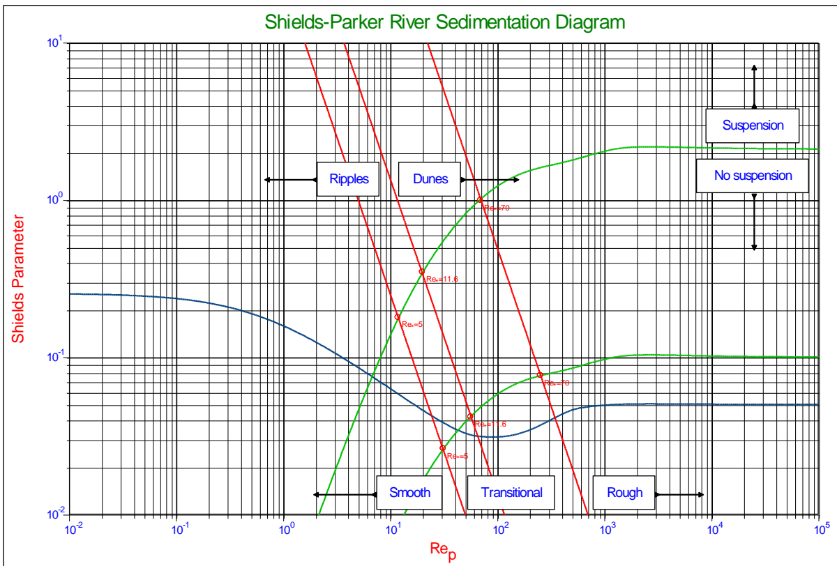
Figure 4-23: The Shields-Parker diagram as a function of the particle Reynolds number.
