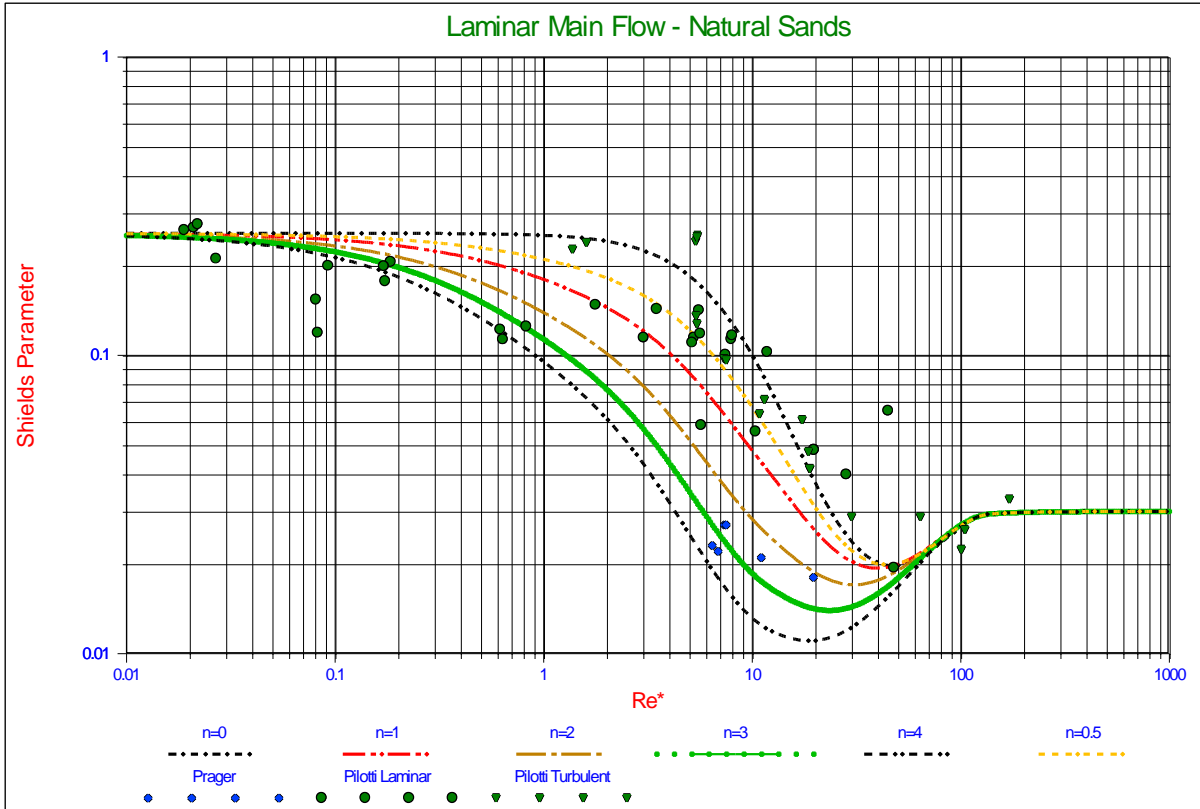
Figure 4-20: Measurements and calculation in a laminar main flow.
