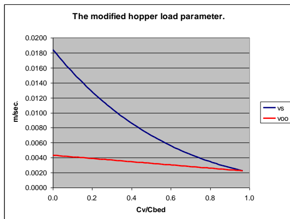
Figure 10-37: d=0.18 mm.
