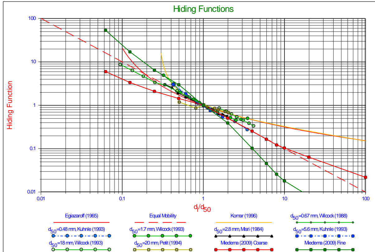
Figure 6-6: Hiding functions.
