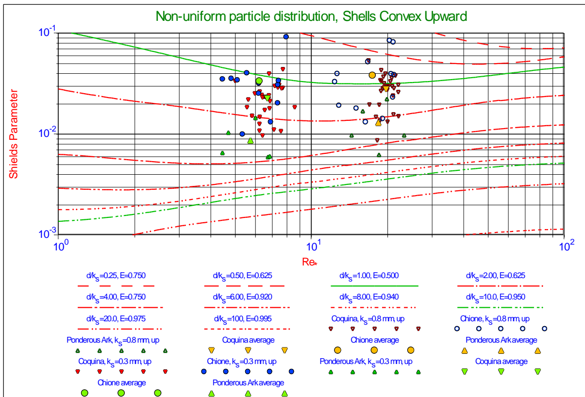
Figure 6-10: Shells convex upward.
