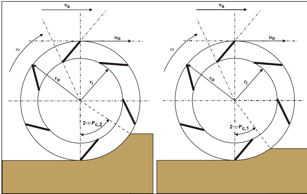
Figure 7-17: The percentages cut in segments 1 and 2.
