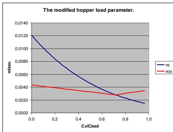
Figure 10-35: d=0.14 mm.
