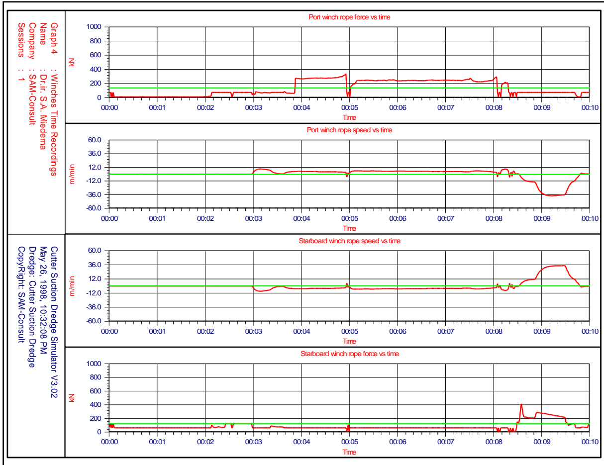
Figure 9-4: The output of the winch parameters.
