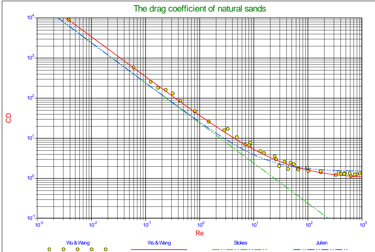
Figure 1-5: Drag coefficient for natural sediments ( S_f=0.7 ) (Wu & Wang, 2006).
