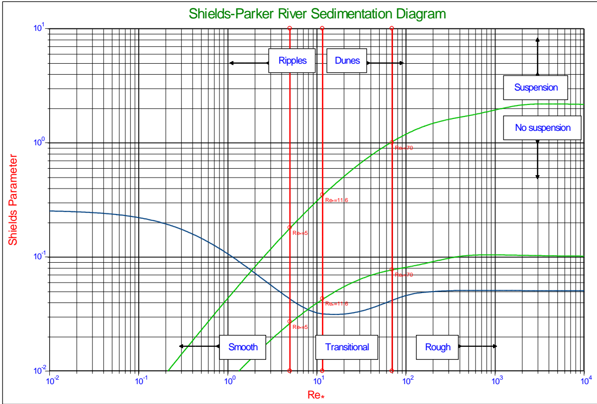
Figure 4-22: The Shields-Parker diagram as a function of the roughness Reynolds number.
