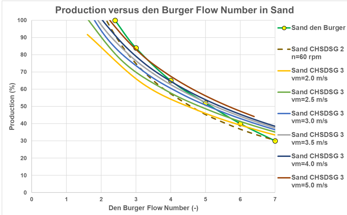
Figure 7-40: Production in sand, n from 20 to 200 rpm, including filling degree effect, model cutter head with \epsilon=3.5 .
