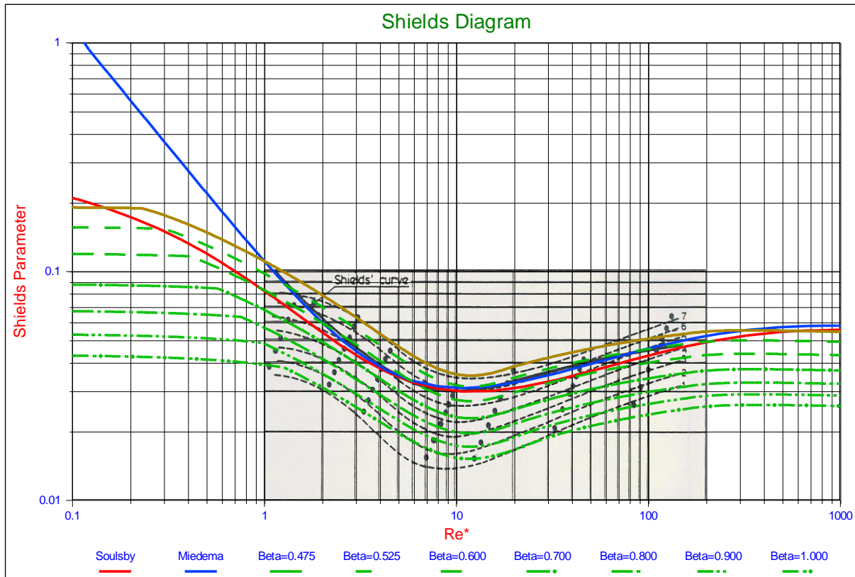
Figure 10-85: The 7 levels of erosion according to Delft Hydraulics (1972).
