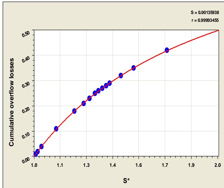
Figure 10-49: The cumulative overflow losses vs S^* , c_b re-calculated.
