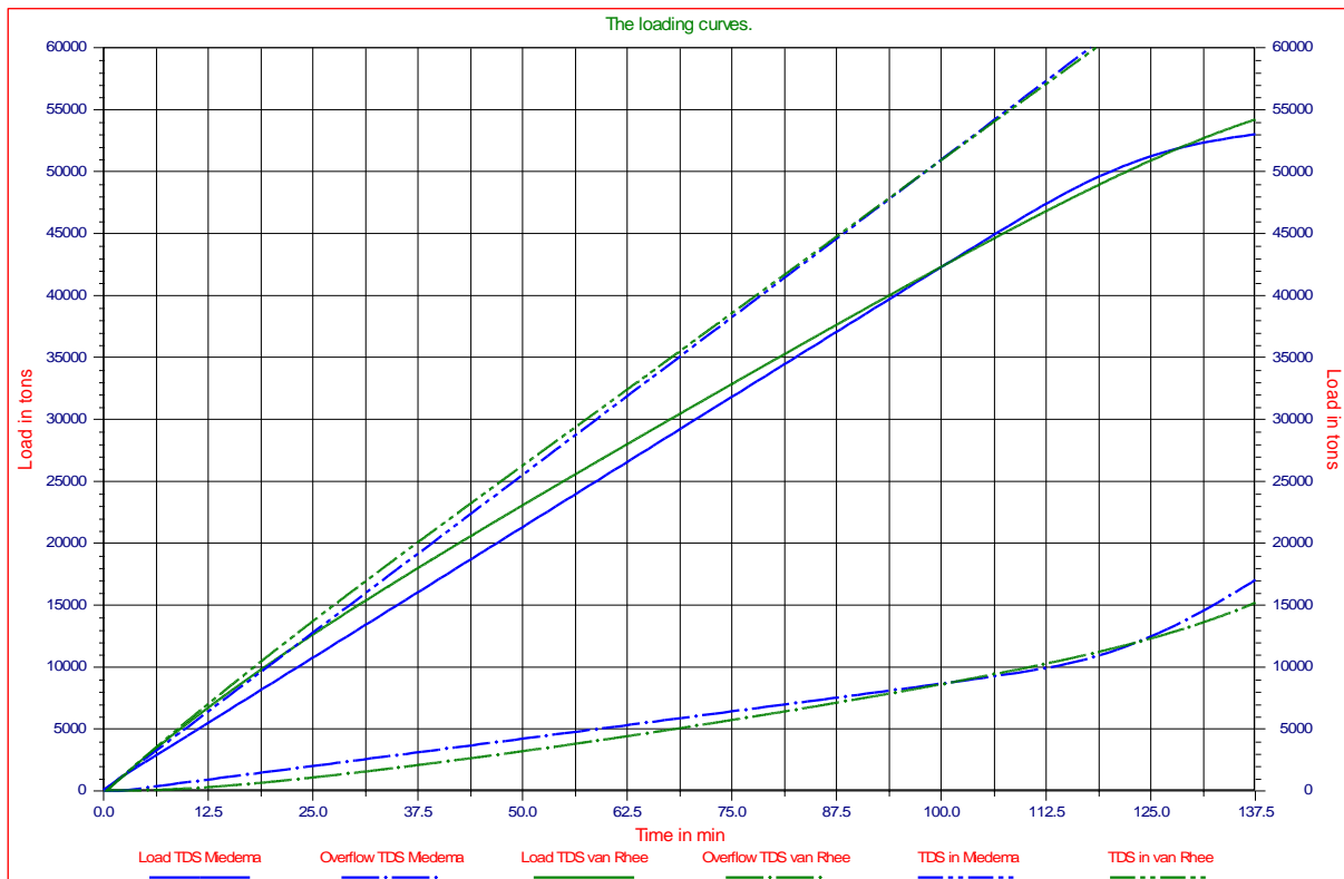
Figure 10-75: Comparison of the two models for the Mega hopper.
