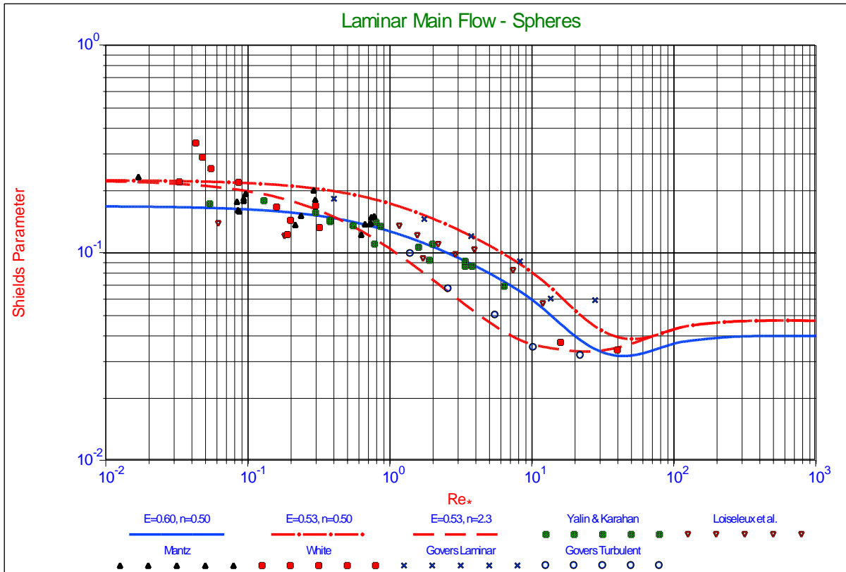
Figure 4-21: Spheres in a laminar main flow.
