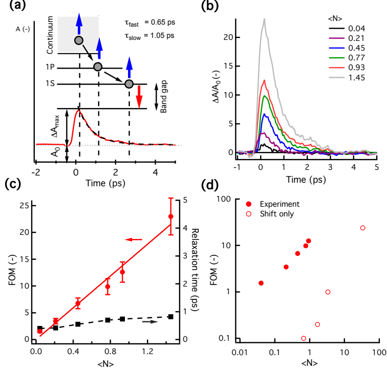
Figure 3: Pump power dependence (a) Schematic of proposed mechanism of 1P-1S limited hot carrier cooling in relation the observed response at the matching wavelength. A bi-exponential fit yields a fast and slow relaxation rate of 0.65 ps and 1.05 ps respectively. (b) Transients of differential absorbance \Delta A normalized to the linear absorbance A_0 for increasing pump fluence as expressed by increasing average exciton population \langle N \rangle (c) FOM (red circles) - the maximum of the \Delta A/A_0 transients of Figure 3b - for increasing fluence plotted with decay constant (black squares). A linear fit ( \text{FOM} = C \times \langle N \rangle ) to the data is shown (solid red line). (d) Expected FOM for a case of pure spectral shifting, calculated according to Geiregat et al. 16 A shift of 3 meV was used per created exciton. We clearly see that the observed modulation is much stronger (up to 2 orders of magnitude) than ever to be expected from multi-X induced shifts. This confirms the idea of competition of interband bleach with (hot and cold carrier) intraband absorption only.
