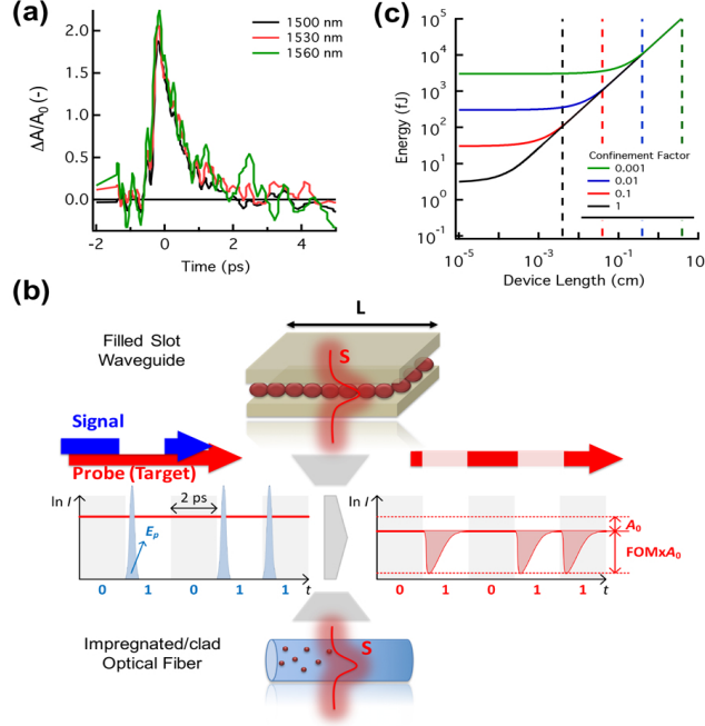
Figure 5: Integration with photonic devices (a) Demonstration of burst absorption in thin (75 nm) spincoated film of QDs on a glass substrate ( \langle N \rangle ), (b) Wavelength conversion scheme with incident pump (or signal, dashed blue)/probe (or target, solid red) sequence and corresponding output indicating the meaning of the FOM, using either a typical integrated SOI design with slot waveguide ( \Gamma = 0.1 ) containing nanocrystals or a impregnated or QD covered glass fiber ( \Gamma = 0.001 ). (c) Evaluation of switching energy per bit (in femtojoule) and device interaction length (in cm) for a variety of optical confinement factors with 3 dB extinction (vertical dashed lines) of the target wave without pump pulse present. Additional calculations are added in the Supporting Information.
