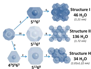
Figure 1. Clathrate's structures: cages, water units and (reproduced from reference 12 with permission from ELSEVIER) [12].
