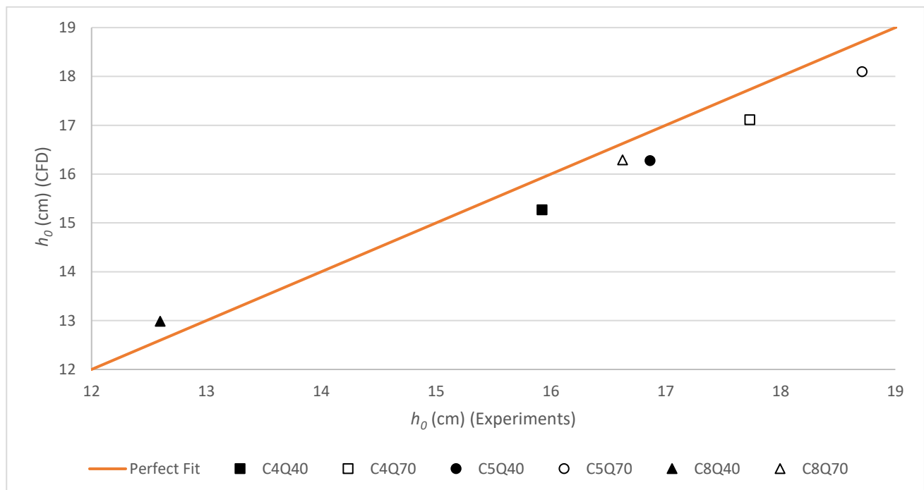
Figure 2. Comparison of measured (Yildiz and Uijttewaai 2023) and modeled upstream flow depths ( h_o ) at each case.
