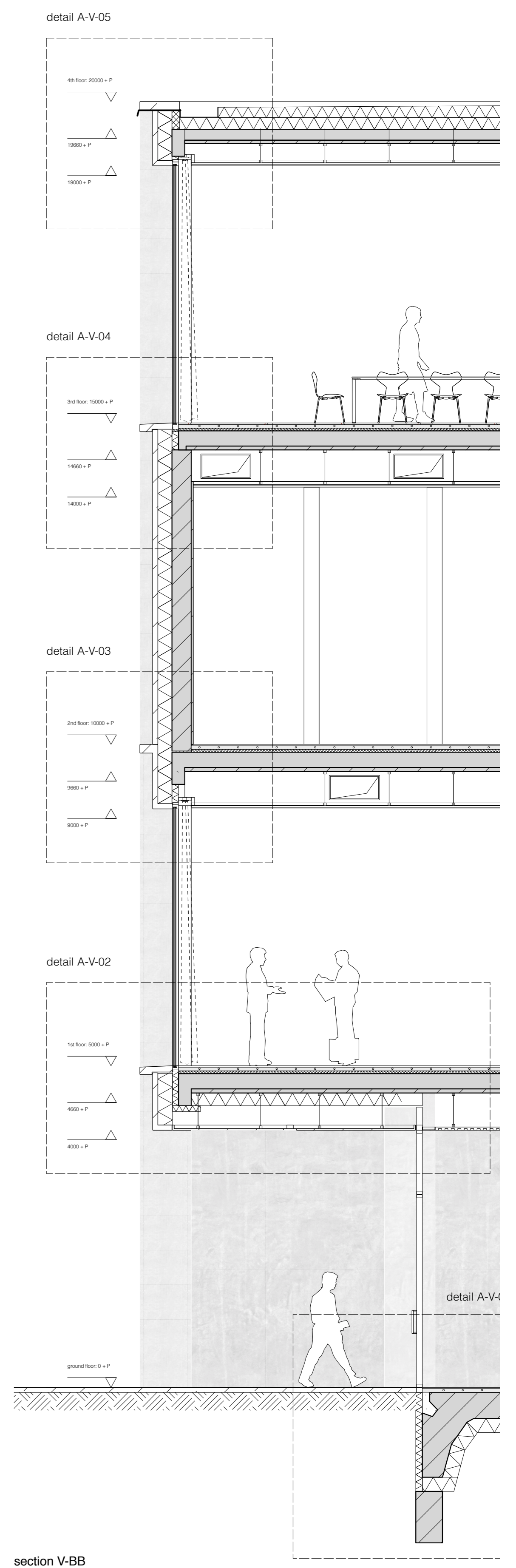
section V-BB
