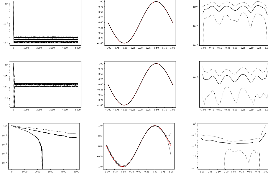
Figure 5: Estimation results of the polynomial regression problem using the stochastic gradient process with reflected Brownian motion process with \sigma = 5 (top row), \sigma = 0.5 (centre row), and \sigma = 0.05 (bottom row). The figures depict the mean over 100 runs (black solid line), mean \pm standard deviation (black dotted line). Left column: trajectory of the rel_err over time; centre column: comparison of \Theta (solid red line) and estimated polynomial; right column: estimation error in terms of abs_err.
