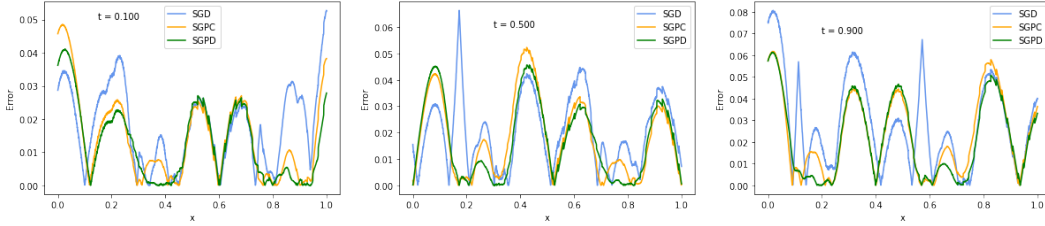
Figure 11: The plots of the test error at time t = 0.1, 0.5, 0.9 . We evaluate the models at 2000 uniformly sampled points. For each method, the predicted values are taken by averaging over the predicted values from the best models (the model that achieves the lowest training loss within the 600 iteration steps) in 30 random experiments. At each point x , the error calculated by taking the absolute value of the difference between the predicted value and the true solution.
