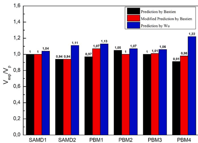
Fig. 7. Comparison of punching shear strength between experimental and predicted results [56,58,59]. (Note: V_{exp}/V_p indicates the ratio between experimental and predicted results, and the series of SAMD samples were tested by Wuest [71], and the series of PBM sample were tested by Bastien [56].).
