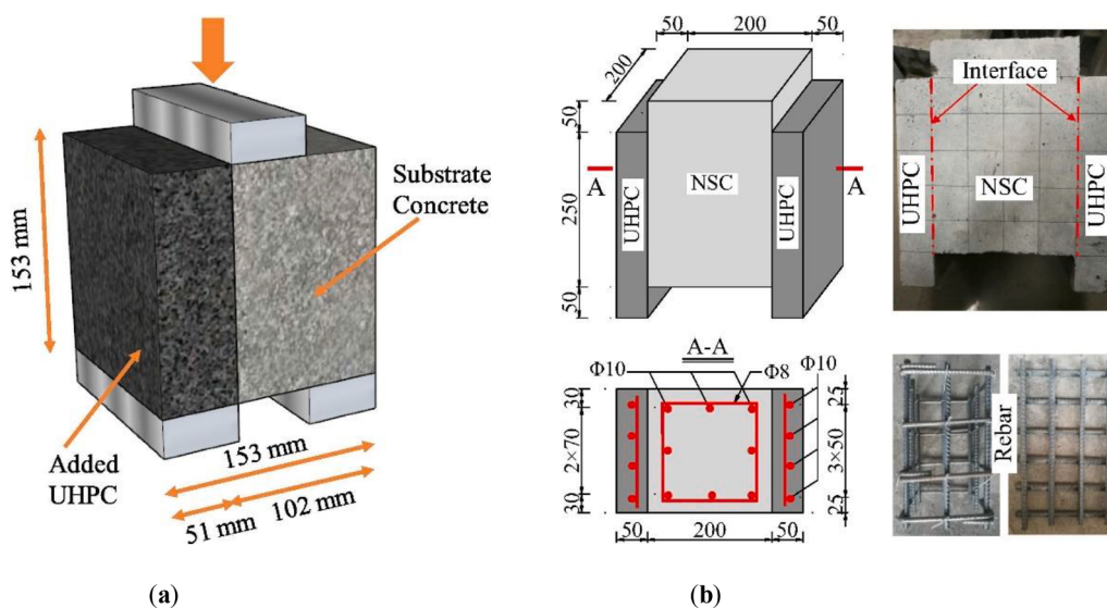
Fig. 11. Shear test: (a) Bi-surface shear [99]; (b) Double-sided shear [100].
