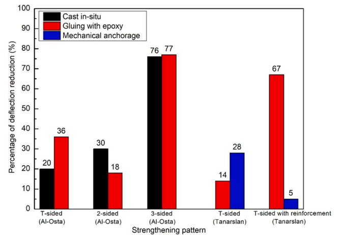
Fig. 17. Deflection reduction with different bonding techniques (calculated as (1 - \Delta_s/\Delta_c) \times 100\% , \Delta_s is displacement at peak load of strengthened beam, \Delta_c is displacement at peak load of control beam) [77,107].
