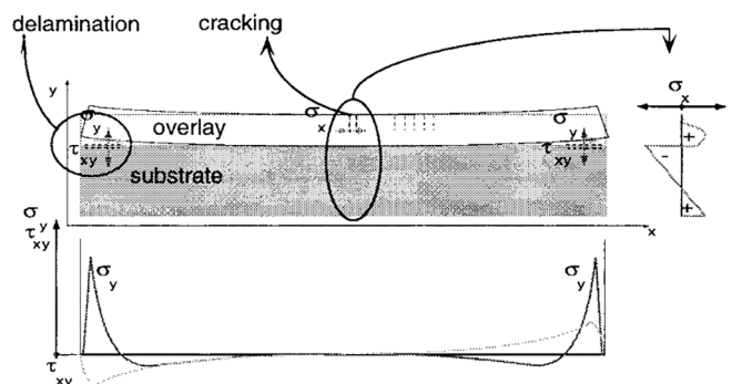
Fig. 20. Damage mechanisms in strengthening systems [82,118].
