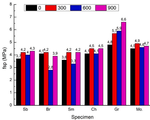
Fig. 23. Effect of freeze-thaw cycles on splitting tensile strength of composite specimen ( f_{sp} =splitting tensile stress, Sb = sandblasted; Br = Brushed; Sm = smooth; Ch = chipped; Gr = grooved; Mo = monolithic (only concrete)) [127].
