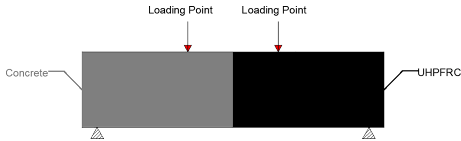
Fig. 13. Four-point bending test.
