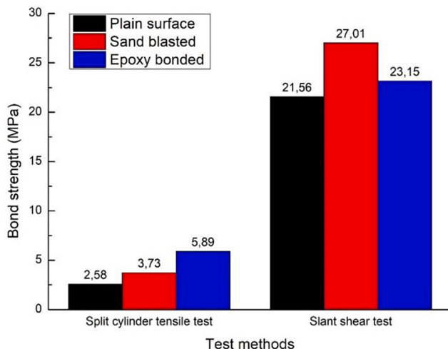
Fig. 14. Bond strength test results [77].
