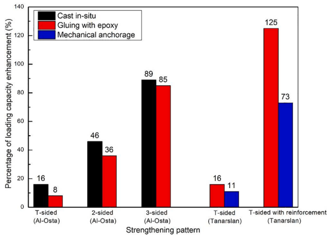
Fig. 16. Loading capacity enhancement with different bonding techniques (calculated as (F_{u,s}/F_{u,c} - 1) \times 100\% , F_{u,s} is peak load of strengthened beam, F_{u,c} is peak load of control beam) [77,107].
