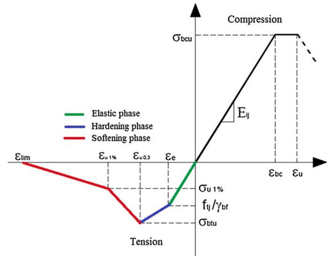
Fig. 8. The uniaxial stress-strain curve for UHPFRC [75].
