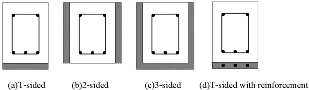
Fig. 15. Strengthening configuration [77,107].
