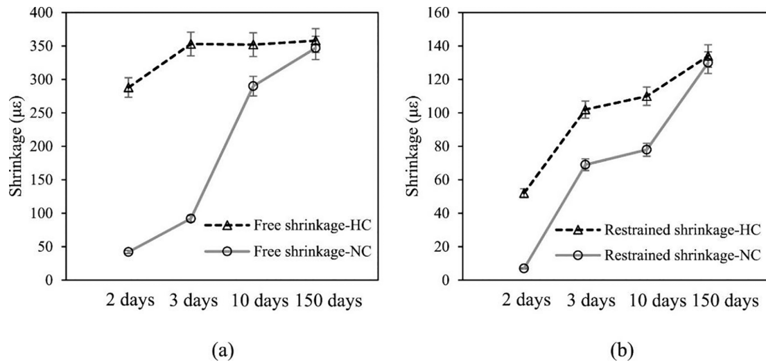
Fig. 22. Free and restrained shrinkage in (a) reinforced UHPFRC and (b) reinforced UHPFRC-concrete composite under different curing conditions (NC and HC respectively denote normal curing and steam curing condition) [126].
