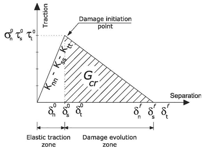
Fig. 9. Bilinear traction-separation law at near interface concrete zone [75].
