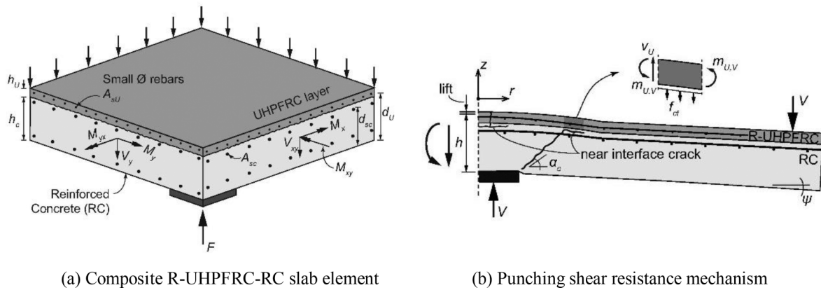
Fig. 5. Punching shear resistance strengthening mechanism with UHPFRC [56].
