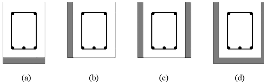
Fig. 3. Typical patterns for shear strengthening with UHPFRC (a) T-sided (Strengthening on tension side); (b) L-sided (Strengthening on one lateral side); (c) 2-sided (Strengthening on two lateral sides); (d) 3-sided beam (Strengthening on three sides).
