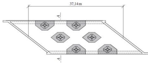
Fig. 6. Slab bridge strengthened with R-UHPFRC over piers (dark areas) in the Switzerland [60].
