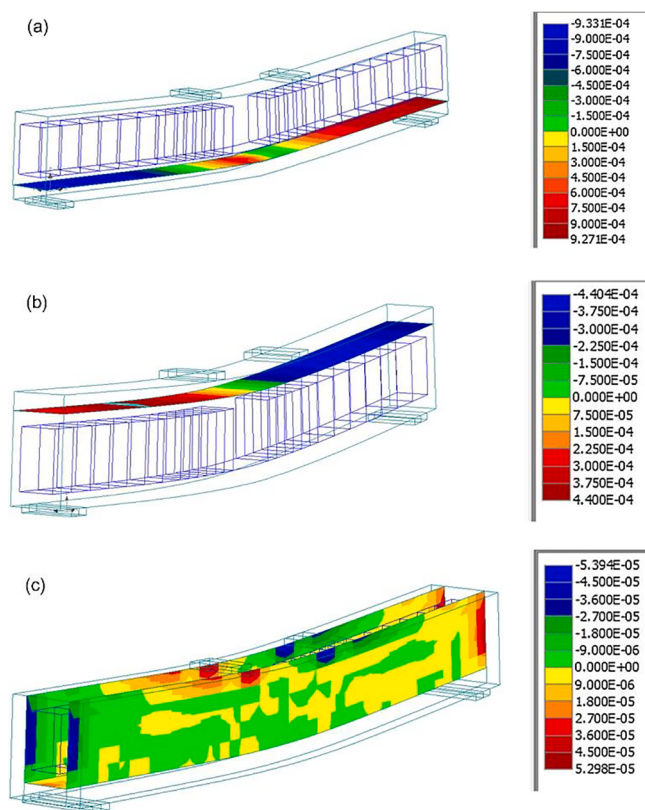
Fig. 25. Interface slip (m) for strengthened beams at ultimate resistance with different UHPFRC configuration: (a) the tensile side, (b) the compressive side, and (c) three sides jacket [135].
