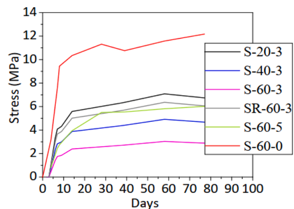
Fig. 21. Restrained concrete shrinkage stresses (S and SR respectively denote strengthened UHPFRC with or without rebars inserted in UHPFRC layer, 20, 40, 60 denote the thickness of UHPFRC layer in mm and 0, 3, 5 denote the volume percentage content of steel fiber.) [124].
