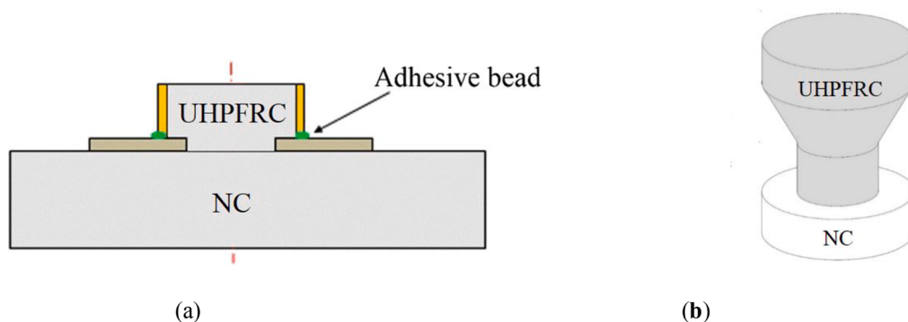
Fig. 10. Test set-up for proposed UHPC debonding test (a) Modified pull-off test (b) Proposed debonding test method [96].
