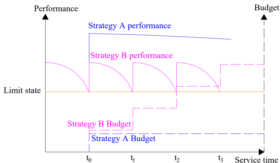
Fig. 1. Two different strengthening strategies for service life maintenance: Strategy A (Structures strengthened with UHPFRC and Strategy B (Structures strengthened with NC) [2].
