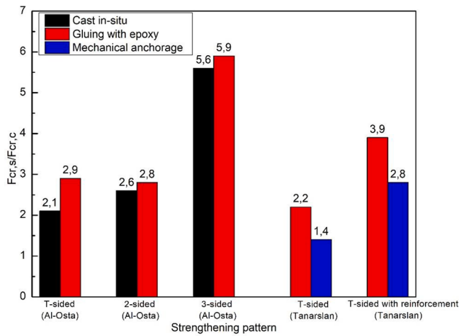
Fig. 18. Cracking resistance improvement with different bonding techniques (denoted as F_{cr,s}/F_{cr,c} , F_{cr,s} is initial cracking load of strengthened beam, F_{cr,c} is initial cracking load of control beam) [77,107].
