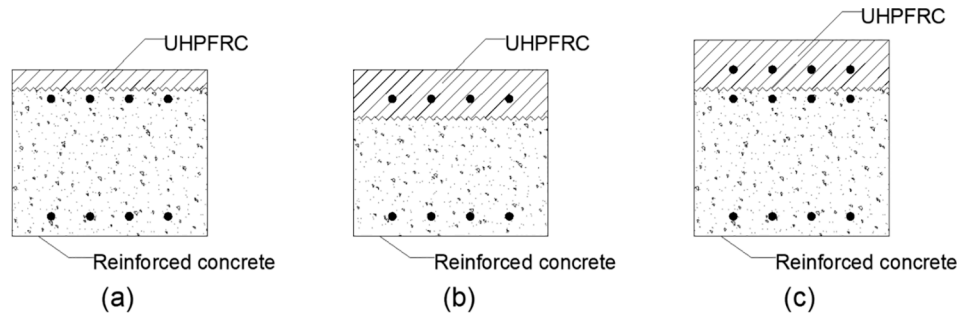
Fig. 2. Concept and principle of composite structural element when UHPFRC layer has a protection function, (a) without and (b) with reinforcement embedded in; and (c) when UHPFRC is used for strengthening, both providing protective function and improving structural resistance [11].
