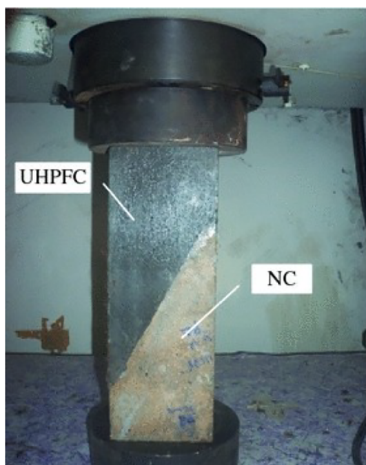
Fig. 12. Slant shear test set-up for UHPFRC-NC specimen [89].
