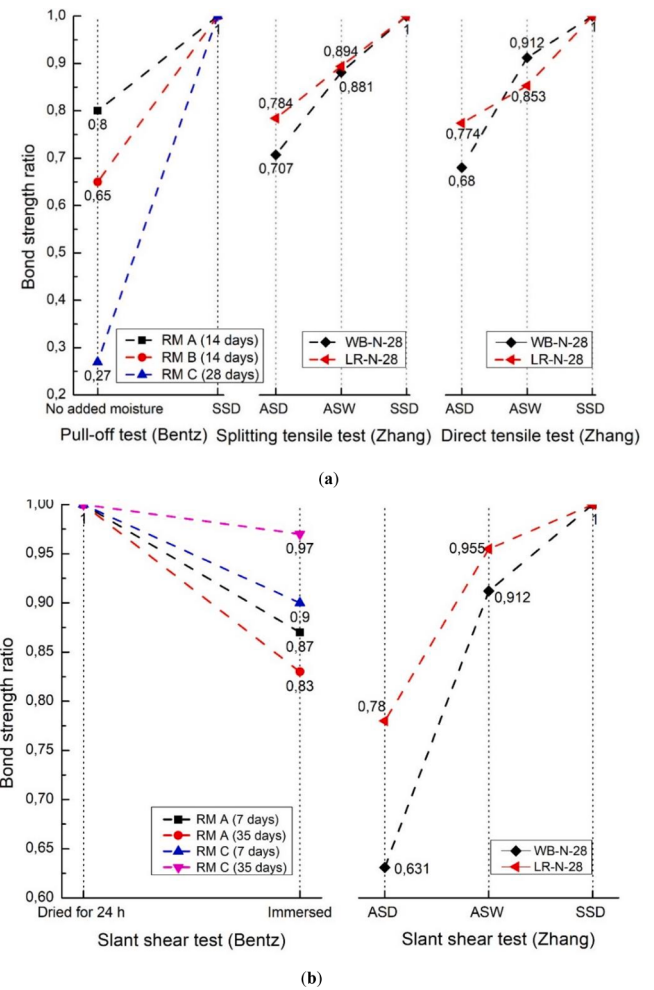
Fig. 19. Effects of moisture state of substrate on relative bond strength for different repair materials (named RM A, RM B and RM C, WB-N-28 and LR-N-28) and different moisture state of substrate (SSD, ASD and ASW stand for saturated surface dry conditions, air surface dry condition and air surface wet condition respectively.): (a) Effects of moisture state of substrate on tensile bond strength for normal strength concrete (RM A, RM B and RM C) and UHPFRC (WB-N-28 and LR-N-28); (b) Effects of moisture state of substrate on shear bond strength for normal strength concrete (RM A, RM B and RM C) and UHPFRC (WB-N-28 and LR-N-28) [87,117].
