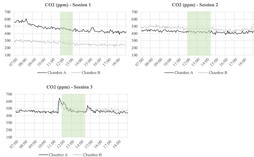
Figure 7. CO 2 levels (ppm) measured during the three sessions from 7.00 to 19.00 every 5 minutes. The highlighted section is the period when the participants executed the experiment and filled the questionnaires.
