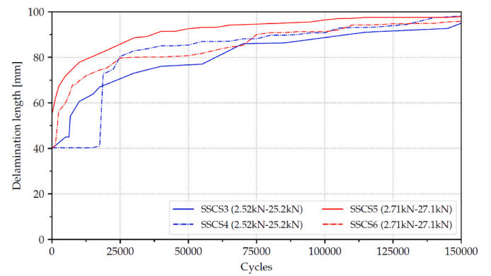
Fig. 13. Delamination length versus cycle count for specimens SSCS3 to SSCS6.
