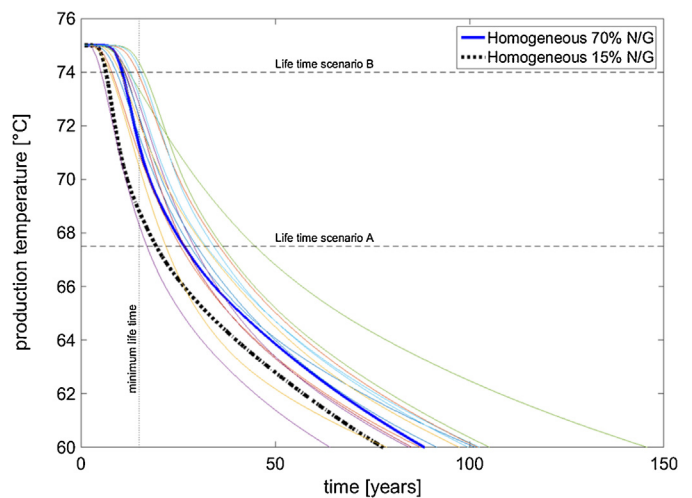
Fig. 12. Production temperature development over time for a 600 m well spacing and a production rate of 100 m 3 /h, for all facies realisations (thin coloured lines) and the two homogeneous models as indicated in the legend. (For interpretation of the references to colour in this figure legend, the reader is referred to the web version of the article.)
