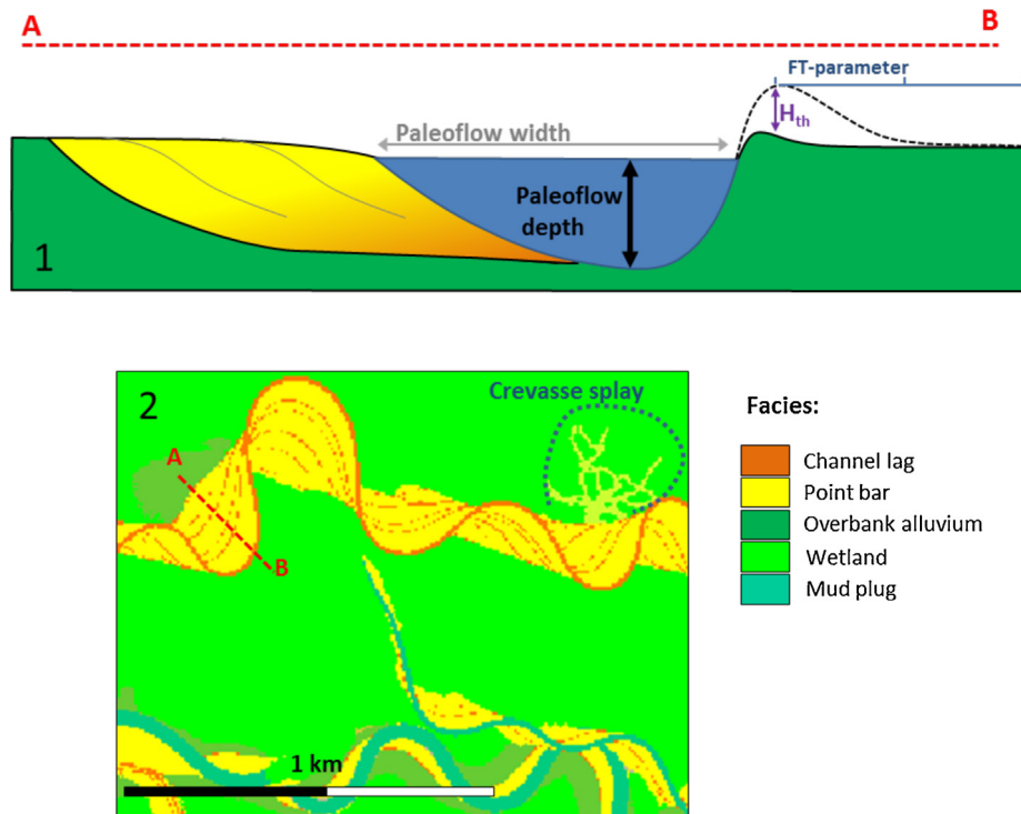
Fig. 2. (1) Process-based facies modelling input parameters in a cross-section of a point bar. Lateral accretion surfaces and coarse channel lag deposits are indicated in the point bar. (2) Map view of facies in the depositional environment.
