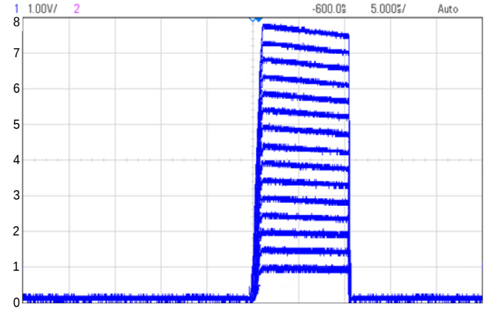
Fig. 23. High-voltage monophasic stimulator output waveform.
