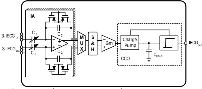
Fig. 3. Bio-potential measurement system architecture.
