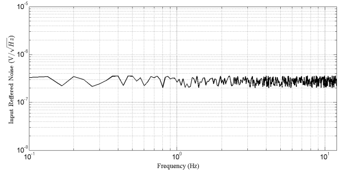
Fig. 19. Bio-impedance channel input referred noise (Gain=40 dB).
