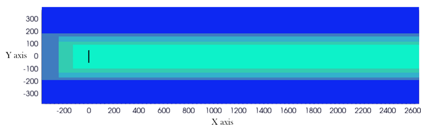
FIGURE 3 Two-dimensional visualization of the domain with the line in black in the middle representing the turbine and the rectangles representing the refinement areas whose dimensions are indicated in Table 2.
