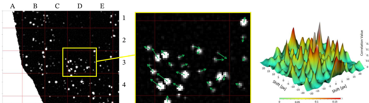
Fig. 6 Seeding distribution and resulting correlation peak in the wake of the side mirror
