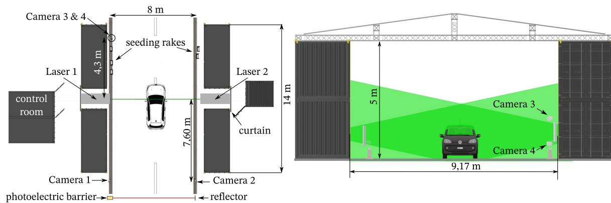
Fig. 1 Schematic setup and position of experimental hardware. (left) top view and (right) front view with Volkswagen up! partly passing the laser sheet
