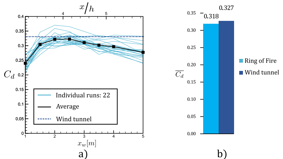
Fig. 13 Drag results Volkswagen up! a in wake distance x_w from 1 to 5 m; b mean drag comparison to windtunnel
