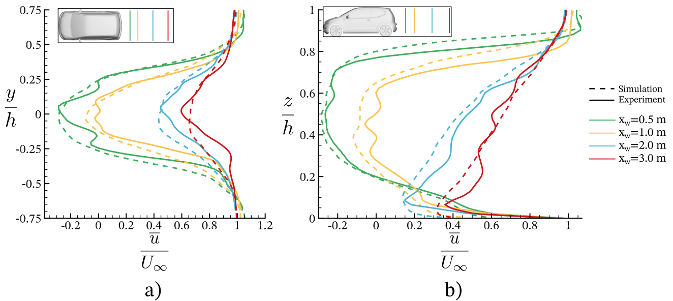
Fig. 12 Volkswagen up! comparison of mean streamwise velocity in the wake. a y-Slice at z/h=0.5 ; b z-slice at y/h=0
