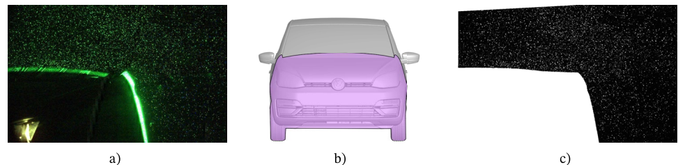
Fig. 5 Samples of an image recording for the car mirror measurement a raw image; b CAD-model and extracted mask (purple); c preprocessed image converted to gray scale and masked
