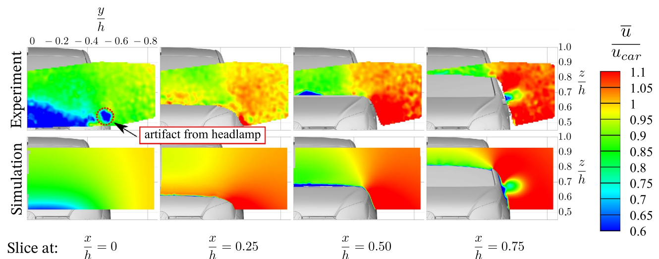
Fig. 9 Comparison of A-Pillar and mirror flow field: dimensionless streamwise mean velocity \frac{\bar{u}}{u_{car}} ; top: experimental results (average of 22 runs); bottom: numerical simulation
