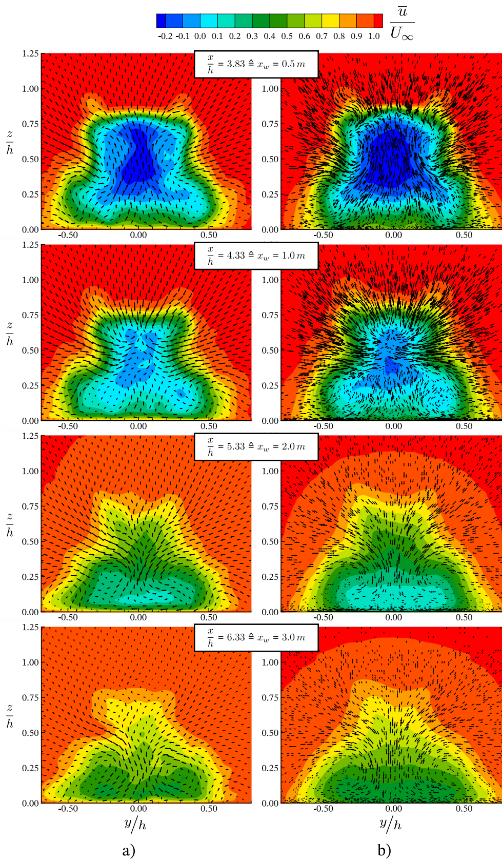
Fig. 11 Volkswagen up! wake contour of streamwise mean velocity \frac{\bar{u}}{U_\infty} at wake distances x_w = 0.5\text{ m}, 1.0\text{ m}, 2.0\text{ m}, 3.0\text{ m} . a Experimental and b numerical results
