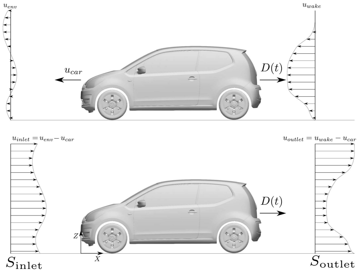
Fig. 7 Galilean transformation from static to moving frame of reference, adapted from Spoelstra et al. (2019)
