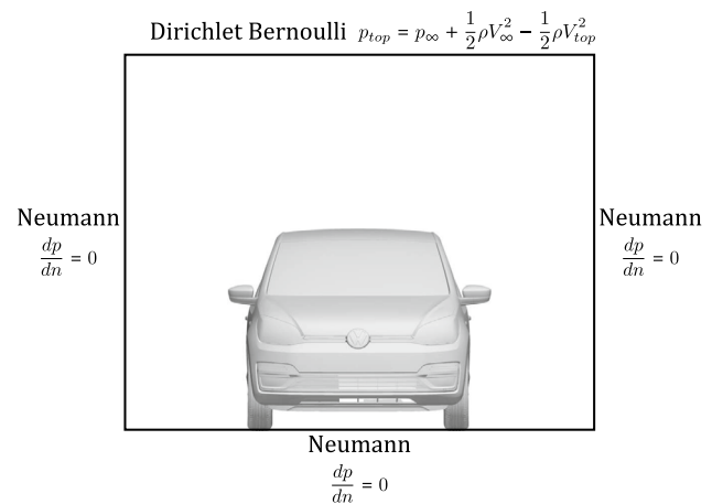
Fig. 8 Boundary conditions for pressure poisson equation
