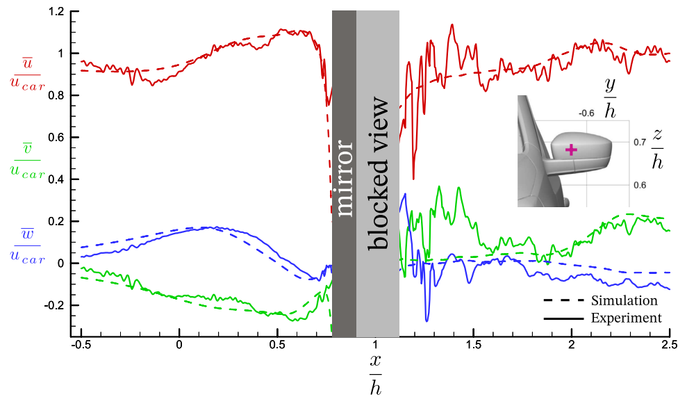
Fig. 10 Dimensionless mean velocities \frac{\bar{u}}{u_{car}} , \frac{\bar{v}}{u_{car}} , \frac{\bar{w}}{u_{car}} along x/h at y/h = -0.56 , z/h = 0.68
