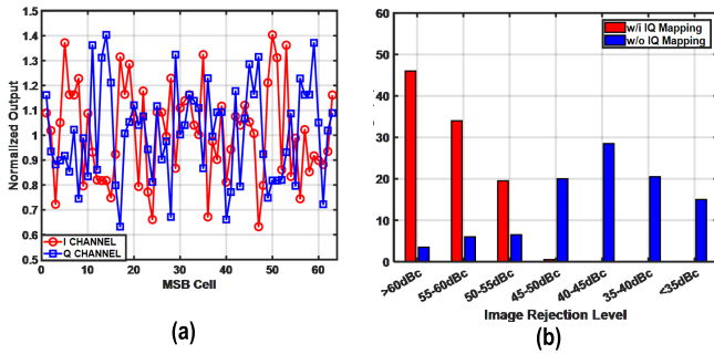
Fig. 7. (a) DNL pattern of MSB cells in the proposed decoder pattern (the DNL pattern of I and Q is inverse to each other). (b) IRR distribution with \sigma = 1 LSB with and without signed IQ-mapping technique in MC simulations.
