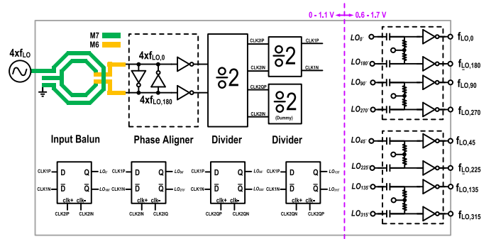
Fig. 13. Schematic of the LO generator.
