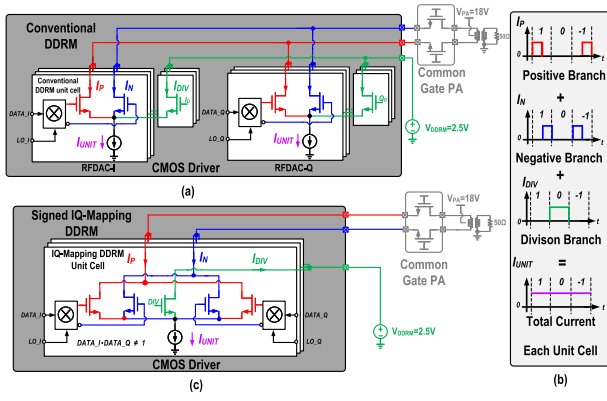
Fig. 3. (a) Conventional DDRM with current division paths. (b) Its unit cell up-converted current waveform. (c) Proposed DDRM architecture with the signed IQ-mapping technique [35].
