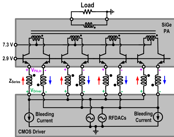
Fig. 14. Conceptual diagram of CB PA with connection to CMOS driver.
