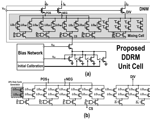
Fig. 12. (a) Schematic of the proposed unit cell with mixing cell of 50% duty-cycle RFDAC and (b) schematic of mixing cell of 25% duty-cycle RFDAC.
