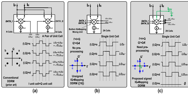
Fig. 5. DDRM evolution. (a) Conventional DDRM. (b) Unsigned IQ-mapping DDRM [16]. (c) Proposed signed IQ-mapping DDRM.
