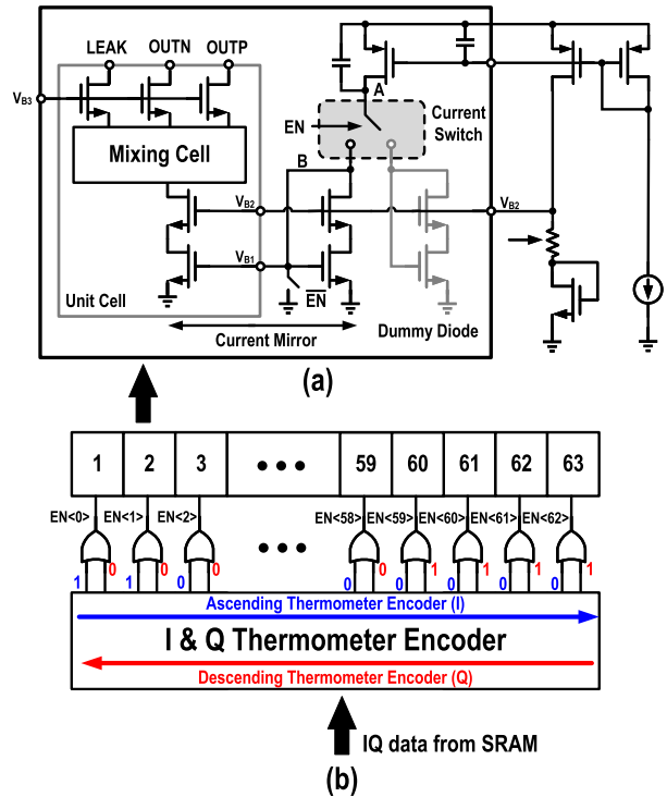
Fig. 10. (a) Topology of current source switch in unit cells and (b) thermometer decoding scheme for dynamic biasing.
