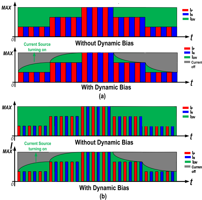
Fig. 9. Concept of dynamic biasing technique: (a) with 50% duty-cycle RFDAC and (b) with 25% duty-cycle RFDAC.
