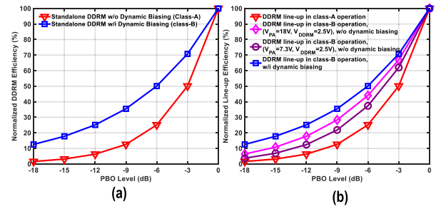
Fig. 4. Normalized drain efficiencies curve of (a) proposed standalone DDRM and (b) TX line-up.
