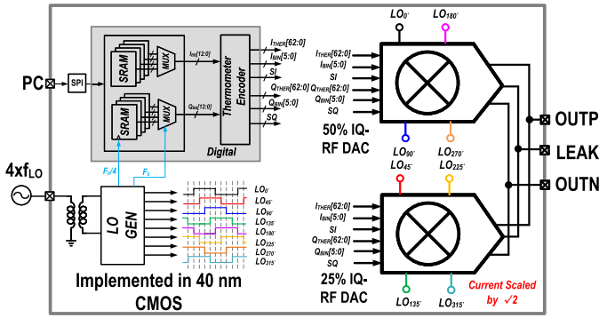
Fig. 11. Proposed DDRM driver's block diagram with standalone testing output circuitry.
