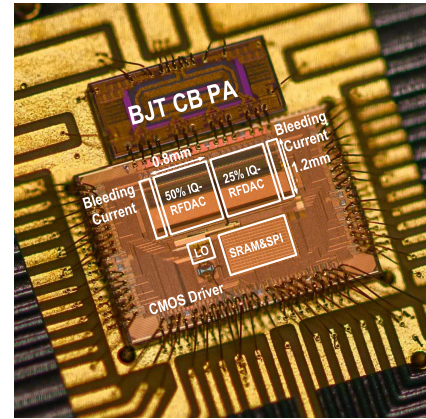
Fig. 15. Chip micrograph of the proposed TX line-up.
