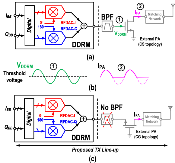
Fig. 1. (a) Conceptual diagram of DDRM drivers to drive a CS/CE PA. (b) Its corresponding voltage/current waveforms. (c) Conceptual diagram of the proposed current-mode DDRM to drive a CG/CB PA.
