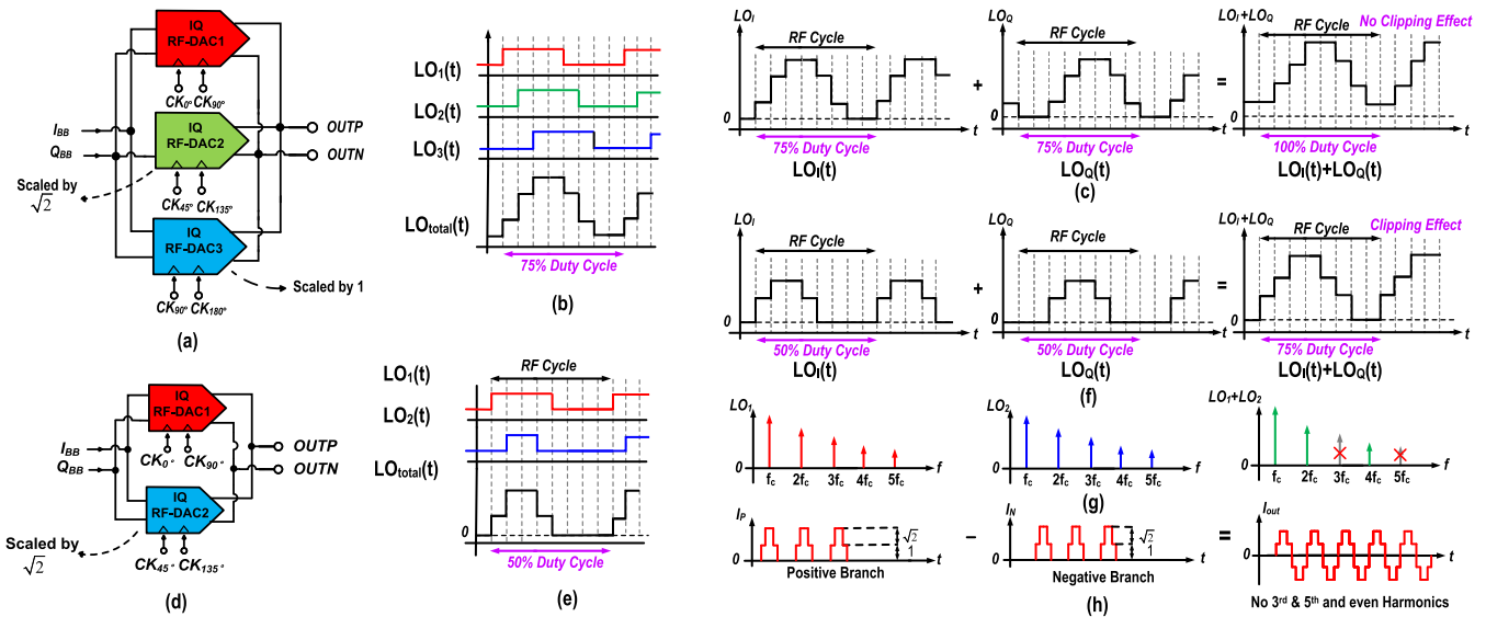
Fig. 8. Principle of class-A HR technique: (a) block diagram, (b) timing diagram, and (c) waveform after IQ summing. Principle of the proposed class-B HR technique: (d) block diagram, (e) timing diagram, and (f) waveform after IQ summing. (g) Spectrum of class-B HR and (h) push-pull output to cancel even harmonics.
