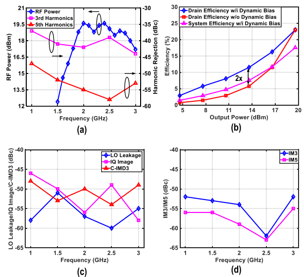
Fig. 16. (a) Measured peak output power, HR ratio versus f_{LO} . (b) Efficiency versus output power with/without dynamic biasing at 2.4 GHz. (c) LO leakage, IQ image, and C-IMD3 in single-tone test versus f_{LO} . (d) IM3 and IM5 in two-tone test versus f_{LO} .
