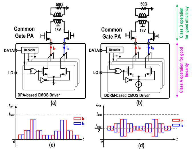
Fig. 2. Block diagram of (a) DPA ([36]) and (b) current-steering RFDAC/DDRMs as a driver of CG/CB PA stages. Responding current waveforms for (c) DPA and (d) RFDAC/DDRMs when applied a two-tone signal, respectively.
