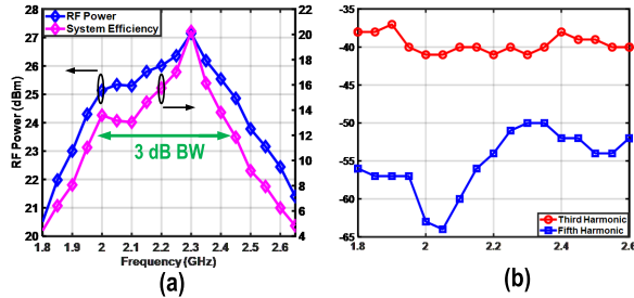
Fig. 18. CW measurement with whole system. (a) Peak power and system efficiency versus f_{LO} . (b) Third and fifth harmonic levels versus f_{LO} .
