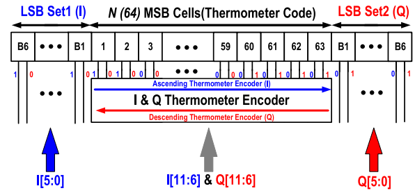
Fig. 6. I/Q complementary decoding scheme.
