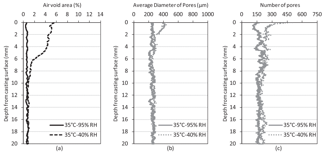
Fig. 11. Air void area (a), average pore diameter (b), and the number of the pores (c) by depth from the casting surface of UHPC-S30 at 35 °C.
