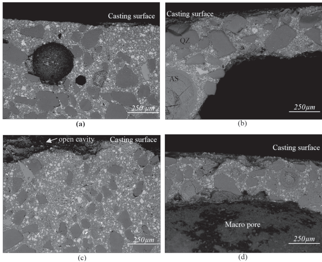
Fig. 15. BSE micrographs of UHPC-S30 stored at 20 °C-95% RH (a), 20 °C-40% RH (b), 35 °C-95% RH (c), and 35 °C-40% RH (d). (QZ: quartz, AS: agglomerated silica fume).
