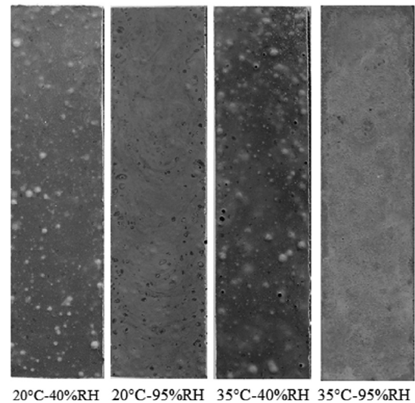
Fig. 4. Surface appearances of UHPC-C mixture depending on climatic condition.
