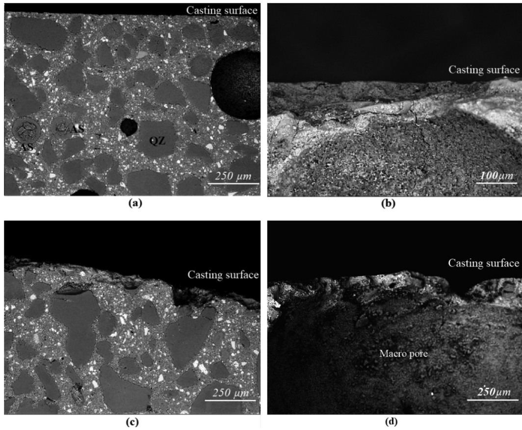
Fig. 14. BSE micrographs of UHPC-C stored at 20 °C-95% RH (a), 20 °C-40% RH (b), 35 °C-95% RH (c), and 35 °C-40% RH (d). (QZ: quartz, AS: agglomerated silica fume).
