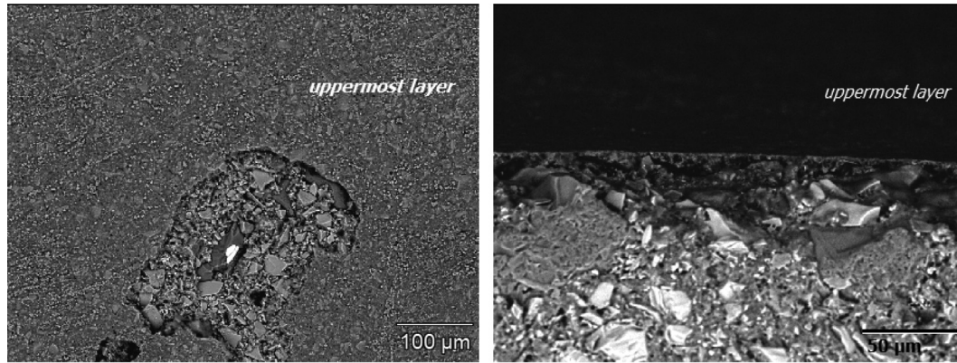
Fig. 18. BSE micrographs from above (a) and cross-section (b) (UHPC-S60 at 35 °C–40% RH).
