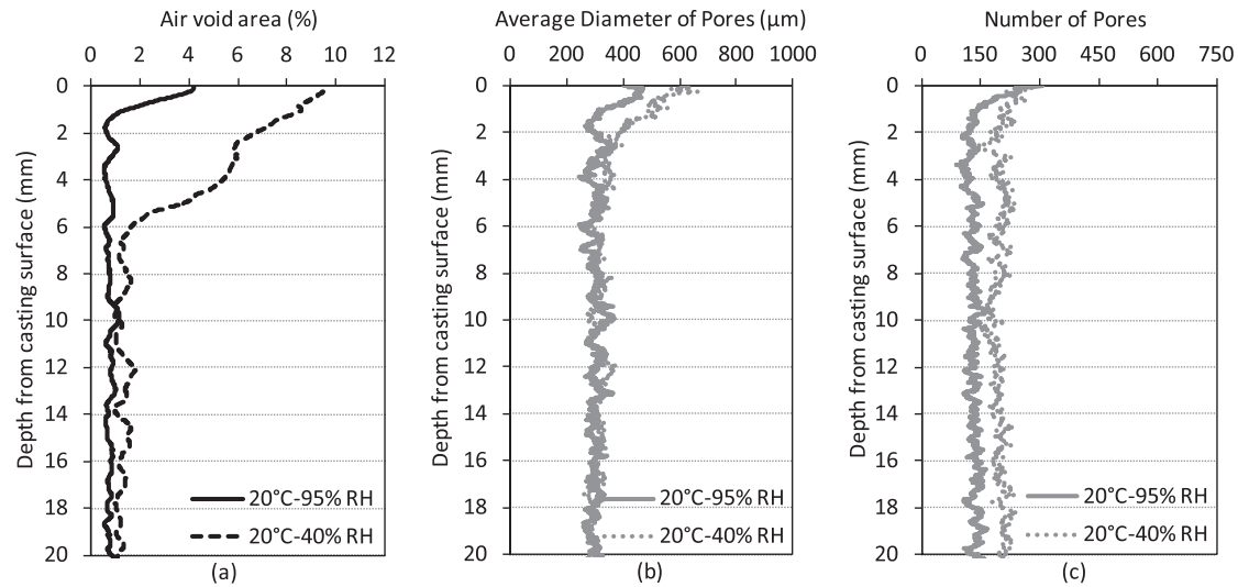
Fig. 8. Air void area (a), average pore diameter (b), and the number of the pores (c) by depth from the casting surface of UHPC-C at 20 °C.
