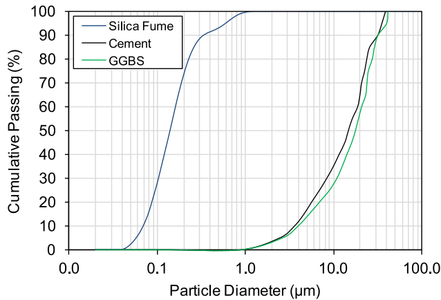
Fig. 1. Particle size distribution of cementitious materials.
