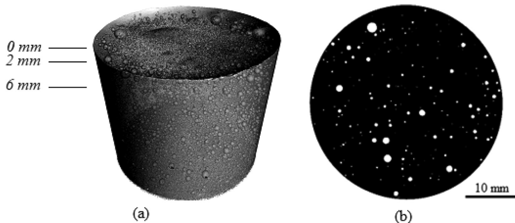
Fig. 7. 3D visualization of porosity (a), 2D slice image after thresholding (b).
