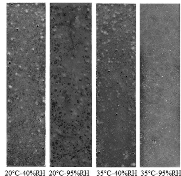
Fig. 5. Surface appearances of UHPC-S30 mixture depending on climatic condition.
