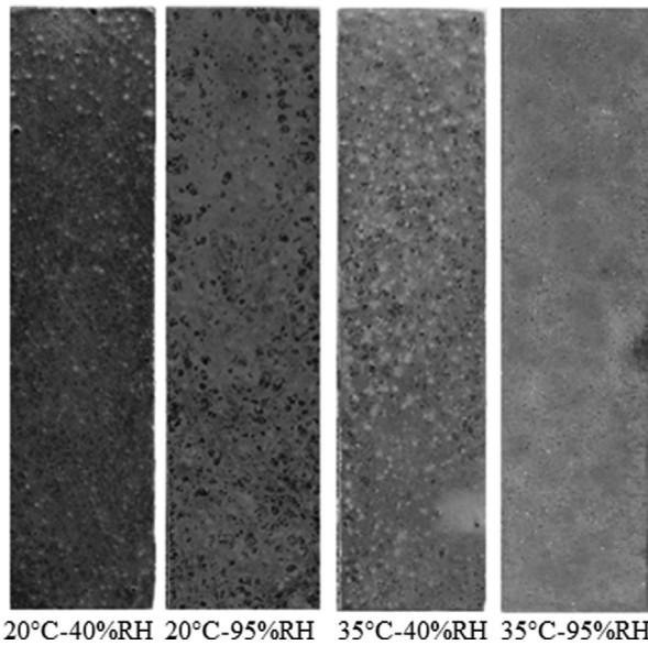
Fig. 6. Surface appearances of UHPC-S60 mixture depending on climatic condition.
