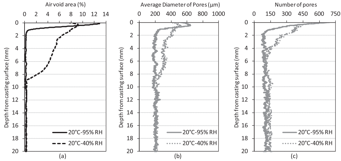
Fig. 12. Air void area (a), average pore diameter (b), and the number of the pores (c) by depth from the casting surface of UHPC-S60 at 20 °C.
