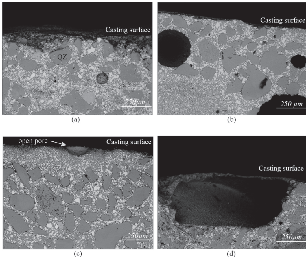
Fig. 16. BSE micrographs of UHPC-S60 stored at 20 °C-95% RH (a), 20 °C-40% RH (b), 35 °C-95% RH (c), and 35 °C-40% RH (d). (QZ: quartz).
