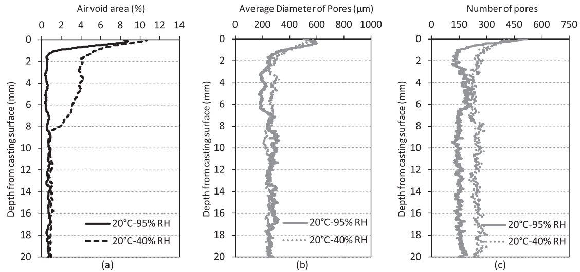
Fig. 10. Air void area (a), average pore diameter (b), and the number of the pores (c) by depth from the casting surface of UHPC-S30 at 20 °C.
