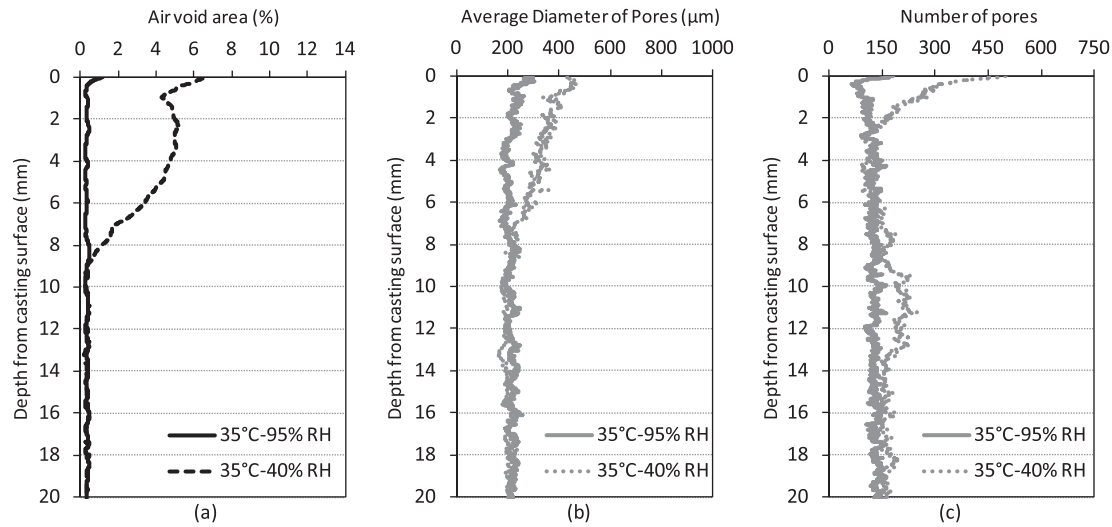
Fig. 13. Air void area (a), average pore diameter (b), and the number of the pores (c) by depth from the casting surface of UHPC-S60 at 35 °C.
