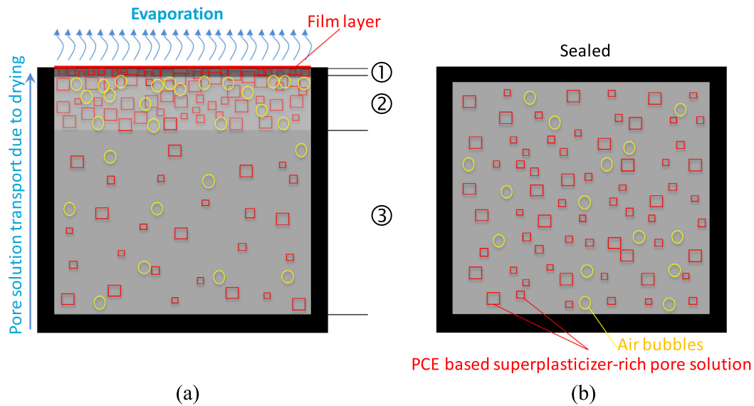
Fig. 19. Illustration of elephant skin formation and multi-layered structure of UHPC (a), prevention of elephant skin (b) (①organic film layer and dense zone due to enrichment of superplasticizer + early hydration products + contraction, ②porous zone due to hindered deaeration, ③the bulk of UHPC).
