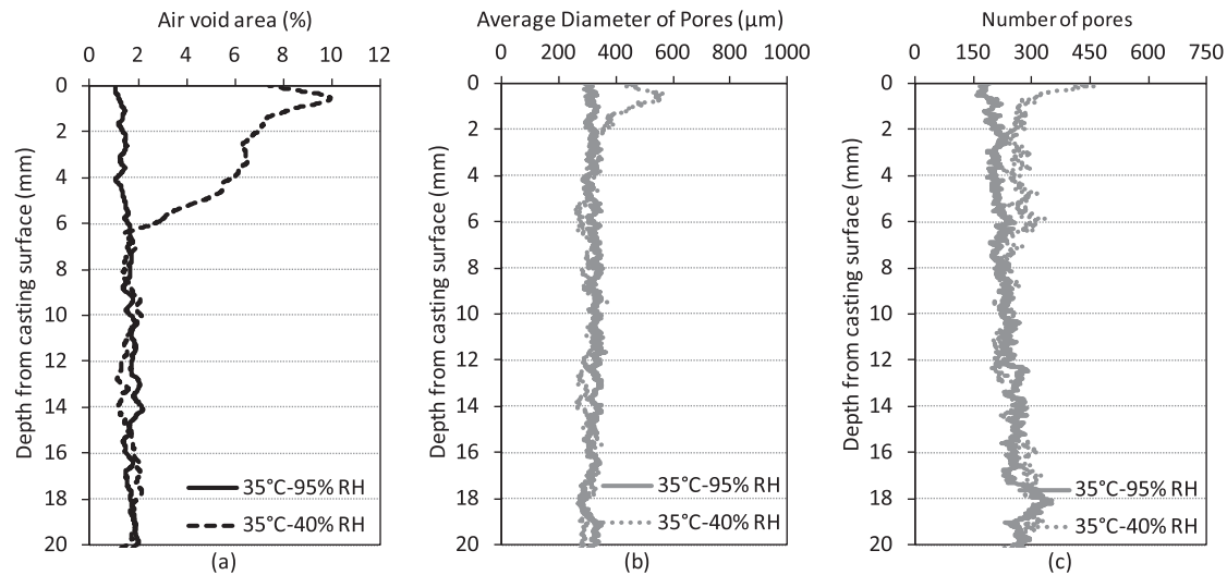
Fig. 9. Air void area (a), average pore diameter (b), and the number of the pores (c) by depth from the casting surface of UHPC-C at 35 °C.
