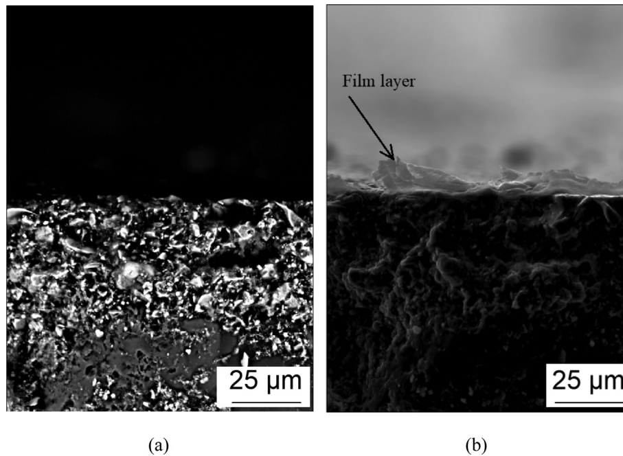
Fig. 17. Typical BSE (a) and SE (b) micrographs of the organic film layer (UHPC-C at 35 °C-40% RH).
