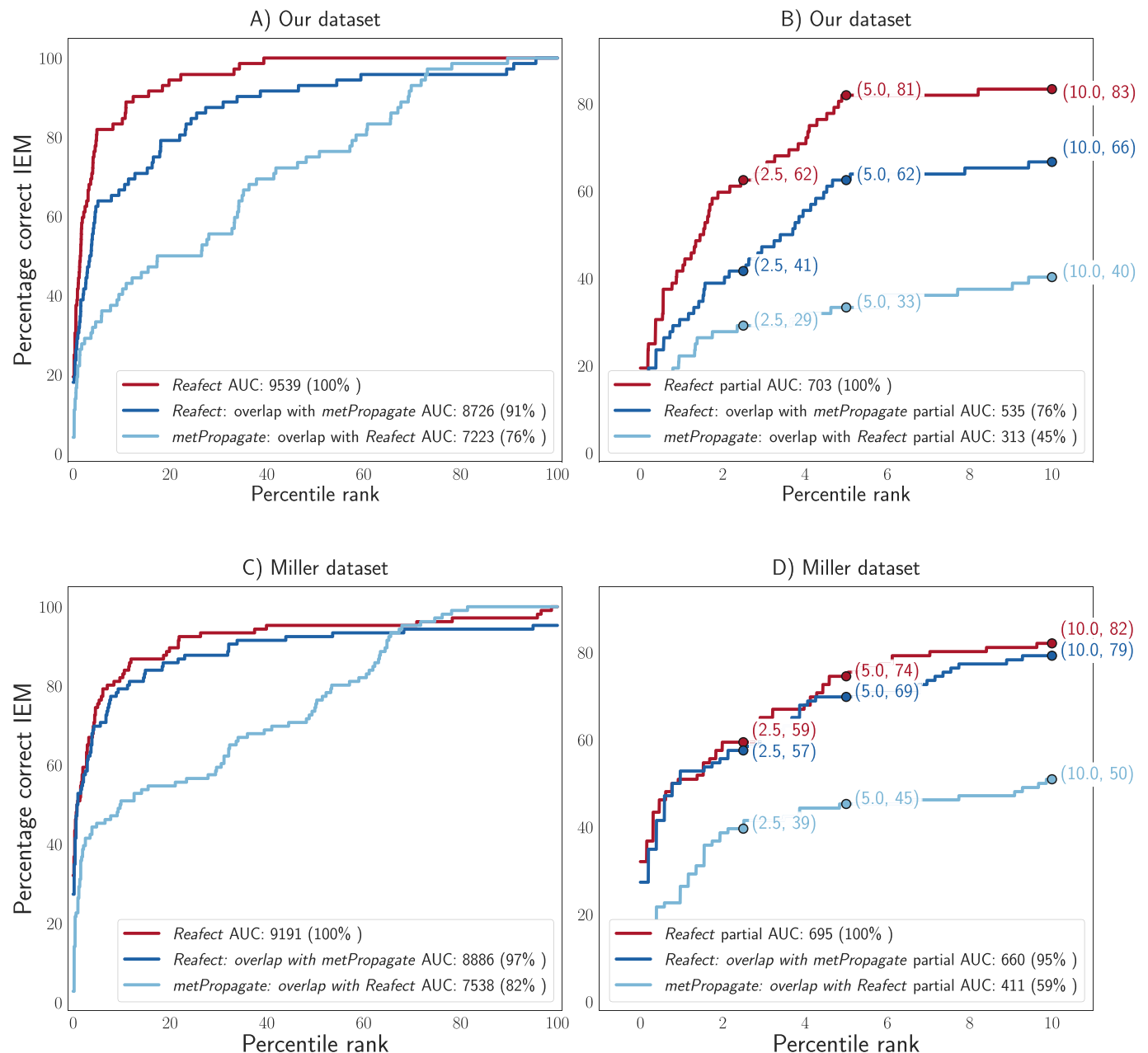
Fig. 3. IEM ranking performances for different approaches as indicated by the legend. Each curve shows the percentage of IEM patient samples for which the percentile rank (PR) of the true enzyme deficiency is within the top x% (horizontal axis) of all considered enzyme deficiencies. Model settings for Reaffect : a = 0.85 , b = 0.35 and c = 0.75 . A) Full performance curves using our dataset. B) Performance curves with PR \leq 10\% using our dataset. C) Full performance curves using the Miller dataset. D) Performance curves with PR \leq 10\% using the Miller dataset. To perform a meaningful comparison between Reaffect and metPropagate a subset of the data was analyzed that contained only metabolites and genes that were included in both approaches (Methods). Note that this selection reduced the performance of Reaffect to 91% and 97% of its original performance on our dataset and the Miller dataset respectively.
