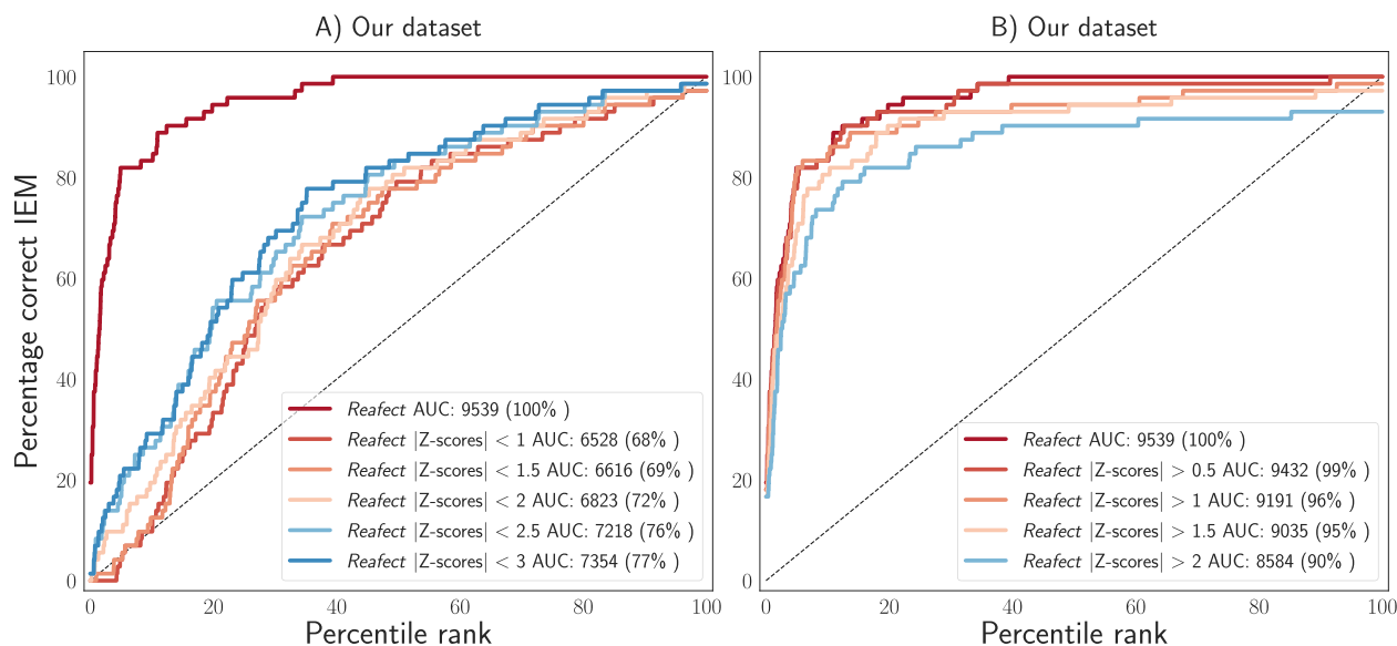
Fig. A6. A) Full performance curves for Reaffect for various Z-score cutoff values, and |Z\text{-score}| < \text{cutoff} . Cutoff values are indicated by the legend. B) Full performance curves for Reaffect for various Z-score cutoff values, and |Z\text{-score}| > \text{cutoff} .
