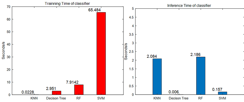
Fig. 8. Average (left) training time (right) inference time of 10-fold cross-validation.
