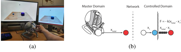
Fig. 2: (a) Tactile Internet setup in our lab showing the the user interacting with a virtual environment. The monitor on the left and right correspond to master and controlled domains, respectively. (b) Conceptual illustration of generation of haptic feedback. HIP is the white circle in the controlled domain.
