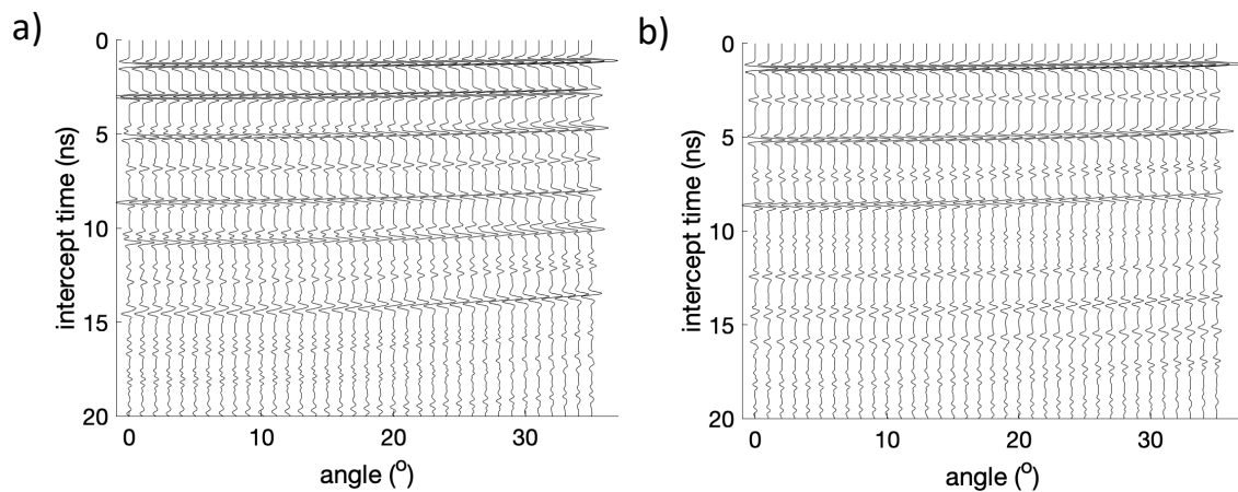
Figure 8. (a) Reflection response from above, R^U(s_1, -x_{3,1}, \tau) , for -x_{3,1} = -0.6 m. (b) Reflection response from below, R^\cap(s_1, x_{3,1}, \tau) , for x_{3,1} = 0.6 m.
