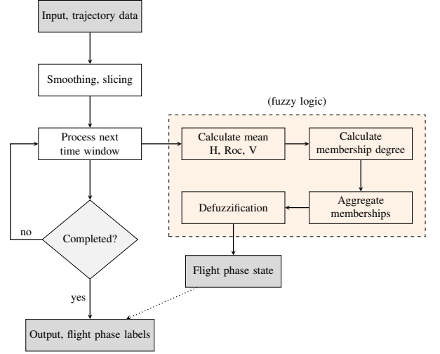
Fig. 6. Flight segmentation with fuzzy logic
