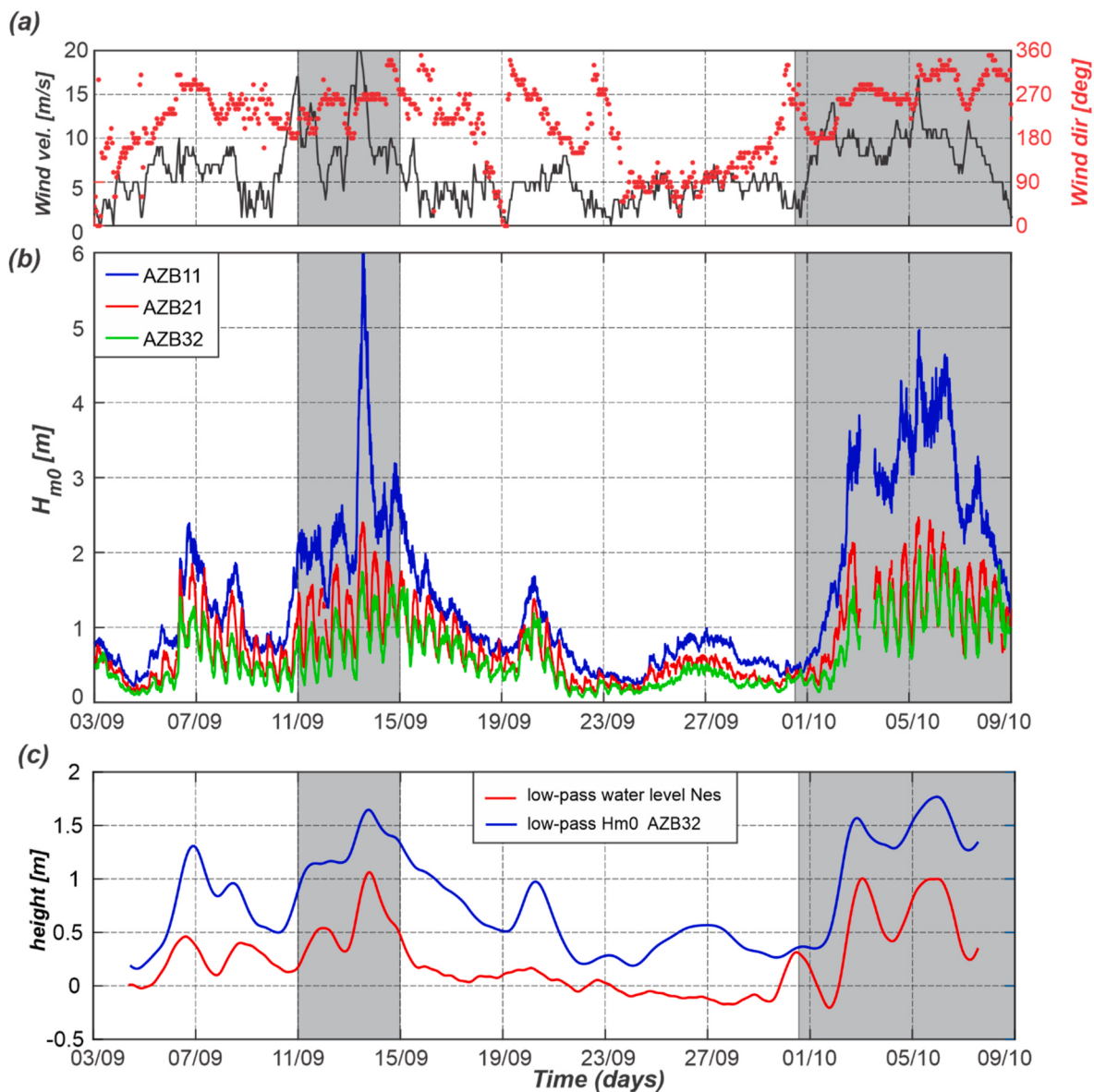
Fig. 8. (a) Wind speed and direction observed at the KNMI station of Terschelling (b). Wave heights observed at the Ameland Zeegat stations AZB11, AZB21 and AZB32. (c) Low-pass filtered water levels (Nes) and wave heights for buoy AZB32. See Fig. 2 for locations. Grey areas indicate elevated levels due to storm Sebastian and Storm Xavier.
