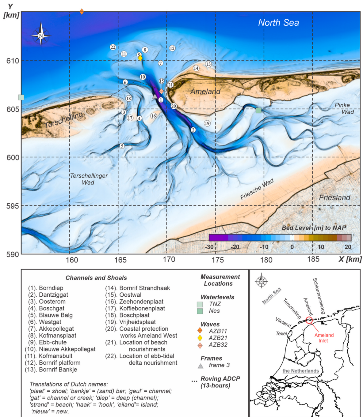
Fig. 2. Overview of the channels and shoals that form the present day Ameland Inlet. The underlying DEM is based on the 2021 Vakkloedingen for the ebb-tidal delta and 2017 measurements of the basin. Bed level is measured with respect to NAP (Normaal Amsterdamse Peil) datum, approximately mean sea level.
