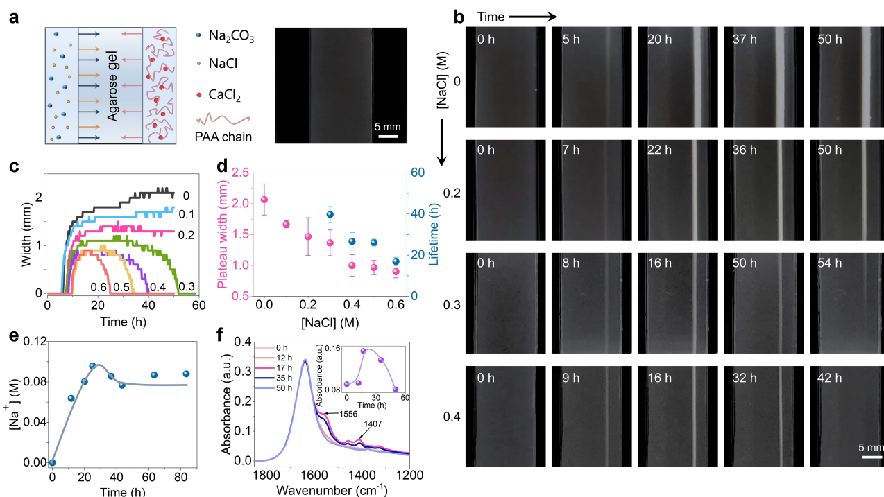
Figure 2. Dynamic growth of 1D supramolecular PAA/ACC hydrogels. a) The formation of a 1D PAA/ACC hydrogel through reaction-diffusion in a 1.0 wt% agarose gel medium; b) snapshots showing the growth process of PAA/ACC hydrogels and c) variation of the hydrogel width over time with different [NaCl]; d) plateau width and lifetime of the hydrogels as a function of [NaCl], the error bars are s.d. calculated from three parallel tests; e) evolution of [Na + ] over time at the region of hydrogel formation, the line is added to guide the eyes; f) ATR-IR spectra showing the dynamic growth process of PAA/ACC hydrogels. Samples in (b)–(d): 2 mL PAA/CaCl 2 (0.114 M/0.02 M, pH 3.5) and 2 mL Na 2 CO 3 /NaCl (0.02 M/ different [NaCl]), additional 0.4 M NaCl were used in (e) and (f).
