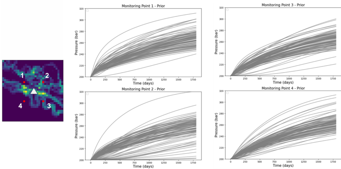
Figure 9 Prior ensemble pressure response at four monitoring points using 100 prior models. The left panel shows the location of the monitoring points around the central injection well. The right panels display the pressure evolution over time at each monitoring point.
