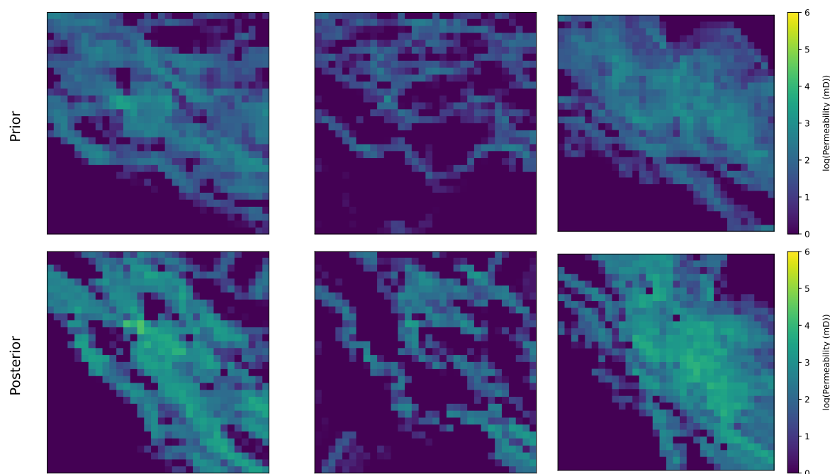
Figure 15 Posterior permeabilities for Hybrid-RML-Surrogate with FNO surrogates.
