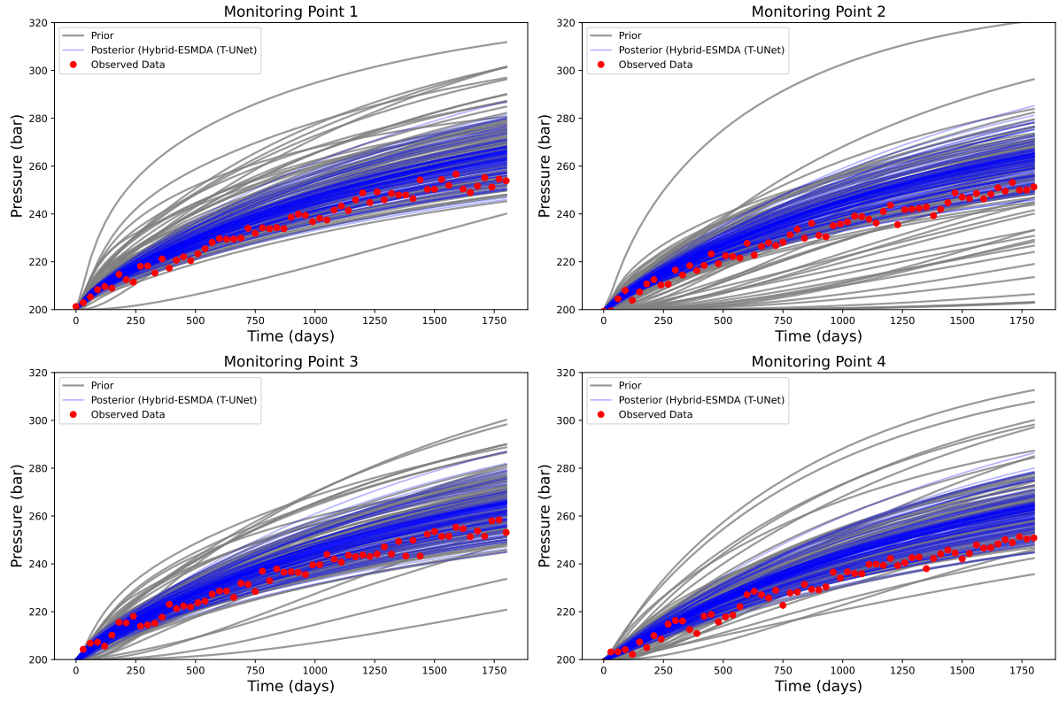
Figure 17 Pressure comparison at monitoring points for Hybrid ESMDA using T-UNet surrogate. Red dots represent a realization of perturbed observed data.
