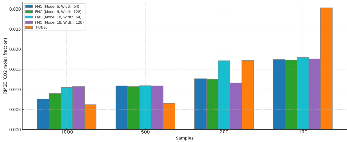
Figure 6 Test RMSE Metrics for CO 2 molar fraction
