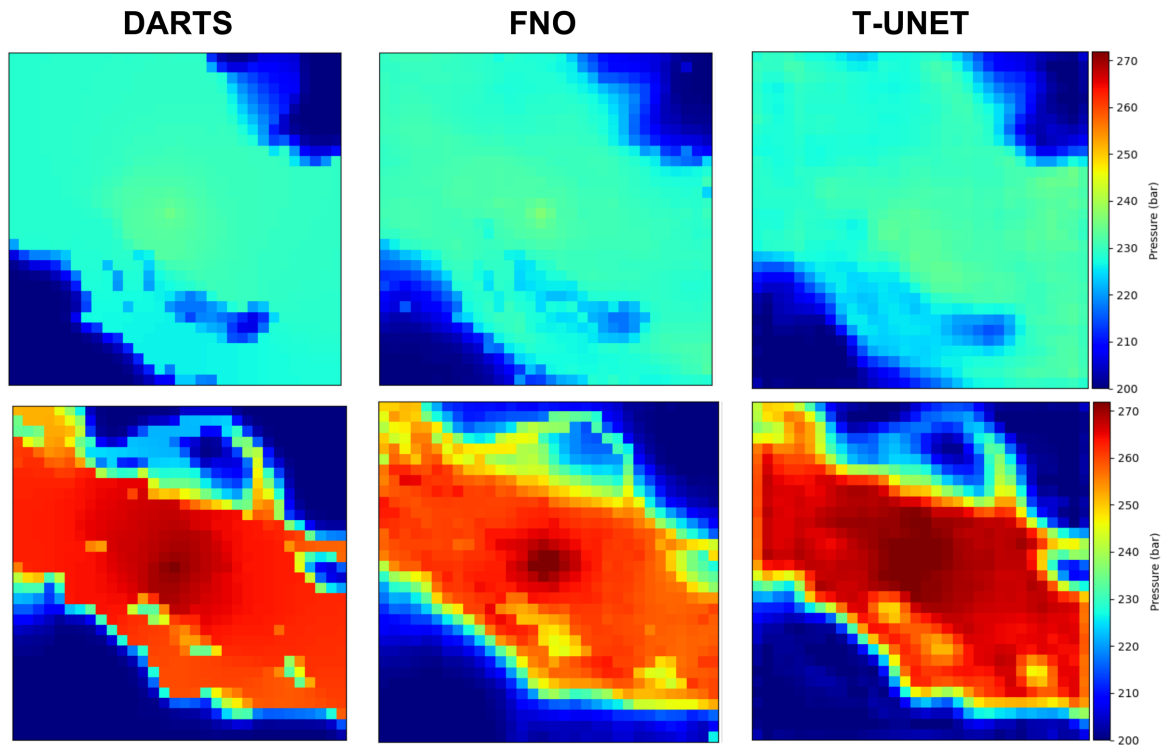
Figure 7 Pressure distributions for a test case using DARTS, FNO, and T-UNET predictions.
