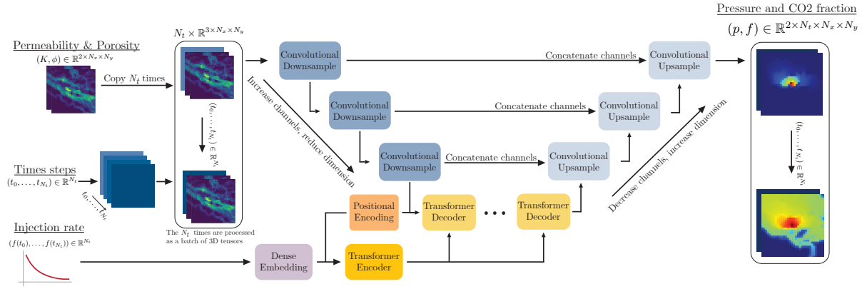
Figure 3 T-UNet setup applied, which combines convolutional layers with transformer modules to optimize the handling of spatial and temporal data (Seabra et al., 2024)
