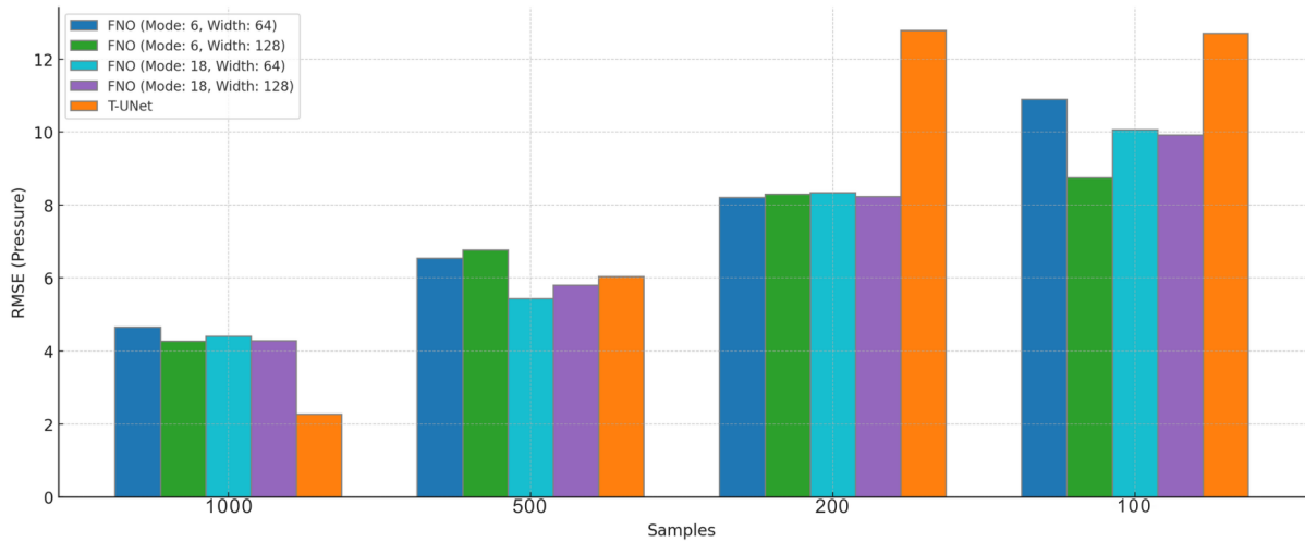
Figure 5 Test RMSE Metrics for pressure (bars)
