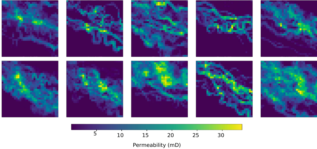
Figure 1 Permeability maps of ten models from the dataset.
