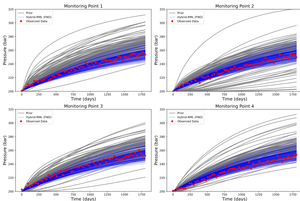
Figure 18 Pressure comparison at each monitoring point for SH-RML using FNO surrogates. Red dots represent a realization of perturbed observed data, highlighting the accuracy of SH-RML in matching observed data closely.
