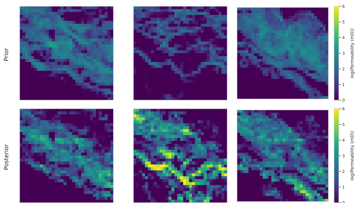
Figure 12 Comparison between prior and posterior permeabilities across three different samples for the ESM DA.
