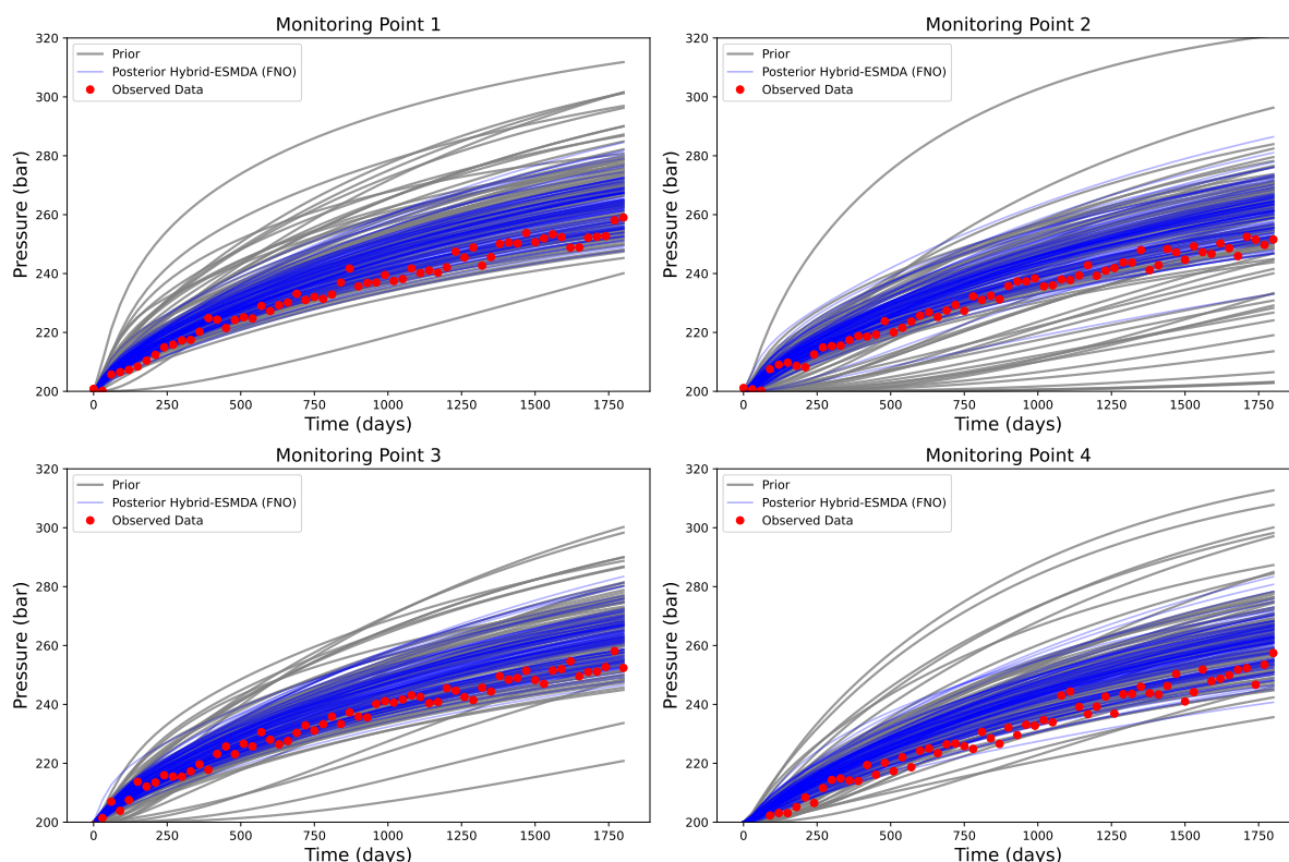
Figure 16 Pressure comparison at monitoring points for Hybrid ESM DA using FNO surrogate. Red dots represent a realization of perturbed observed data.
