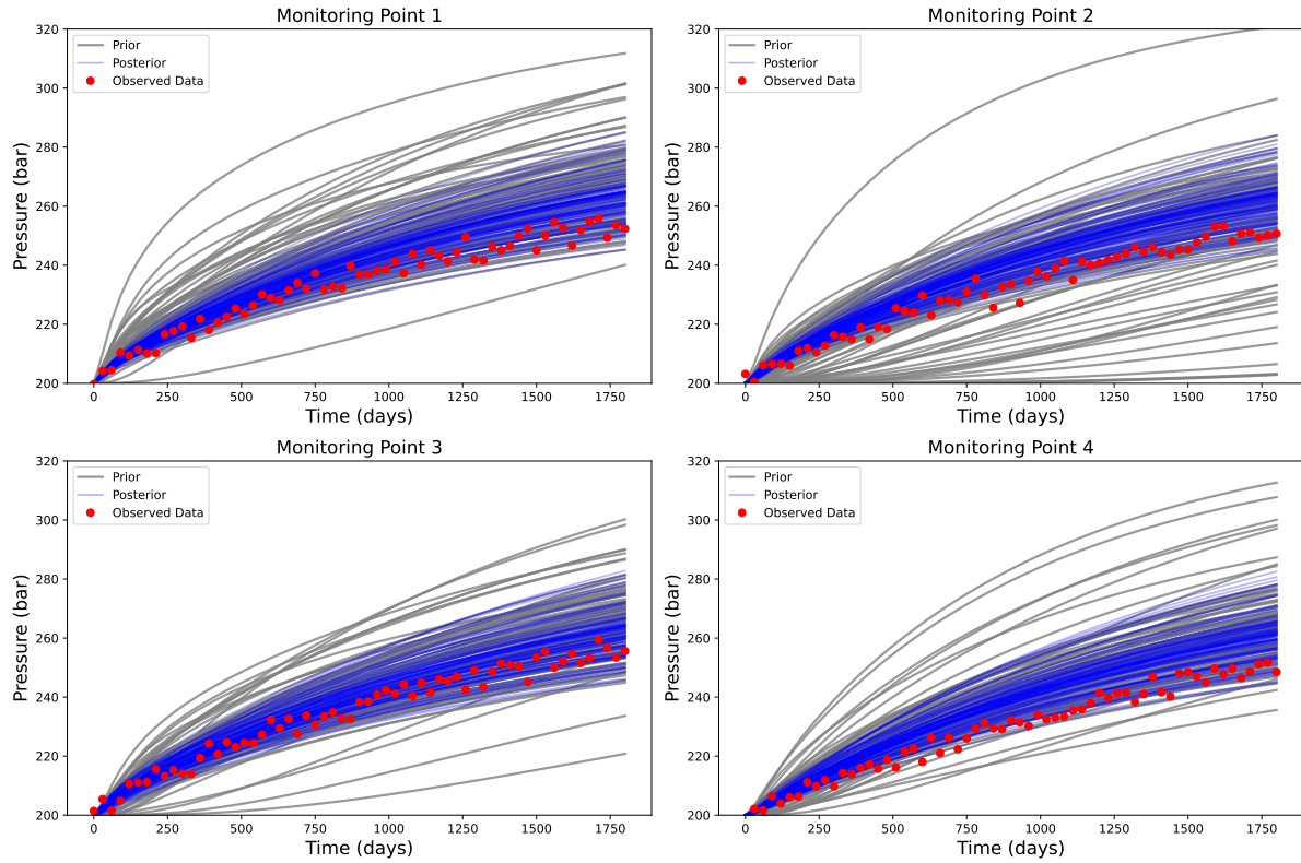
Figure 10 Comparison between the prior, reference model, and posterior pressures at each monitoring point for the ESM DA history matching. Red dots represent a realization of perturbed observed data.
