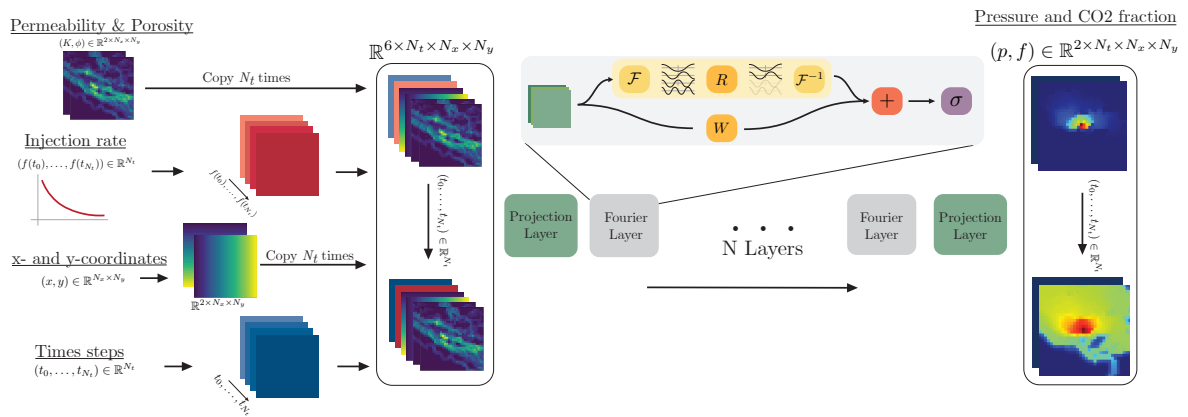
Figure 4 Fourier Neural Operator setup used in our study, which leverages Fourier transformations to efficiently process parametric PDEs. (Seabra et al., 2024)
