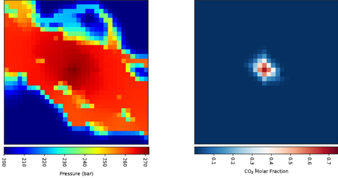
Figure 2 Simulation results using DARTS. Left panel: Pressure distribution (Bar); Right panel: CO 2 molar fraction.
