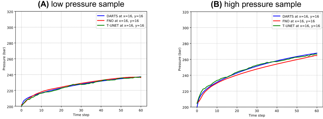
Figure 8 Pressure evolution over time for two different samples using DARTS, FNO, and T-UNet models. (A) Low pressure sample. (B) High pressure sample.
