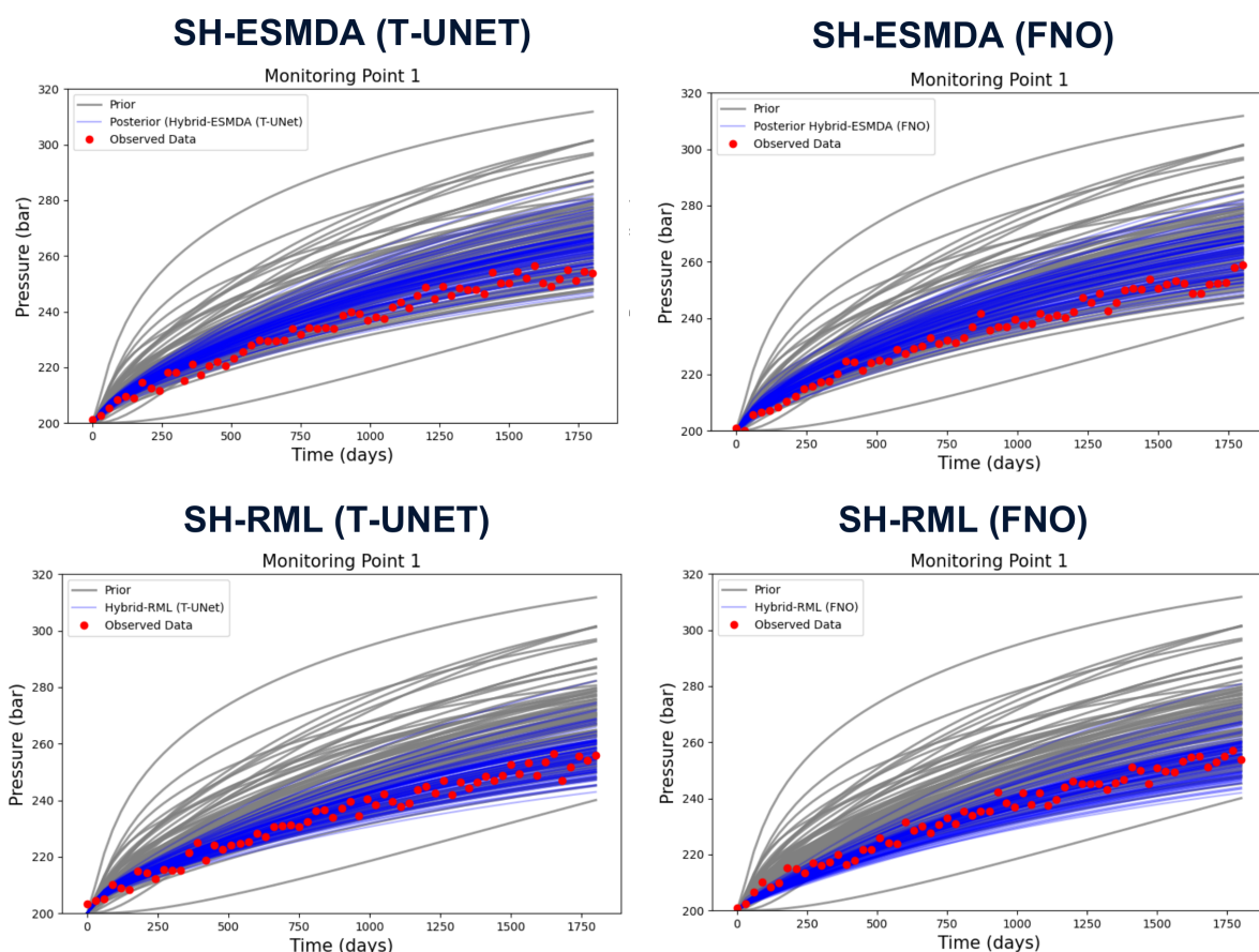
Figure 13 History matching results at Monitoring Point 1 for SH-ESMDA and SH-RML methods using both T-UNet and FNO surrogates.
