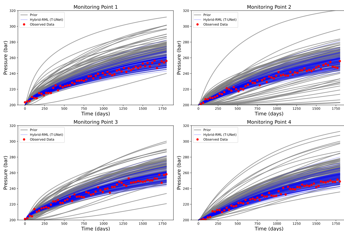
Figure 19 Comparison of monitoring pressure results using T-UNet surrogates in SH-RML. This figure illustrates the surrogate's capability to adhere to the accuracy requirements while enabling faster computational times.
