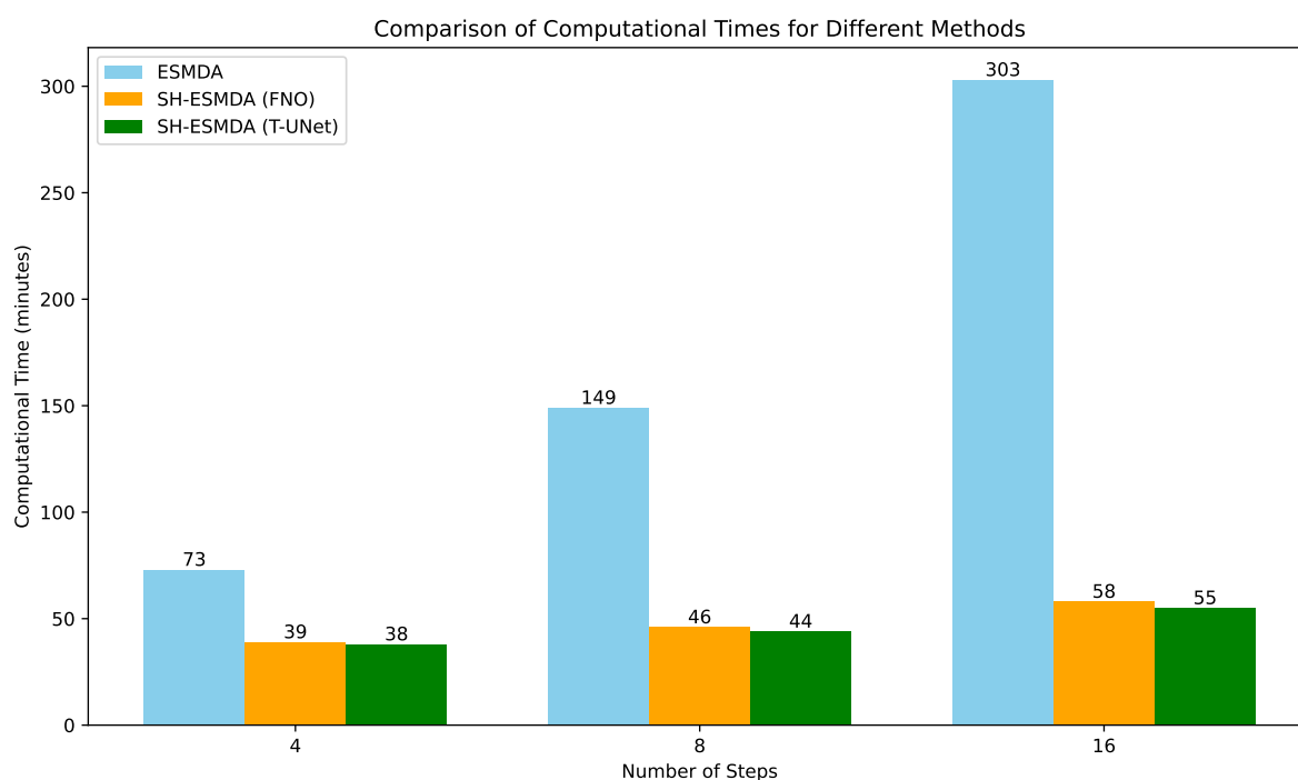
Figure 14 Comparison of computational times for ESM DA and SH-ESMDA methods using FNO and T-UNet surrogates. The bar chart shows the runtime in minutes for different numbers of assimilation steps, demonstrating the significant time savings achieved by the hybrid methods.
