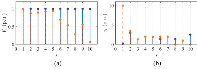
Fig. 7. Results of (14) and (15) achieved by different initial conditions: (a) voltage magnitudes and (b) power injections. The blue and the orange stems represent the two equilibria of the noncooperative game, corresponding to the white and orange area of Fig. 6, respectively.
