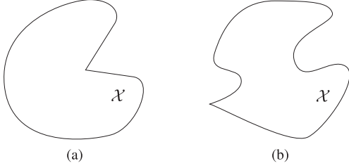
Fig. 2. Example of (a) nonproximally smooth set and of (b) proximally smooth set.
