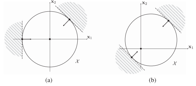
Fig. 1. Illustration of LGNE points in (a) Example 1 and (b) Example 2.
