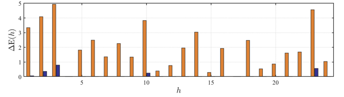
Fig. 9. Power mismatch \Delta E(h) of the microgrid over the control horizon achieved by the standard OPF (orange bars) and the noncooperative approach (blue bars).
