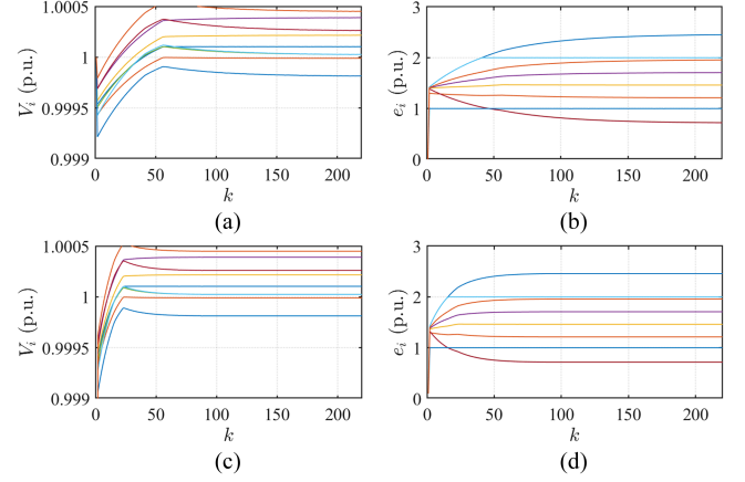
Fig. 8. Convergence of Algorithms (14) and (15) with the flat-start approach: (a) voltage magnitudes with Algorithm (14), (b) power injections with Algorithm (14), (c) voltage magnitudes with Algorithm (15), and (d) power injections with Algorithm (15).
