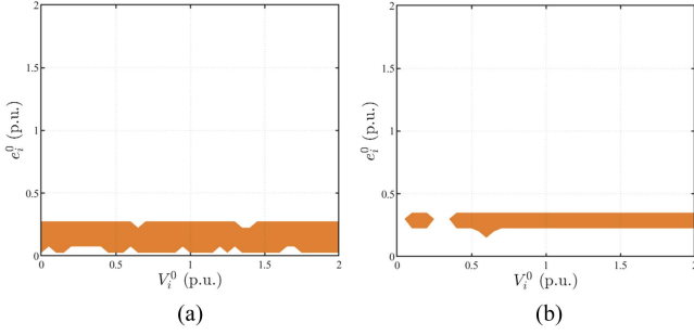
Fig. 6. Convergence regions with respect to the initial voltage magnitude and power injection (both equal for all buses): (a) Algorithm (14) and (b) Algorithm (15). The white and the orange regions correspond to the two equilibria of the noncooperative game.
