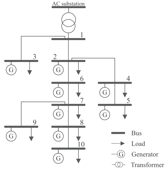
Fig. 5. Scheme of the simulated DC microgrid.
