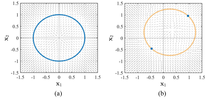
Fig. 3. Pseudophase plane plots for (a) Example 1 and (b) Example 2, where we indicate the vLGNE in blue.
