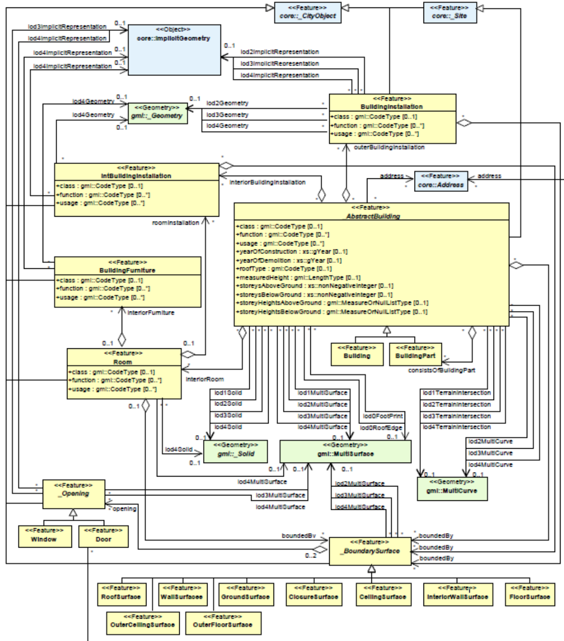
Figure 6- UML diagram of CityGML's building model (Gröger et al., 2012)
