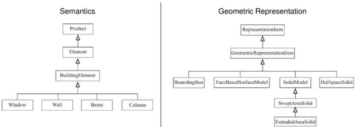
Figure 12- Separation of geometry and semantics in the IFC data model
