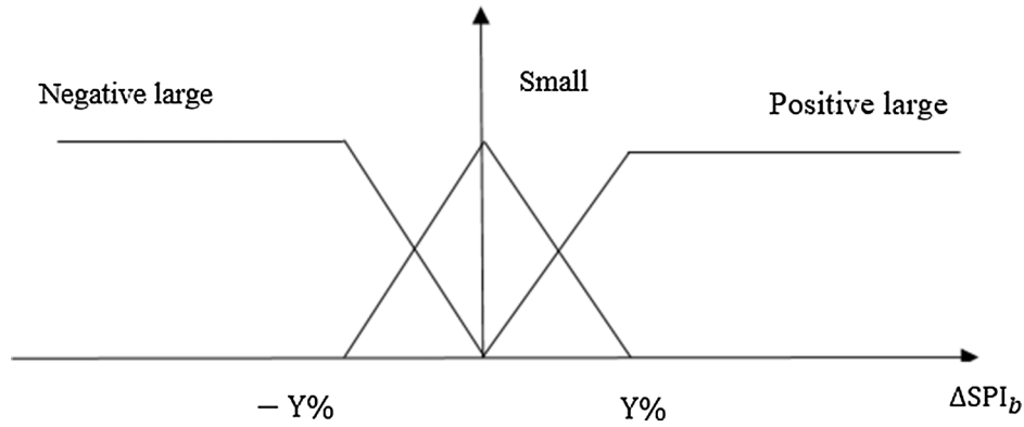
Fig. 9. Membership function of three different values of \Delta SPI_b .
