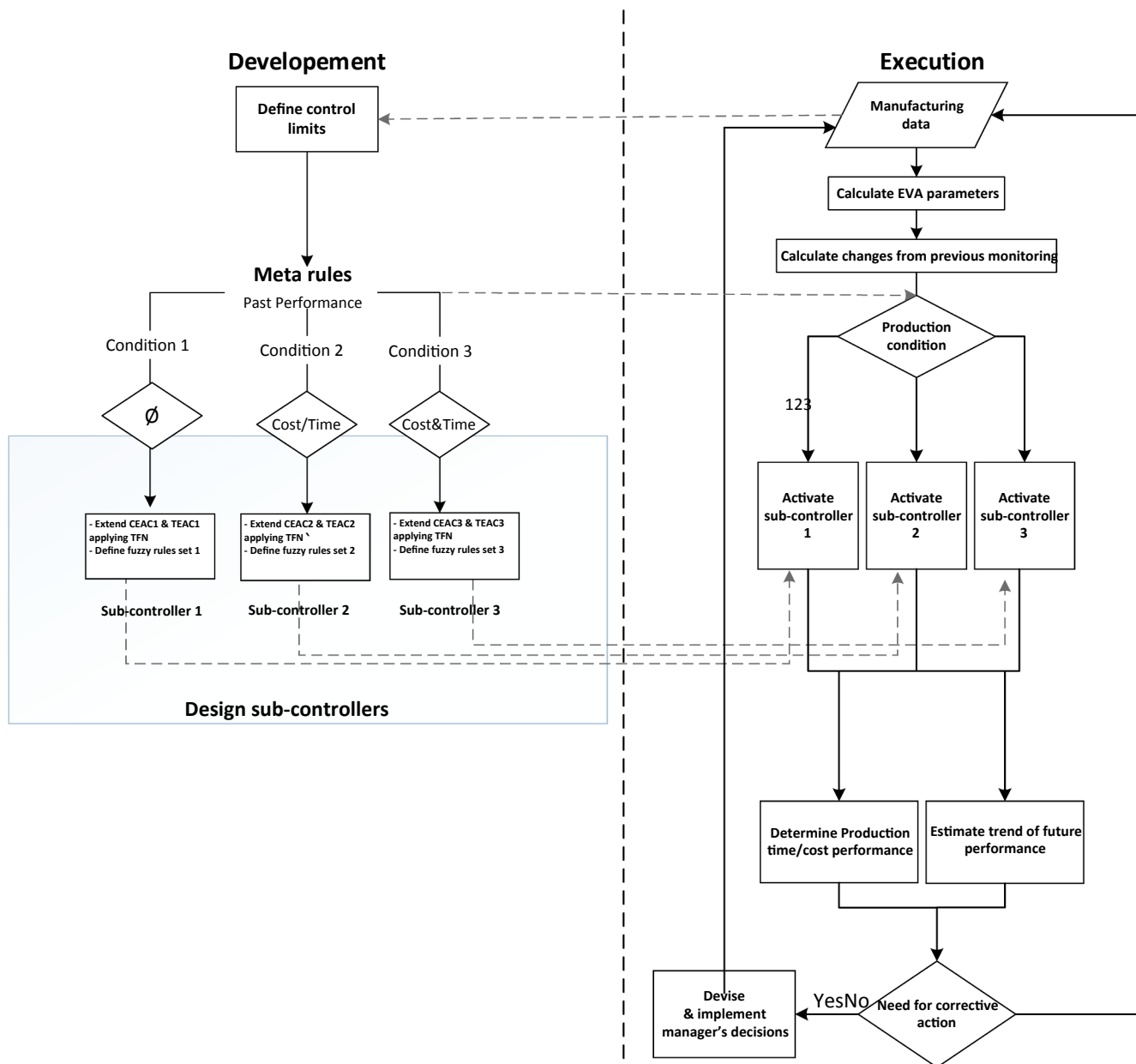
Fig. 3. Proposed methodology.
