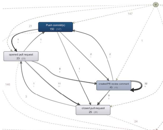
Fig. 1. Excerpt from the Apache Camel process map.
