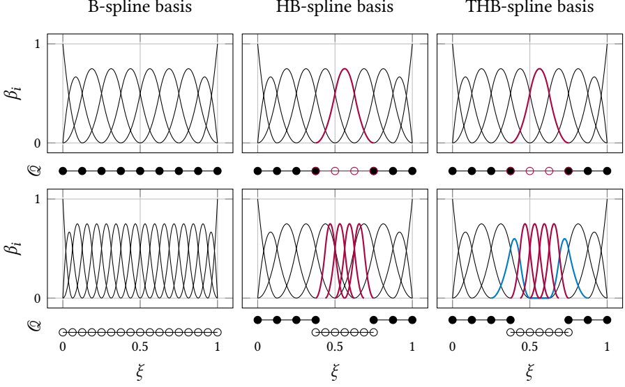
Figure 2.6: Principles of refinement for different spline bases. The top plots represent the basis on level 0, optionally with (to be) refined functions given in red color. The bottom plots illustrate the refined bases: uniform refinement (left), hence level 1; HB-refinement (middle); and THB-refinement (right) with truncated basis functions in blue color. The line \mathcal{Q} represents the elements of the basis. The unrefined unique knot vector in all cases is \Xi = \{0, 1/8, 2/8, \dots, 7/8, 1\} , and the degree of the basis is 2. All bases are generated with the open-source IGA library G+Smo [294].
