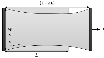
Figure 3.8: Modelling geometry for the uniaxially loaded restrained sheet. The sheet has length L and width W . The strain of the sheet due to load P is denoted by \varepsilon .
