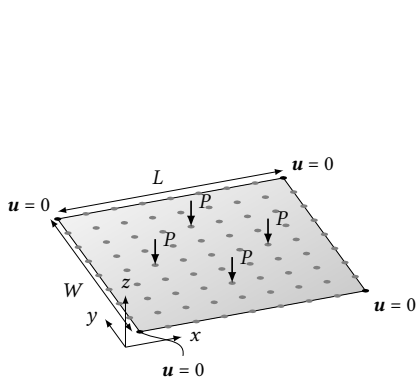
(a) Problem setup for the optimised square plate. The vertical loads have magnitude P and the corners of the plate have restrained displacements u = 0 . The geometry has 9 \times 9 control points, of which the grey ones are degrees of freedom for the shape optimisation and the black ones are fixed.
