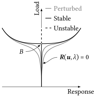
(a) Effect of initial perturbations to avoid passing bifurcation points.
