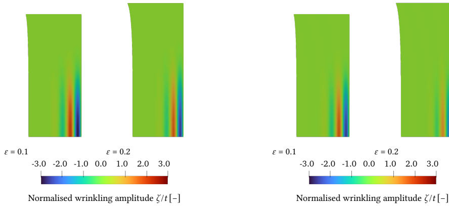
(b) Contour plot of out-of-plane displacements w for different strains \varepsilon for the MR model.
