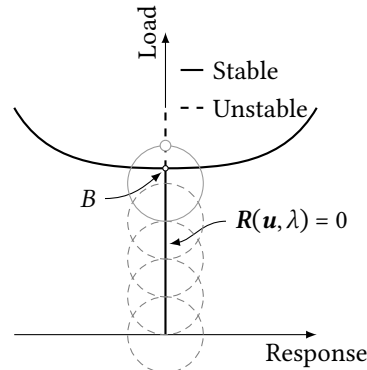
(b) Arc length method applied on pitch-fork bifurcation, without perturbations.
