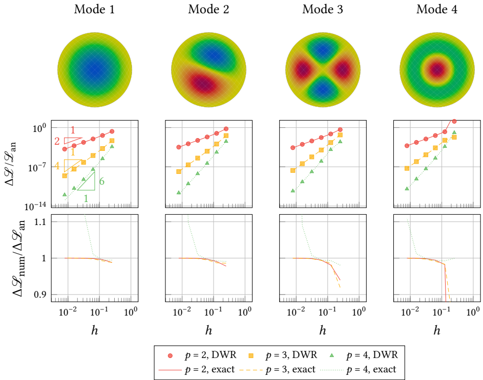
Figure 5.9: Modal analysis of a circular plate. The top row provides the mode shapes from mode 1 up to 4. The mid row provides \Delta \mathcal{L} against the uniform mesh size h , and the bottom row provides the efficiency of the error estimators against the mesh size h . The markers represent error estimates computed via the DWR method, and the lines represent the exact error, i.e. the error of the numerical solution with respect to the analytical solution. The eigenfrequencies for modes 1 up to 4 are, respectively, \omega_1 = 9.56 \cdot 10^{-4} [Hz], \omega_2 = 4.14 \cdot 10^{-3} [Hz], \omega_3 = 1.11 \cdot 10^{-2} [Hz] and \omega_4 = 1.45 \cdot 10^{-2} [Hz].
