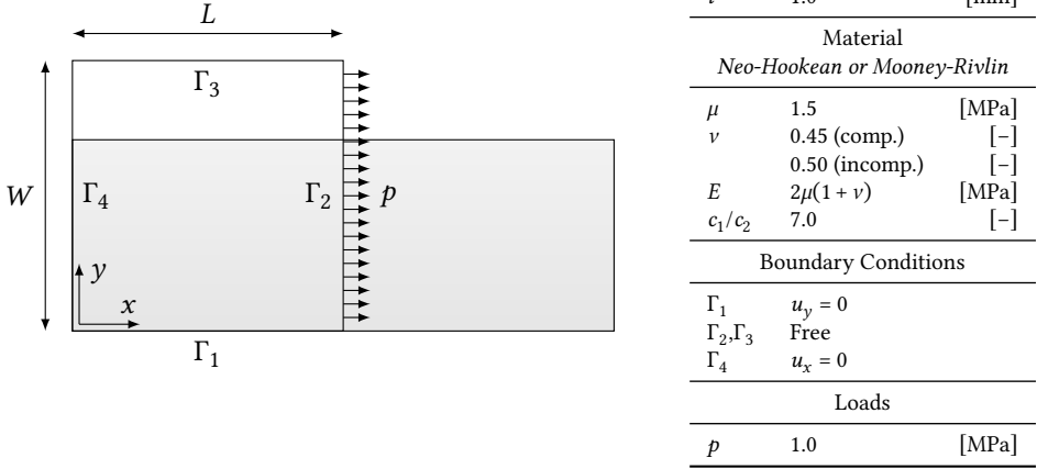
Figure 4.1: Set-up for the uniaxial tension benchmark problem. In the figure on the left, the filled geometry represents the deformed configuration, and the dashed line indicates the undeformed geometry. The load p indicates a line load acting on the undeformed geometry. The table on the right provides the parameter values for the specific benchmark problem for Neo-Hookean (NH) and Mooney-Rivlin (MR) materials.
