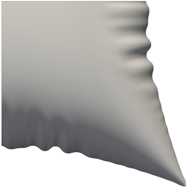
(a) Top view of a quarter of the inflated square membrane for 1024 elements with degree p = 3 using the KL shell.
