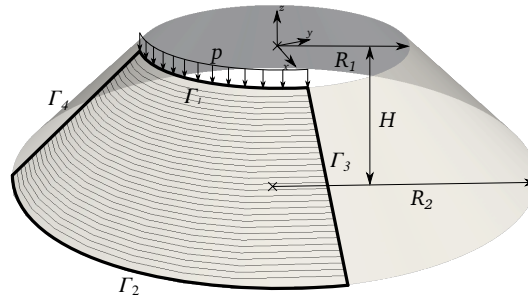
Figure 3.5: Geometry of the collapsing truncated conical shell with top and bottom radii R_1 and R_2 , height H and a line load p on \Gamma_1 . On boundaries \Gamma_3 and \Gamma_4 , symmetry conditions are applied. Boundary \Gamma_1 is either constrained in x and y directions (fixed radius) or free (variable radius). Boundary \Gamma_2 is constrained. The geometry is modelled using 32 quadratic elements over the height.
