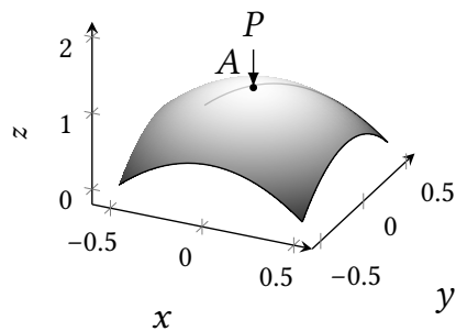
Figure 7.11: Elliptic paraboloid shell geometry with coordinates \mathbf{r}(\xi_1, \xi_2) = [\xi_1 \quad \xi_2 \quad 1 - 2(\xi_1^2 + \xi_2^2)]^T , \xi_1, \xi_2 \in [-1/2, 1/2] . On the corners of the domain, the vertical displacements are set to zero u_z = 0 and one corner is fixed in-plane as well. Furthermore, a point load with a magnitude P = 10^8 t is applied in the middle of the geometry.
