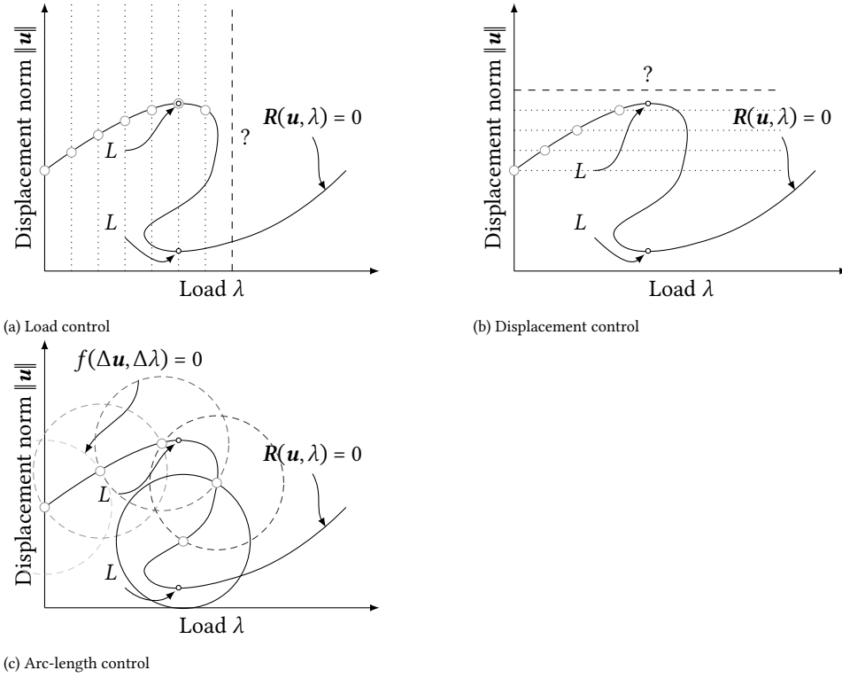
Figure 2.13: Load (top left), displacement (top right), and arc-length control (bottom left) for structural analysis problems. The question mark (?) indicates the iteration where load and displacement control encounter a point where the next obtained point is typically difficult to find. Limit points are indicated with L .
