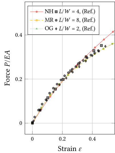
(b) Benchmarking results for comparison with [427] (Ref.). Experimental results are depicted by markers for different aspect ratios L/W of the sheet. Numerical results from [427] are not included since they are indistinguishable from the present MR results.
