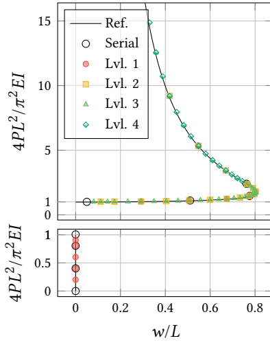
(a) Non-dimensional out-of-plane displacement of the beam with respect to the non-dimensional buckling load.
