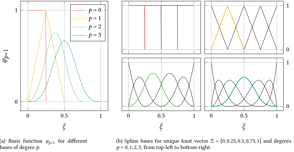
Figure 2.2: B-spline basis functions \varphi_i on the domain \xi \in [0, 1] with unique knot vector \Xi = \{0, 0.25, 0.5, 0.75, 1\} for degrees p = 0, 1, 2, 3 . Figure 2.2a provides a canonical representation of the basis functions, i.e., the functions \varphi_{p+1} are depicted. Figure 2.2b provides all functions of each basis, with the coloured function being the one represented in figure 2.2a.
