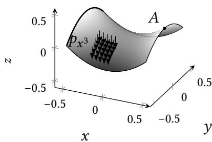
Figure 7.10: Hyperbolic paraboloid shell geometry with coordinates \mathbf{r}(\xi_1, \xi_2) = [\xi_1 \quad \xi_2 \quad \xi_1^2 - \xi_2^2]^T , \xi_1, \xi_2 \in [-1/2, 1/2] . The left-edge of the hyperbolic paraboloid is clamped, i.e., the displacements and rotations are zero ( \mathbf{u} = 0 and \frac{\partial u_z}{\partial x} = 0 ).
