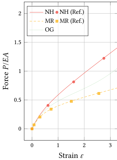
(a) Benchmarking results comparing to the reference results (Ref.) from [480], which are obtained numerically.
