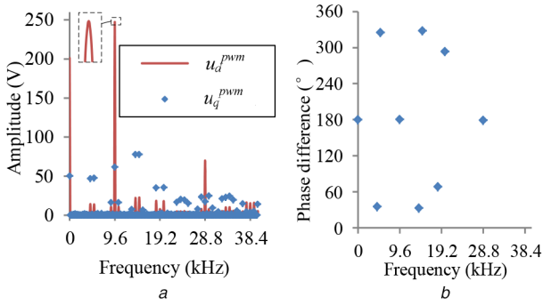
Fig. 5 PWM voltage spectra in the dq reference frame (a) Amplitudes, (b) Phase difference between each preponderant component in u_d^{pwm} and u_q^{pwm}
