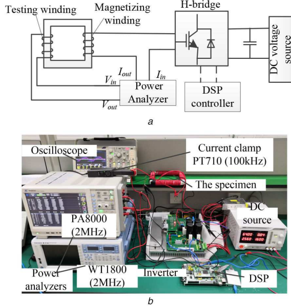
Fig. 15 Measuring iron loss under PWM VSI supply (a) Diagram, (b) Picture
