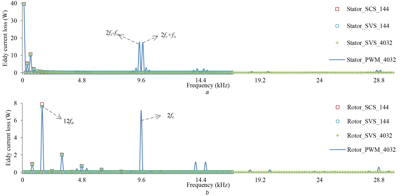
Fig. 2 Spectra of eddy current loss in the ESSs at operating condition A2 where f_o is 400/3 Hz and f_c is 4800 Hz
