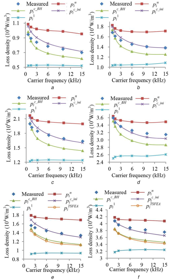
Fig. 19 Comparison of the iron loss densities calculated with different methods under PWM VSI supply
