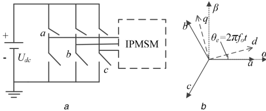
Fig. 3 Diagram of the inverter-motor system
