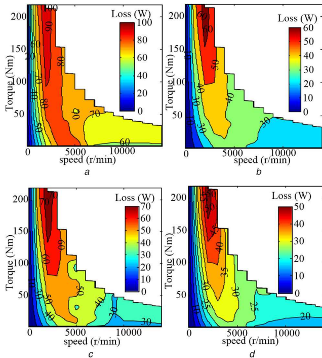
Fig. 12 CHIL maps over the entire operating range
