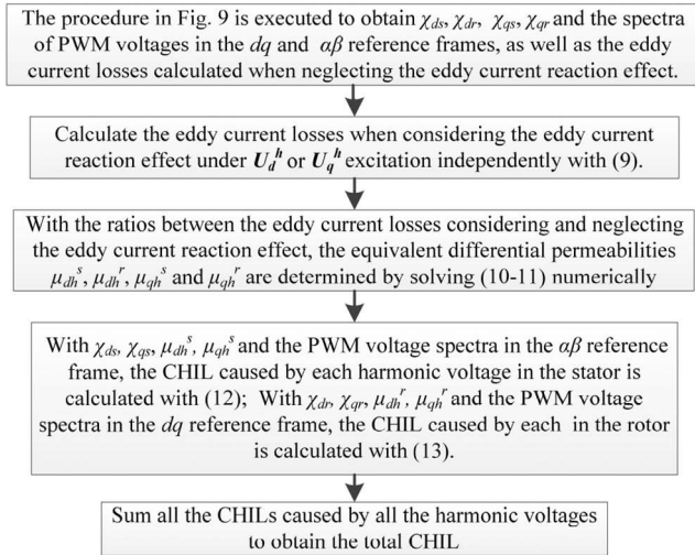
Fig. 11 Calculation of the total CHIL at a given working condition when considering the eddy current reaction effect
