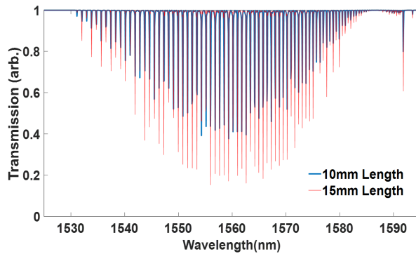
Figure 7: Effect of TFBG length on transmission spectrum
