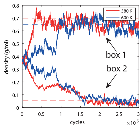
Figure 4. GEMC simulation of \text{H}_2\text{O} at 580 and 600 K. The solid lines represent the densities of the two boxes simulated by the GEMC–ReaxFF, with red at 580 K and blue at 600 K. The dashed lines represent experimental coexistence data. 33
