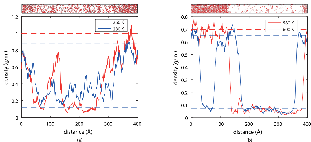
Figure 3. Average density distributions of the simulation boxes of (a) \text{CO}_2 and (b) \text{H}_2\text{O} after MD simulation. The red solid and dashed lines are the simulation results and the experimental coexistence densities 32,33 for the lower temperatures, respectively. The blue solid and dashed lines are the simulation results and the experimental coexistence densities for the higher temperatures, respectively. The top boxes are representations of the final configurations at 280 and 580 K for \text{CO}_2 and \text{H}_2\text{O} , respectively.
