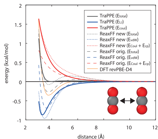
Figure 2. Comparison of different energy contributions regarding the dissociation of two parallel CO 2 molecules. The gray lines represent the total energy. The blue line represents the Lennard-Jones energy contribution for the TraPPE force field and the van der Waals energy for the ReaxFF force fields. The red line represents the Coulomb energy contribution for the TraPPE force field and the summation of the Coulomb and polarization energy in the ReaxFF force fields. The orange line represents the DFT-D reference.
