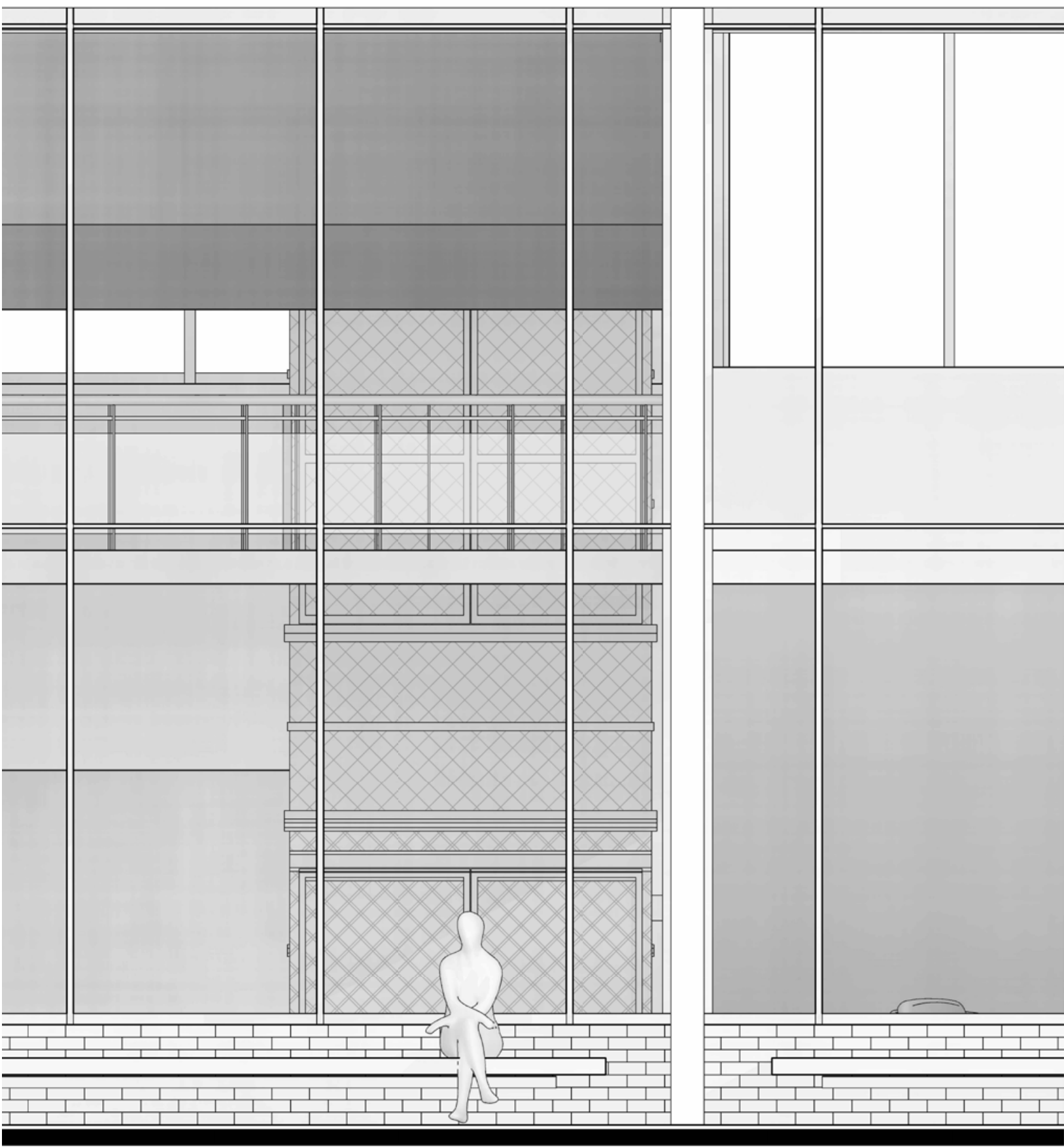
Fragment elevation 1:30
