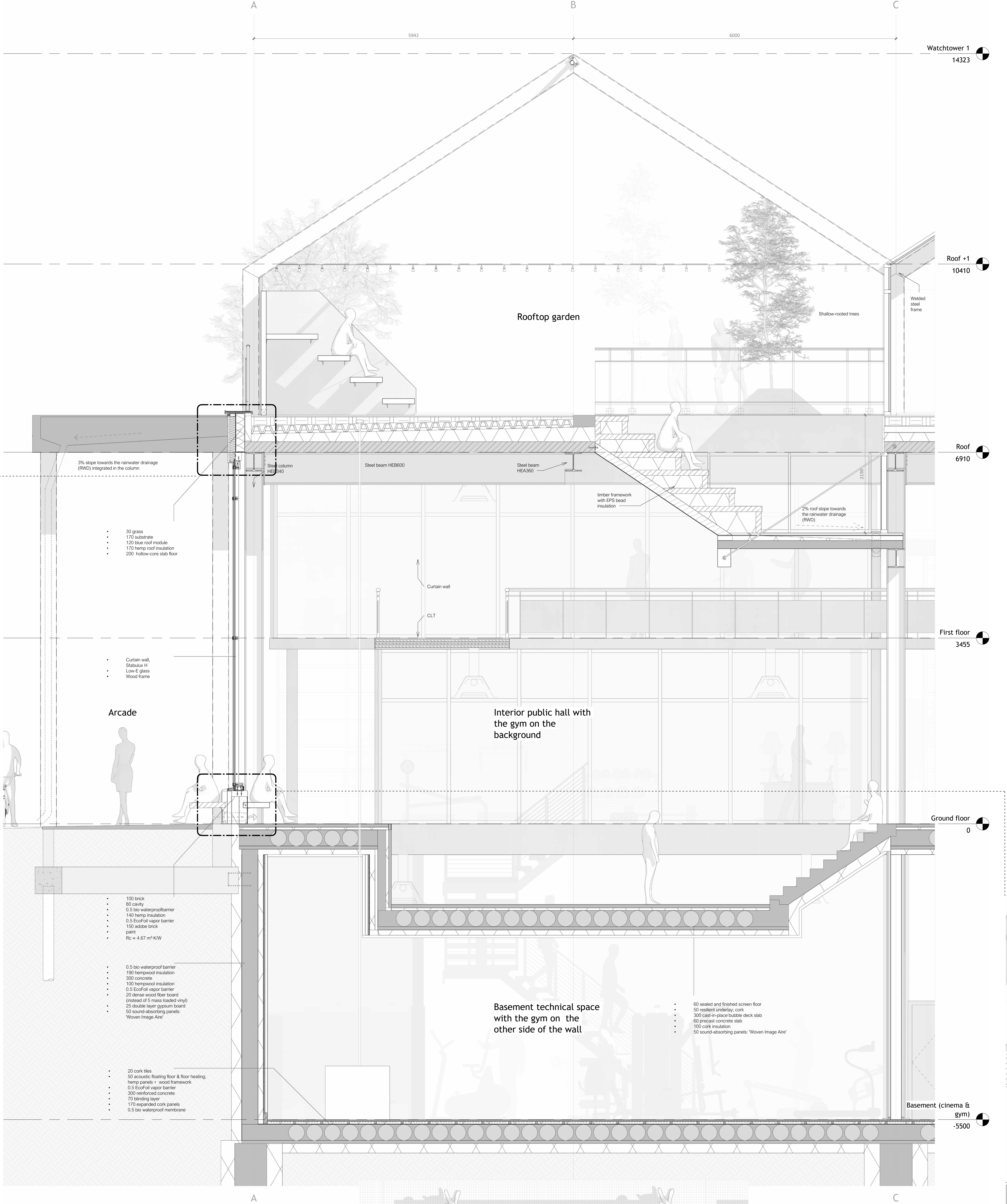
Fragment section 1:30
