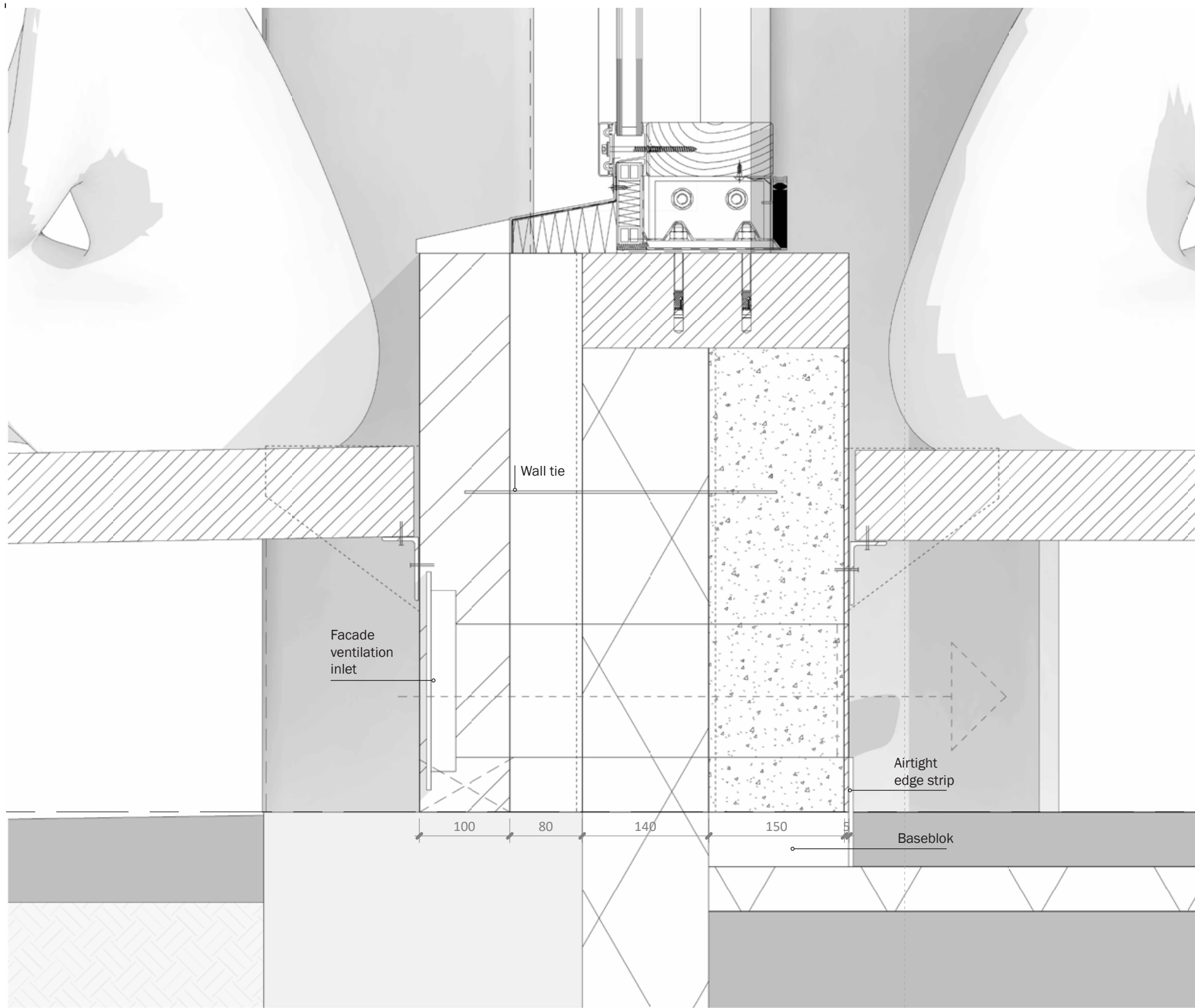
Detail 1:5
