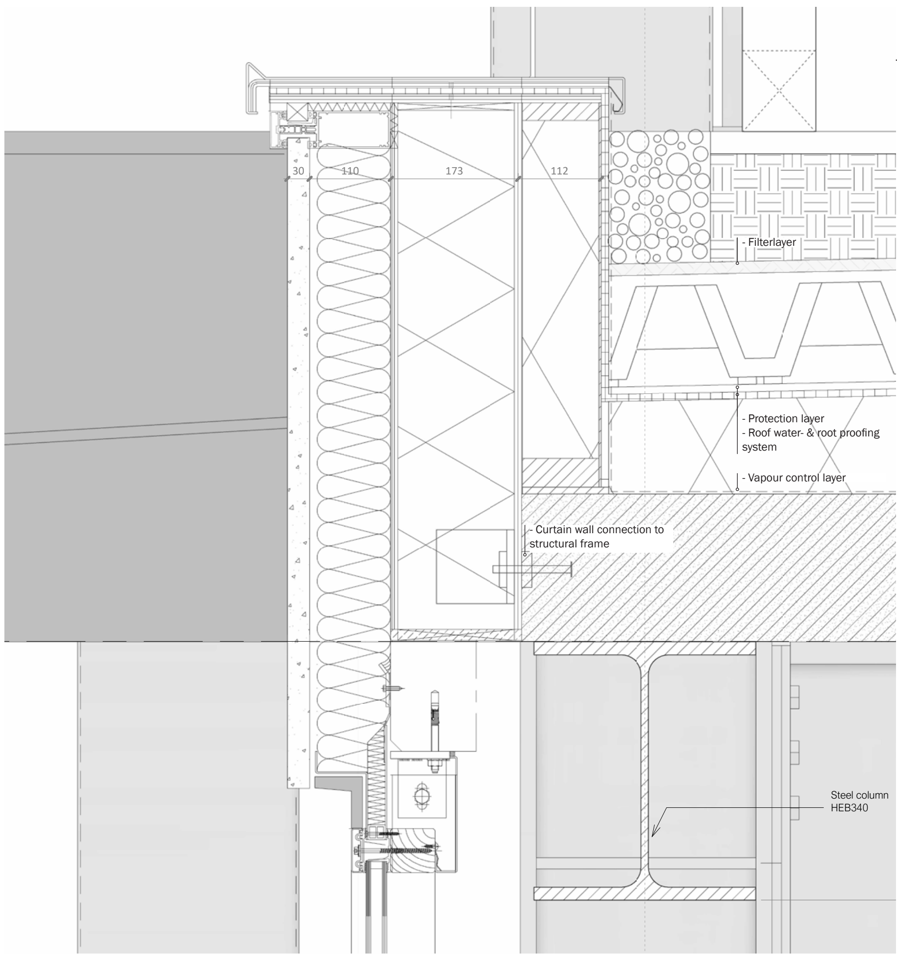
Detail 1:5
