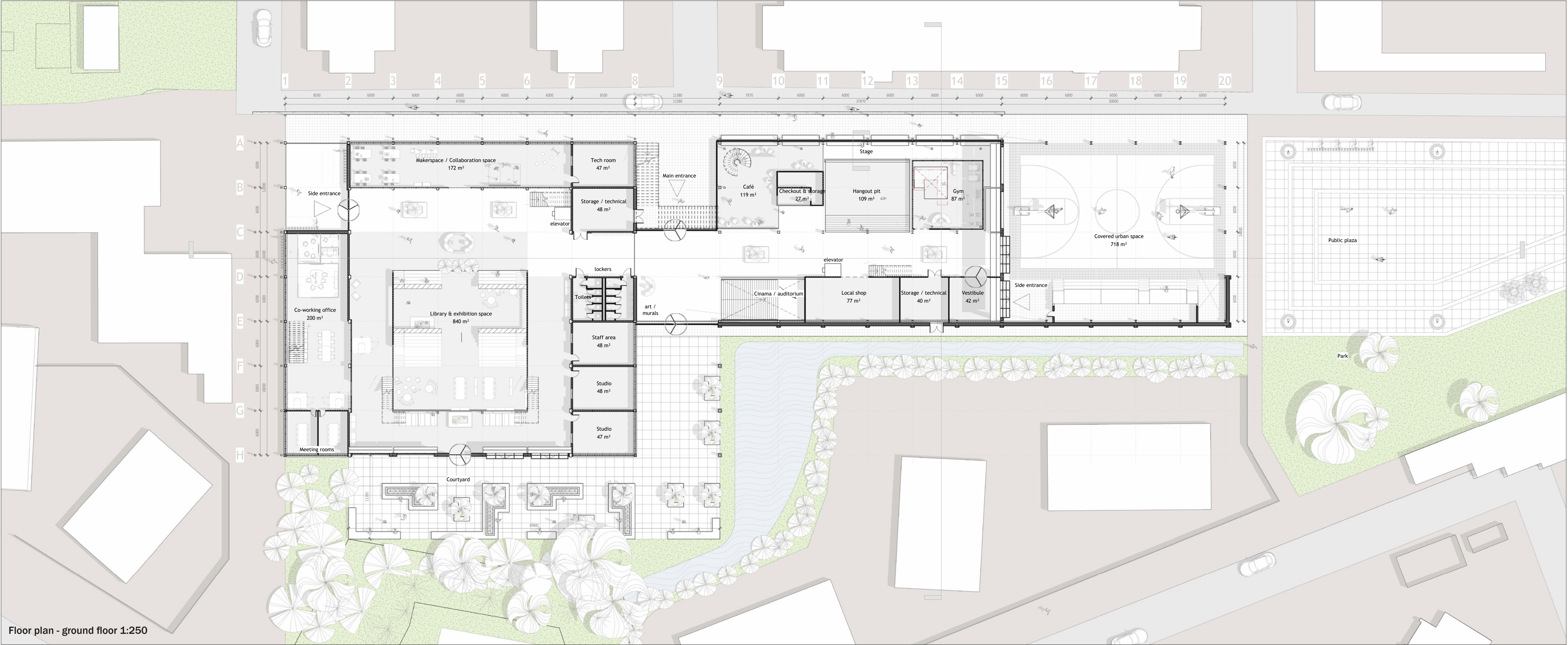
Floor plan - ground floor 1:250
