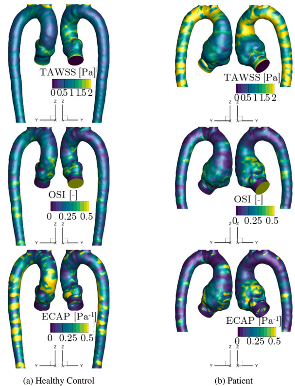
Fig. 4. Time-averaged wall shear stress (TAWSS [Pa]), Oscillatory Shear Index (OSI [-]), and Endothelial Cell Activation Potential (ECAP [ Pa^{-1} ]) for healthy control (a) and patient (b) in the lumen-only approximation of aorta.
