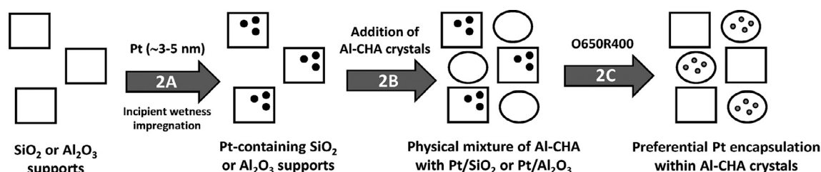
Scheme 1 Atom-trapping methodology when the Al-CHA is mixed with a Pt-containing \text{SiO}_2 or \text{Al}_2\text{O}_3 support. Reproduced with permission from Moliner, M.; Gabay, J.; Klier, C.; Serna, P.; Corma, A., Trapping of Metal Atoms and Metal Clusters by Chabazite under Severe Redox Stress. ACS Catal. 2018 , 8(10), 9520–9528. Copyright 2018, American Chemical Society.
