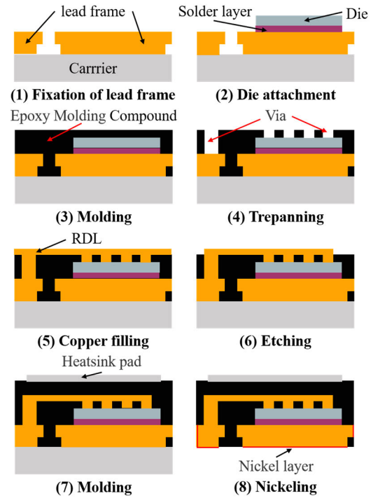
Fig. 2. Flowchart of SiC MOSFET FOPLP packaging process.
