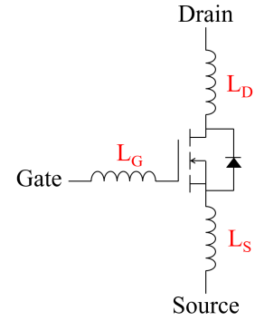
Fig. 4. Equivalent circuit diagram of the SiC MOSFET.
