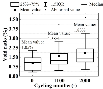
Fig. 13. Void ratios at 0, 1100, and 2000 cycles.
