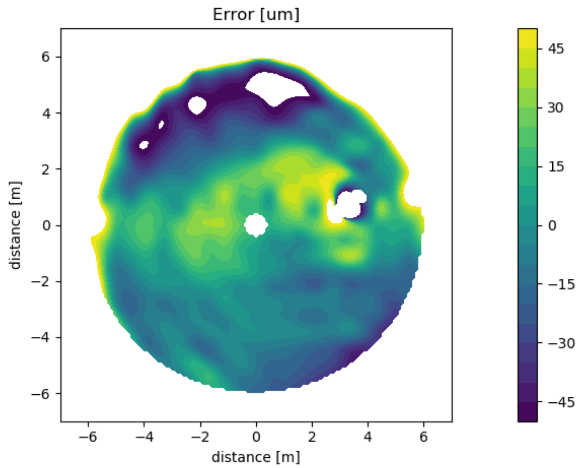
Fig. 10. Equivalent mirror surface accuracy calculated from beam under analysis in Fig. 6. It is a representation in which the wavefront error is presented as generated by a single defective mirror.
