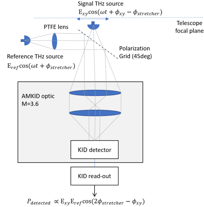
Fig. 2. Schematic of the experimental setup. Reference and signal sources are generated at the instrument focal plane. Both signals propagate through the optics and are detected by the KID detector.
