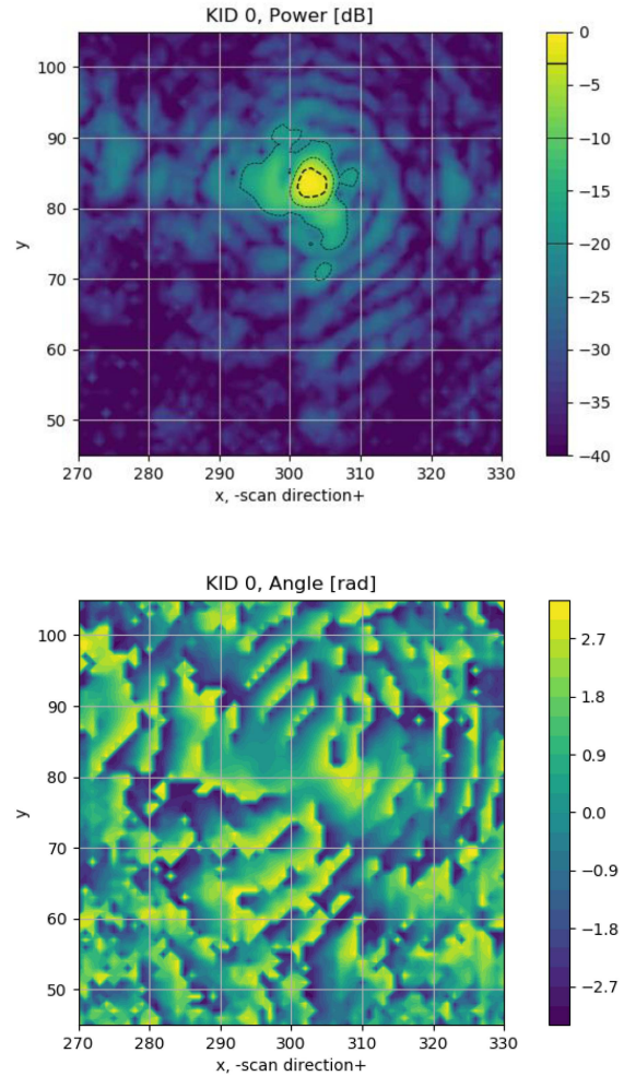
Fig. 11. Phase (bottom) and amplitude (top) beam map of a specific detector in the HFA. Measurement done at 850 GHz.
