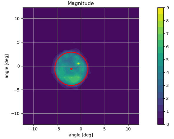
Fig. 8. Magnitude of E-Field distribution at telescope secondary mirror (arbitrary units). The red circle shows the subtended secondary position as seen from the measurement plane.
