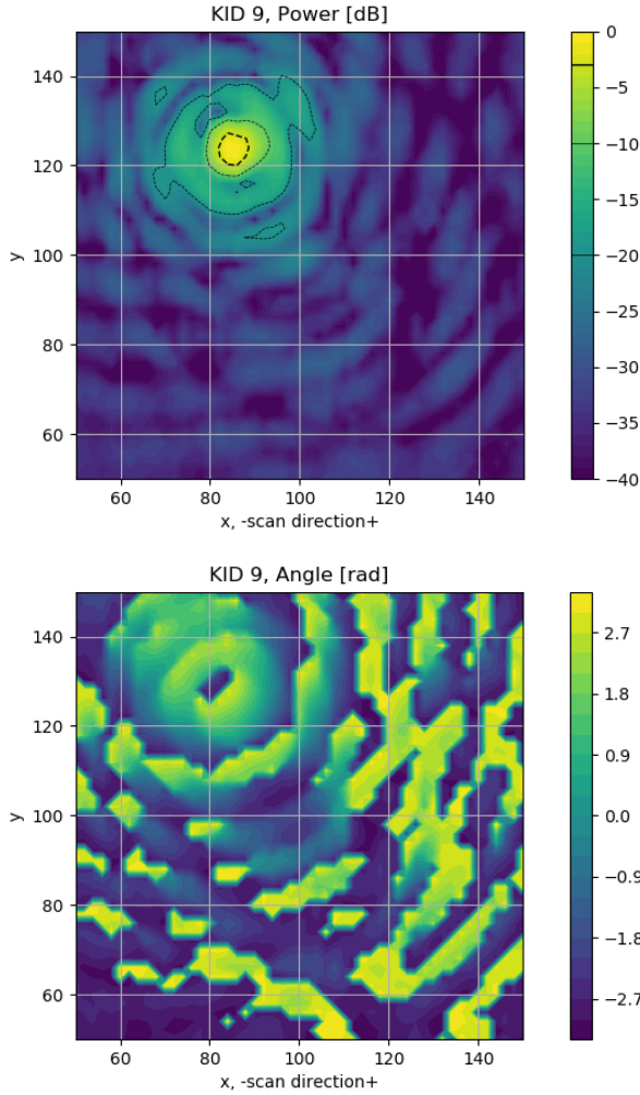
Fig. 7. Amplitude (top) and phase (bottom) beam map of a specific detector in the sampled area. Along with the showed pattern around 30 more good quality maps ( \text{SNR} > 20 \text{ dB} ) are obtained in the scanned area.
