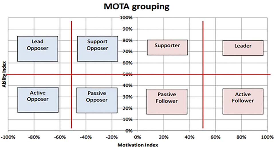
Figure 3. MOTA mapping.
