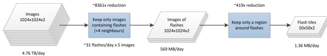
Fig. 9. LUMIO payload data processing strategy.
