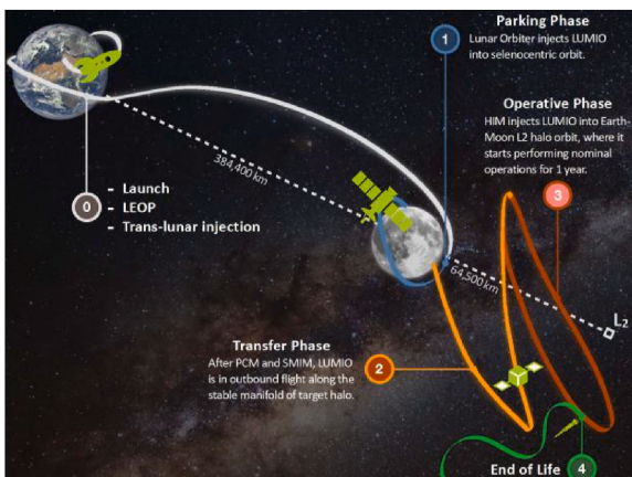
Fig. 2. LUMIO mission concept and phases.
