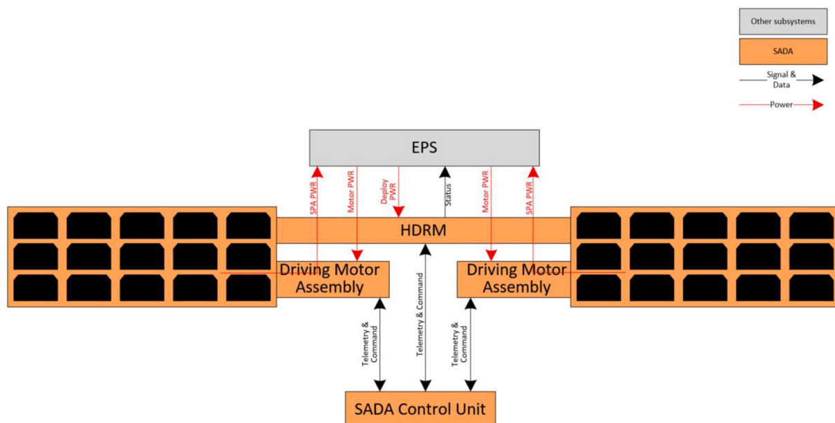
Fig. 10. LUMIO high-level solar array architecture.
