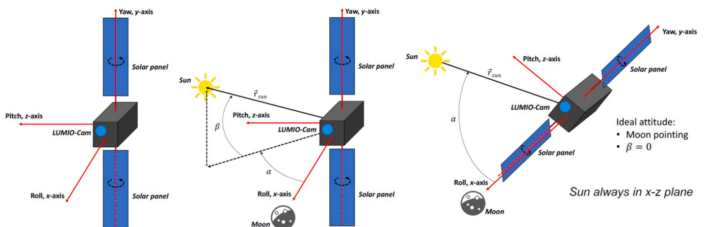
Fig. 8. LUMIO spacecraft pointing strategy.
