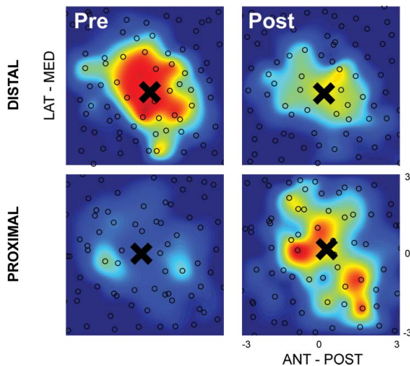
FIGURE 7. Individual examples of TMS maps before and after learning for both a distal muscle (top row) and a proximal muscle (bottom row). In this case, the top row represents a negative responder (decrease in map area), while the bottom row represents a positive responder following the visuomotor tracking learning task (increase in map area). All black open circles represent one stimulation and the black cross (X) highlights the COG. Red indicates big MEPs, in contrast to small MEPs which are indicated by blue.
