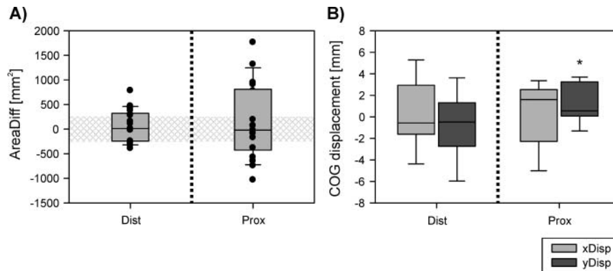
FIGURE 8. Effect of training a visuomotor tracking learning task with a distal (FDI) and proximal (BB) muscle on TMS map area and COG. (A) Change in map area ( \Delta\text{area} = \text{area}_{\text{POST}} - \text{area}_{\text{PRE}} ) was not significantly different from 0 for either muscle; however, there are great interindividual differences with some participants showing an increase, decrease, or no change in map area (black dots). Based on baseline variability of the map area, all participants with a change in map area within the range as marked by the shaded rectangle were classified as nonresponders. (B) No change was found in x -coordinate of the COG for any muscle, while a significant displacement of the y -coordinate for the proximal muscle was found but not the distal muscle.
