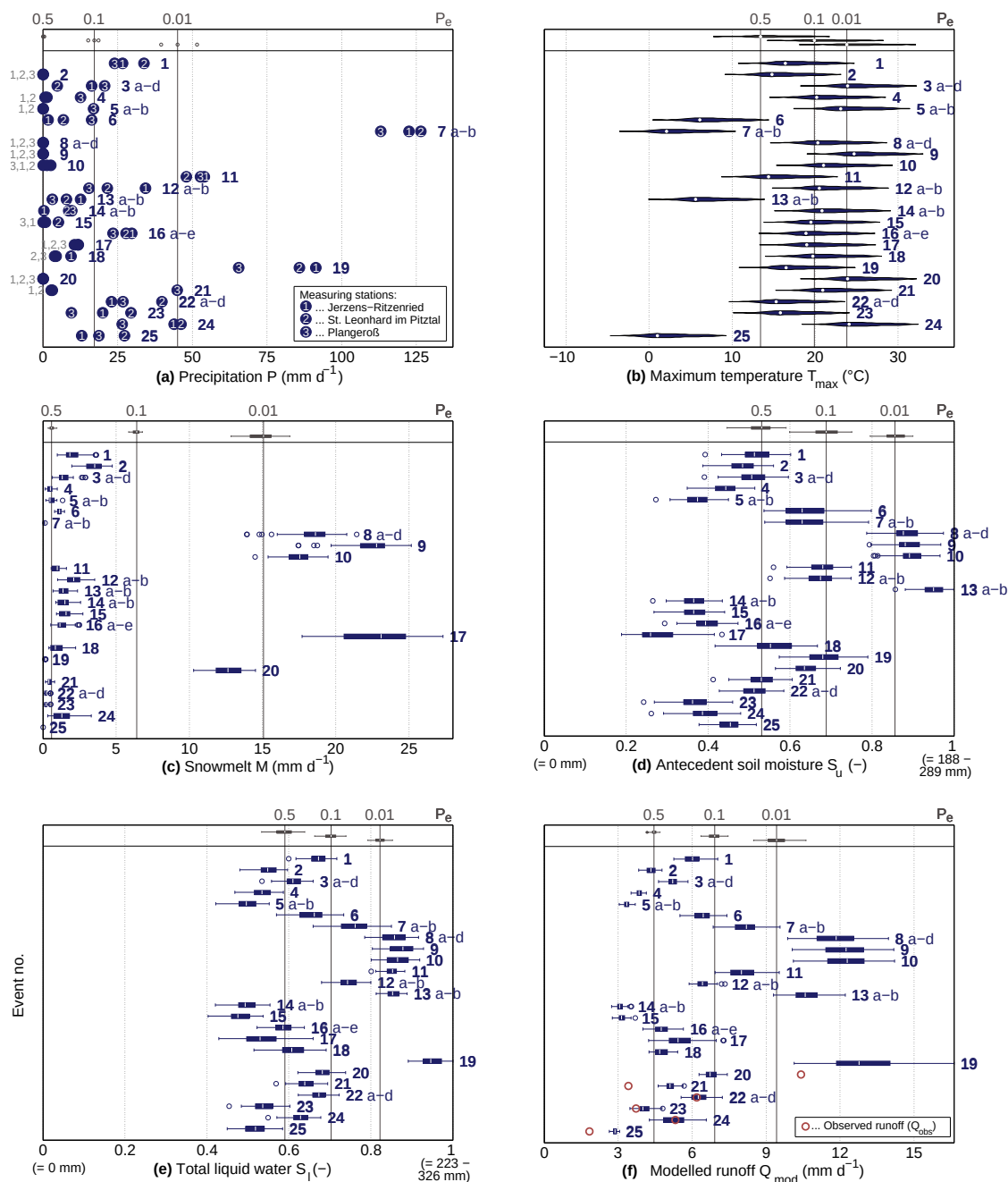
Figure 6. Plots of relevant system variables: (a) precipitation P elevation adjusted for mean catchment elevation, (b) maximum temperature T_{\max} for all catchment elevations (blue bars) and mean elevation (white dots), and (c–f) modelled snowmelt M , antecedent soil moisture S_u , total liquid water availability S_l , and runoff Q_{\text{mod}} (and, where available, Q_{\text{obs}} ). Boxplots comprise all behavioural models. For event numbering see Table 2. P_e is the observed/modelled probability of exceedance (i.e. marginal distribution; see Sect. 3.2) for a specific variable considering all days between 15 May and 15 October within the study period 1953–2012.
