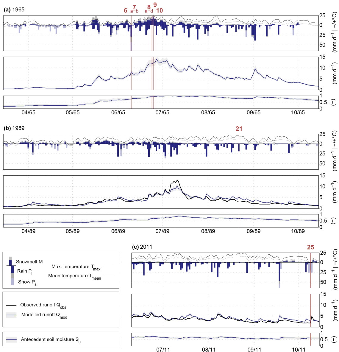
Figure 5. Observed daily streamflow Q_{\text{obs}} (black solid line), daily mean temperature T_{\text{mean}} at mean elevation (grey solid line) and maximum temperature T_{\text{max}} at mean elevation (black solid line) as well as, based on observed precipitation data, modelled daily rainfall P_l (dark blue downward columns for the 5th percentile, including grey downward columns for the 95th percentile), daily snowfall P_s (light blue downward columns for the 5th percentile, including grey downward columns for the 95th percentile) and daily snowmelt M (dark blue upward columns for the 5th percentile, including grey upward columns for the 95th percentile), modelled streamflow (dark blue line for the median and the grey shaded area for the 5/95th percentiles of all behavioural model solutions) and modelled relative soil moisture (solid blue line for the median and the grey shaded area for the 5/95th percentiles) for the 3 selected years (a) 1965, (b) 1989 and (c) 2011 (all remaining years with debris flow occurrence are provided in Fig. S1). The days where a debris flow event has been documented are marked with red vertical lines. Please note that the plots display the period 15 March to 15 October to depict the start and amount of rainfall and snowmelt; however, the analysis (Figs. 6 and 7) is based on the period 15 May to 15 October.
